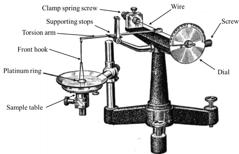
Figure 2-3. A du Noüy ring tensiometer
