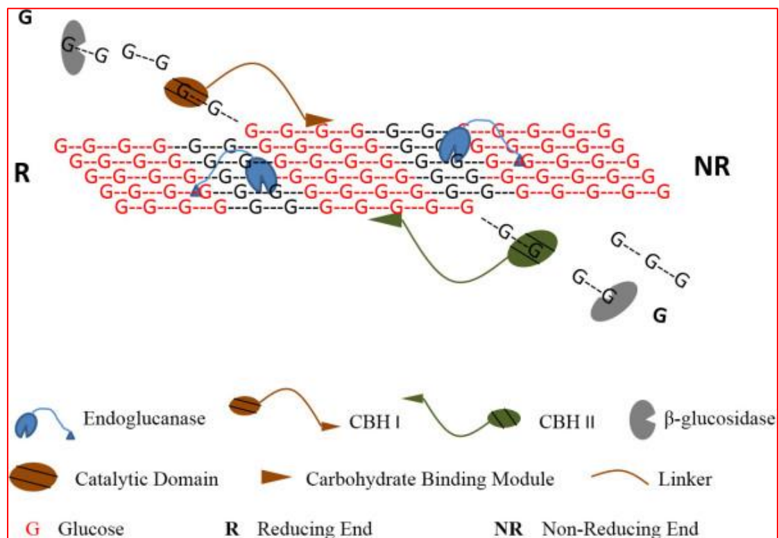
Figure 1-3. Three types of enzyme consisting of cellulase
