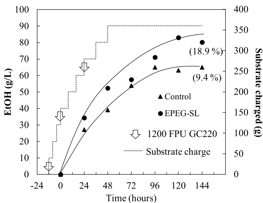
Figure 4-5. Ethanol production with a commercial cellulase (GC220) in the 1.5 L FB-SSF in the presence and absence of 3.0 g/L EPEG-SCL under the optimum condition. Total substrate loading was 360 g and total cellulase charge was 3600 FPU. Substrate
