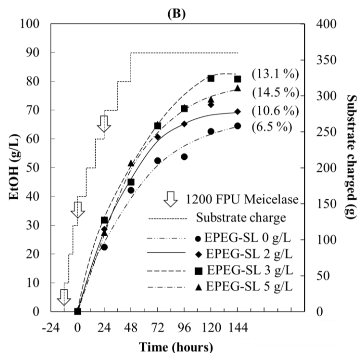
Figure 4-4. Ethanol production with a commercial cellulase (Meicelase) at different loadings of DOPEG-SCL (A) and EPEG-SCL (B) in the 1.5-L scale FB-SSF.
