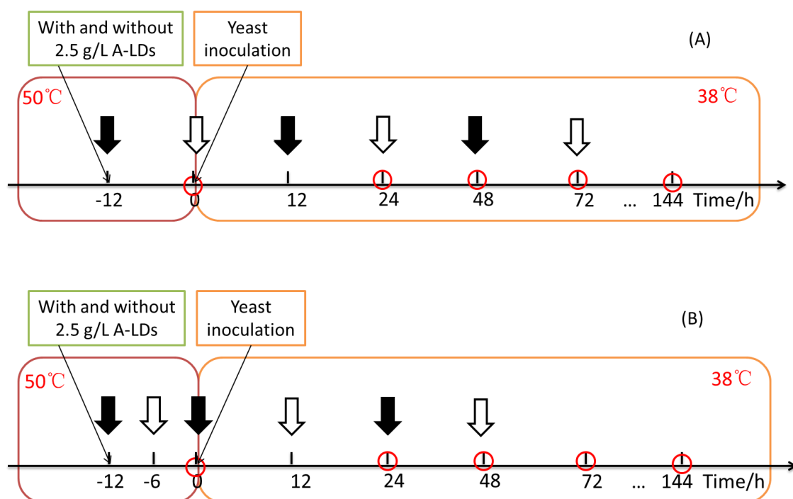
Figure 3-1. Time schedule for reactant charge and sampling during SSF process at a cellulase loading of 5 FPU/g of unbleached cedar soda pulp (A); 6.67 FPU/g and 10 FPU/g (B). (↓, charge of pulp and cellulase; ↘, charge of only pulp; ○, sampling for ethanol determination)
