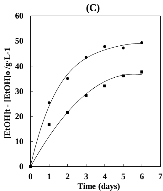
Figure 3-4. Ethanol production in 100 mL scale FB-SSF with GC220 5.0 FPU/g (A); 6.67 FPU/g (B); 10.0 FPU/g (C) of cedar soda pulp in the presence of DOPEG-SCL (●-) and absence of DOPEG-SCL (-■-).
