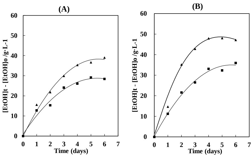
Figure 3-5. Ethanol production in 100 mL scale FB-SSF with GC220 5.0 FPU/g (A); 10.0 FPU/g (B) of cedar soda pulp in the presence of EPEG-SCL (-▲-) and in absence of EPEG-SCL (-■-).
