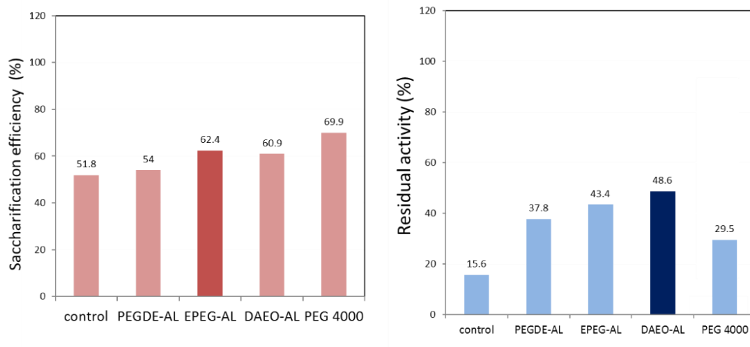
Figure 1-4. Sugar yield and recovery of cellulase activity of unbleached cedar pulp using Meicelase at the initial activity of 10 FPU/g substrate. (PEGDE-AL, EPEG-AL and DAEO-AL is A-LDs made from acetic acid lignin) (Winarni et al., 2013)
