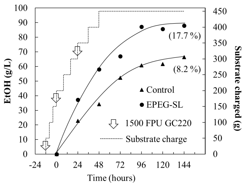
Figure 4-6. Ethanol production with a commercial cellulase (GC220) in the 1.5 L FB-SSF in the presence and absence of 3.0 g/L EPEG-SCL under the optimum condition. Total substrate loading was 450 g and total cellulase charge was 4500 FPU. Substrate charge is shown as a dashed line, and enzyme charge is shown as an arrow. Numbers in the parenthesis indicate the residual enzyme activity (%) after the completion of reaction.
