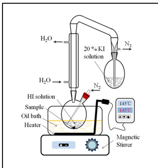
Figure 2-2. Instruments for PEG content measurement
