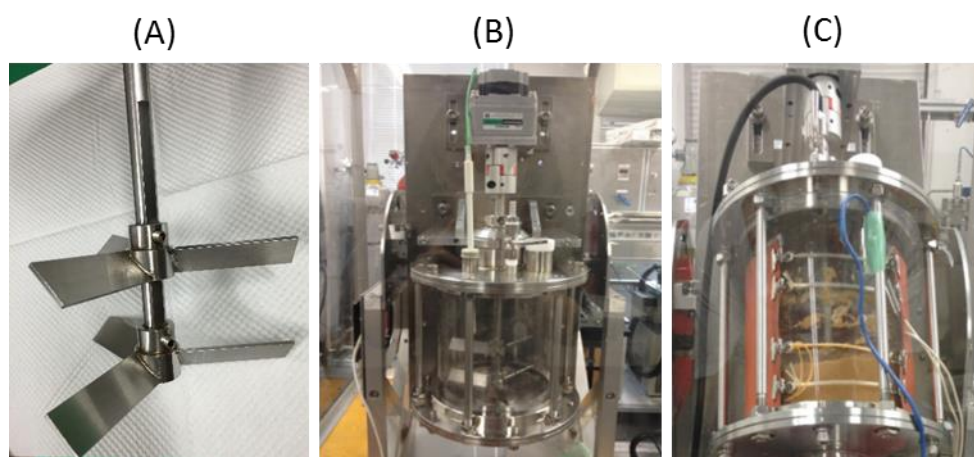
Figure 4-1. Photo of custom-made jar fermenter. (A), impeller inside the tank; (B), front photo of the jar fermenter; (C), operation photo.
