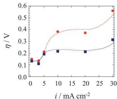
Figure 3. The overpotential, \eta , as a function of the applied current density, i , for Al electrodeposition in EMIC-AlCl 3 ionic liquid at 60°C in 0 T (red ●) and 0.3 T (blue ■) magnetic field.
