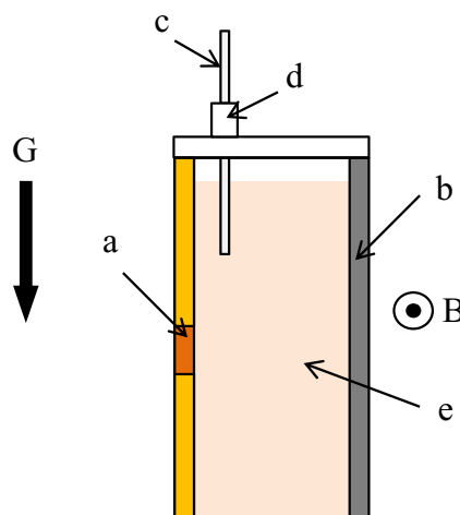
Figure 1. Schematic of the experimental cell showing the cathode (Cu, 25 \text{ mm}^2 ) (a), anode (Al, 350 \text{ mm}^2 ) (b), reference electrode (Al wire, \phi = 0.5 \text{ mm} ) (c), silicon cap (d) and ionic liquid (e). Also shown are the directions of the external magnetic field, B , and the force of gravity, G .
