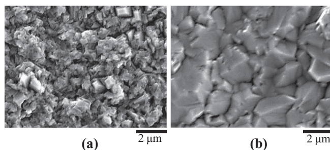
Figure 4. Scanning electron microscope images of Al films electrodeposited galvanostatically for 2 minutes at 30 mA cm -2 in a magnetic field of (a) 0 T and (b) 0.3 T (Film thickness: 10 μm).
