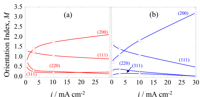
Figure 6. The orientation index, M , as a function of the applied current density, i , for the Al films electrodeposited in (a) 0 and (b) 0.3 T magnetic field, showing the (111) plane (●), (200) plane (■), (220) plane (▲), and (311) plane (◆).
