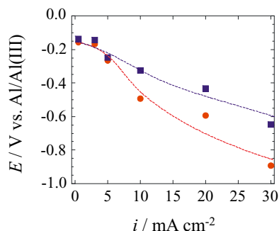
Figure 2. Potential–current plots for Al electrodeposition in EMIC-AlCl 3 ionic liquid at 60°C in a magnetic field of 0 T (red ●) and 0.3 T (blue ■).
