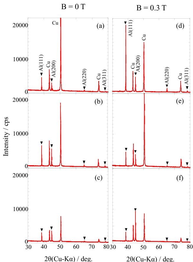
Figure 5. X-ray diffraction spectra of Al films electrodeposited on a Cu substrate at several applied current densities of (a) 5, (b) 10 and (c) 30 mA cm -2 in 0 T magnetic field, and (d) 5, (e) 10 and (f) 30 mA cm -2 in 0.3 T.
