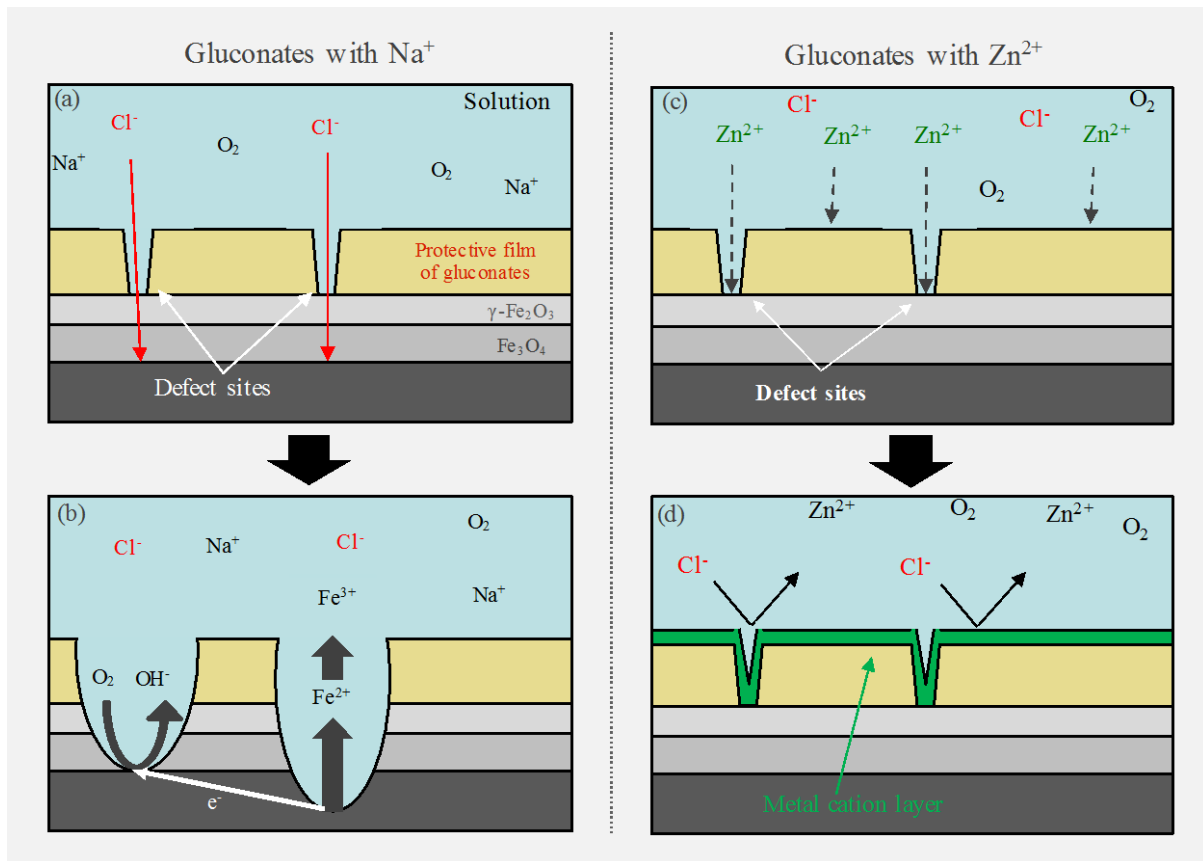
Fig. 9 Schematic images of the process by which a gluconate inhibits corrosion of mild steel in model fresh water containing gluconates with \text{Na}^+ ((a) and (b)) and containing gluconates with \text{Zn}^{2+} ((c) and (d)).
