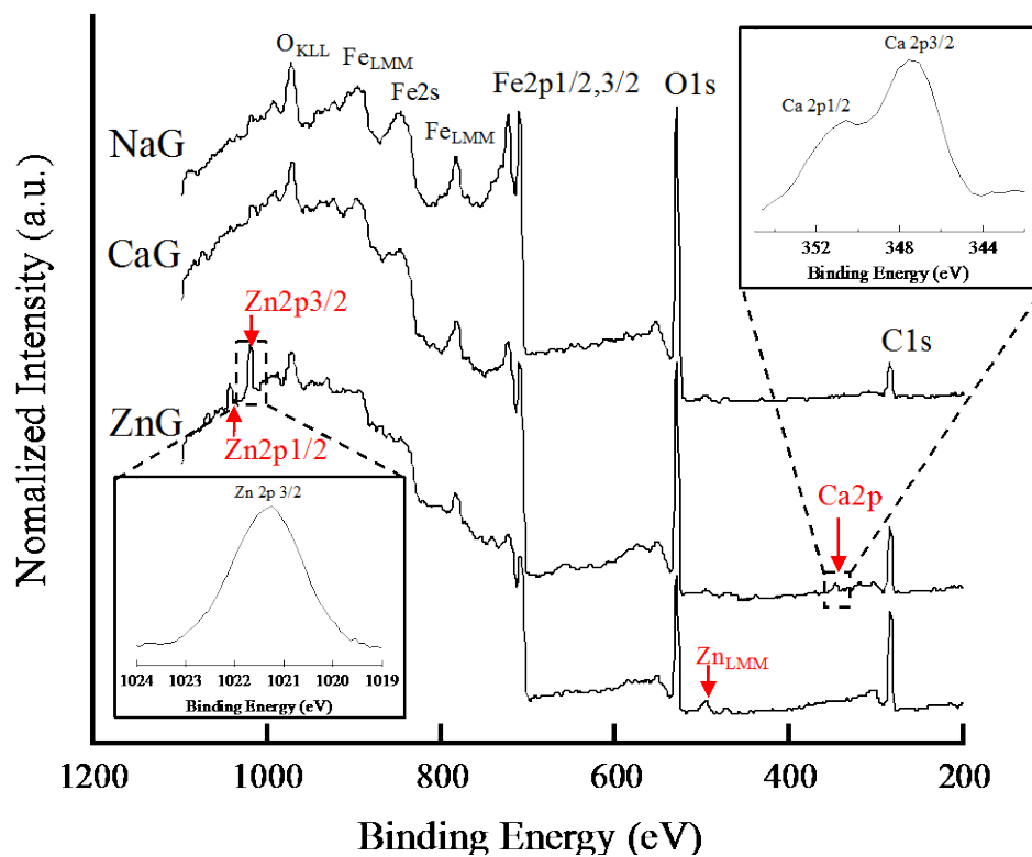
Fig. 3 XPS wide and narrow spectra of metal cations on specimens after immersion for 7 d in model fresh water containing gluconates.
