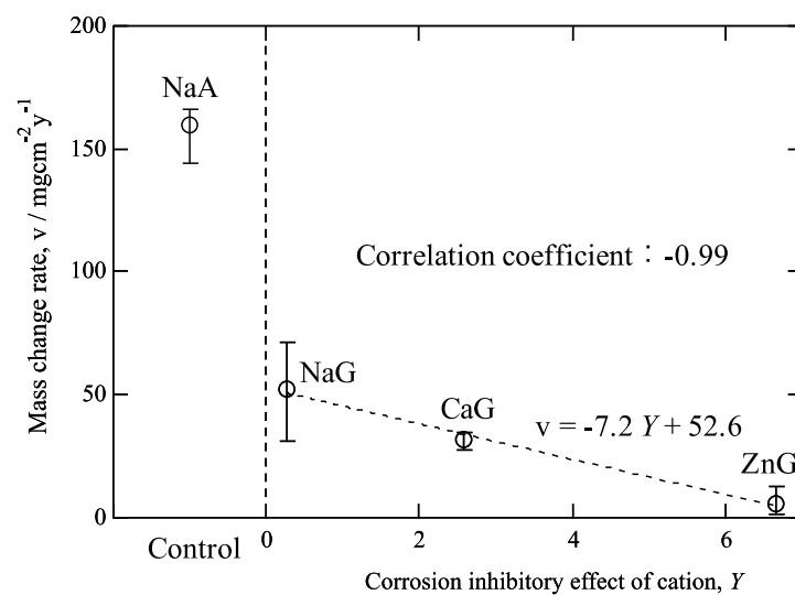
Fig. 6 Mass change rate as a function of Y . The mass change rate of NaA is a control data.
