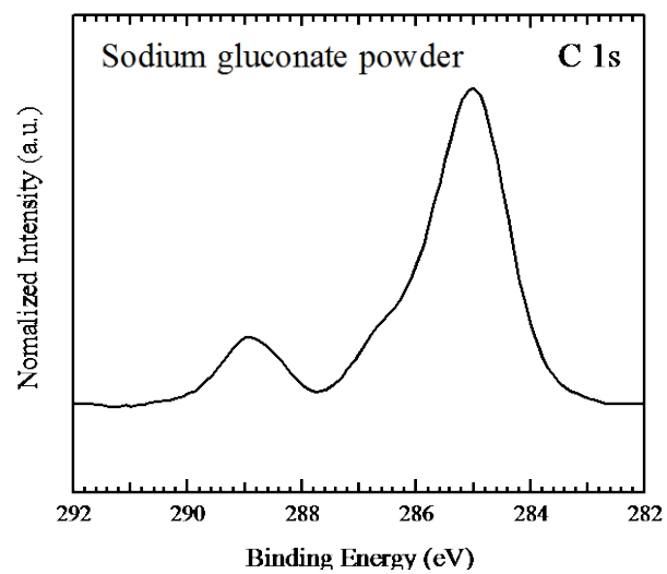
Fig. 5 XPS narrow spectrum of C 1s on sodium gluconate powder.
