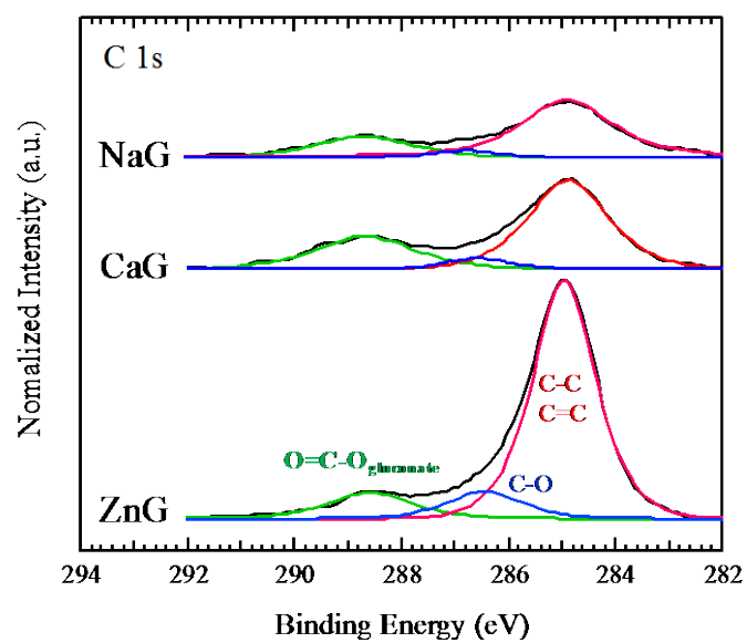
Fig. 4 XPS narrow spectra of C 1s on specimens after immersion for 7 d in model fresh water containing gluconates.
