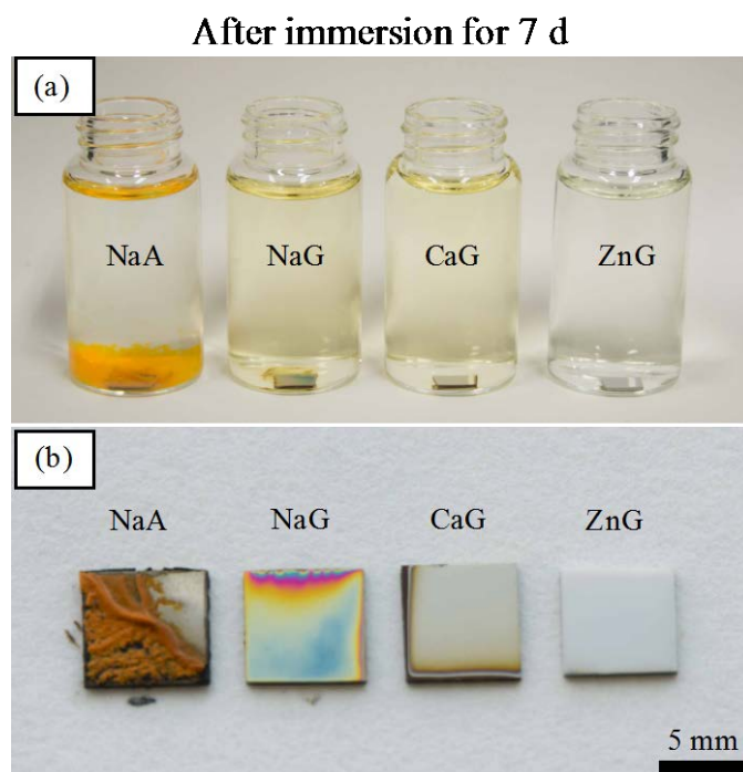
Fig. 1 (a) Appearance of bottled specimens after immersion for 7 d in model fresh water, and (b) surface images of specimens after immersion for 7 d in the solutions.
