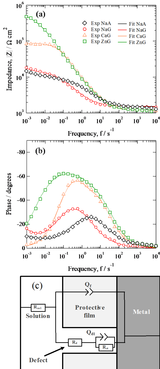
Fig. 7 Bode diagram of (a) Impedance and (b) phase shift after immersion for 7 d in the solutions and fitted lines calculated by an equivalent circuit. (c) Equivalent circuit with a schematic diagram of a mild steel electrode with a protective film having a defect.
