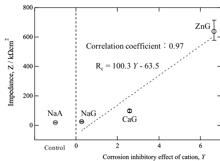
Fig. 8 Corrosion resistance, R_c , as a function of Y . The R_c of NaA is a control data.
