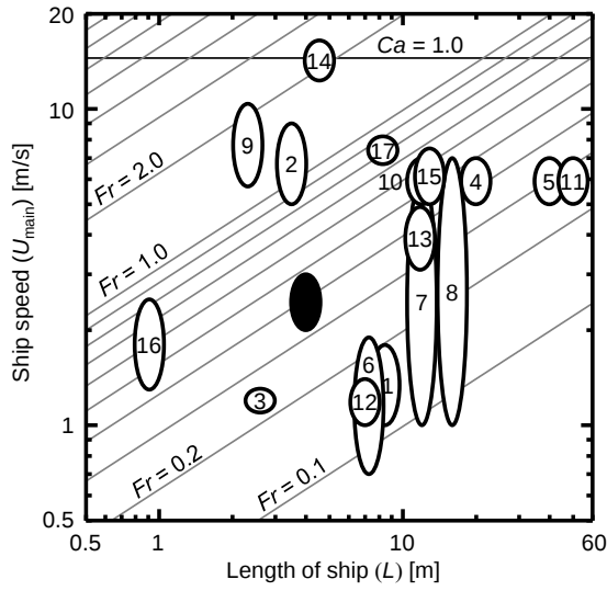
Fig. 5 Ellipse plots of the experimental parameter conditions examined in the past relative to the present experimental condition (closed ellipse); numbers labeling open ellipses correspond to the experimental ships listed in Table 1.
