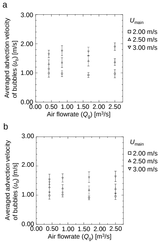
Fig. 11 Averaged advection velocity of bubbles measured at (a) x \approx 2.1 m and (b) 3.3 m, where error bars indicate standard deviations.
