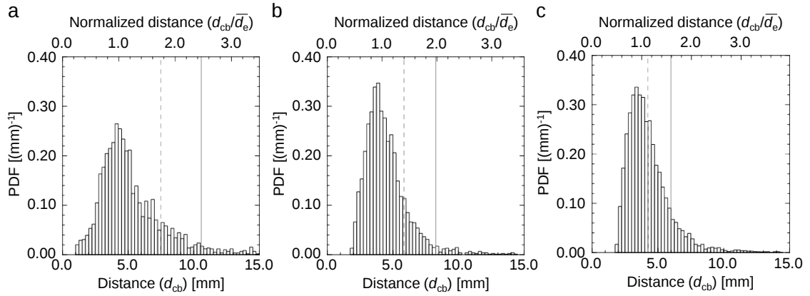
Fig. 15 Probability density distribution of the mutual distance between the closest pair of bubbles for Q_g \approx 0.42 \times 10^{-3} \text{ m}^3/\text{s} at x \approx 3.3 \text{ m} : (a) U_{\text{main}} = 2.00 \text{ m/s} , (b) 2.50 \text{ m/s} and (c) 3.00 \text{ m/s} . Small bubbles, d_e < 1.0 \text{ mm} , are regarded outside the analysis; the vertical solid and dashed lines indicate the distances between bubbles for perfect uniform distribution and random distribution.
