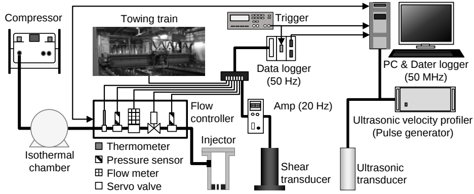
Fig. 2 Schematic diagram of the flow control system synchronized and integrated with multiple measuring devices.
