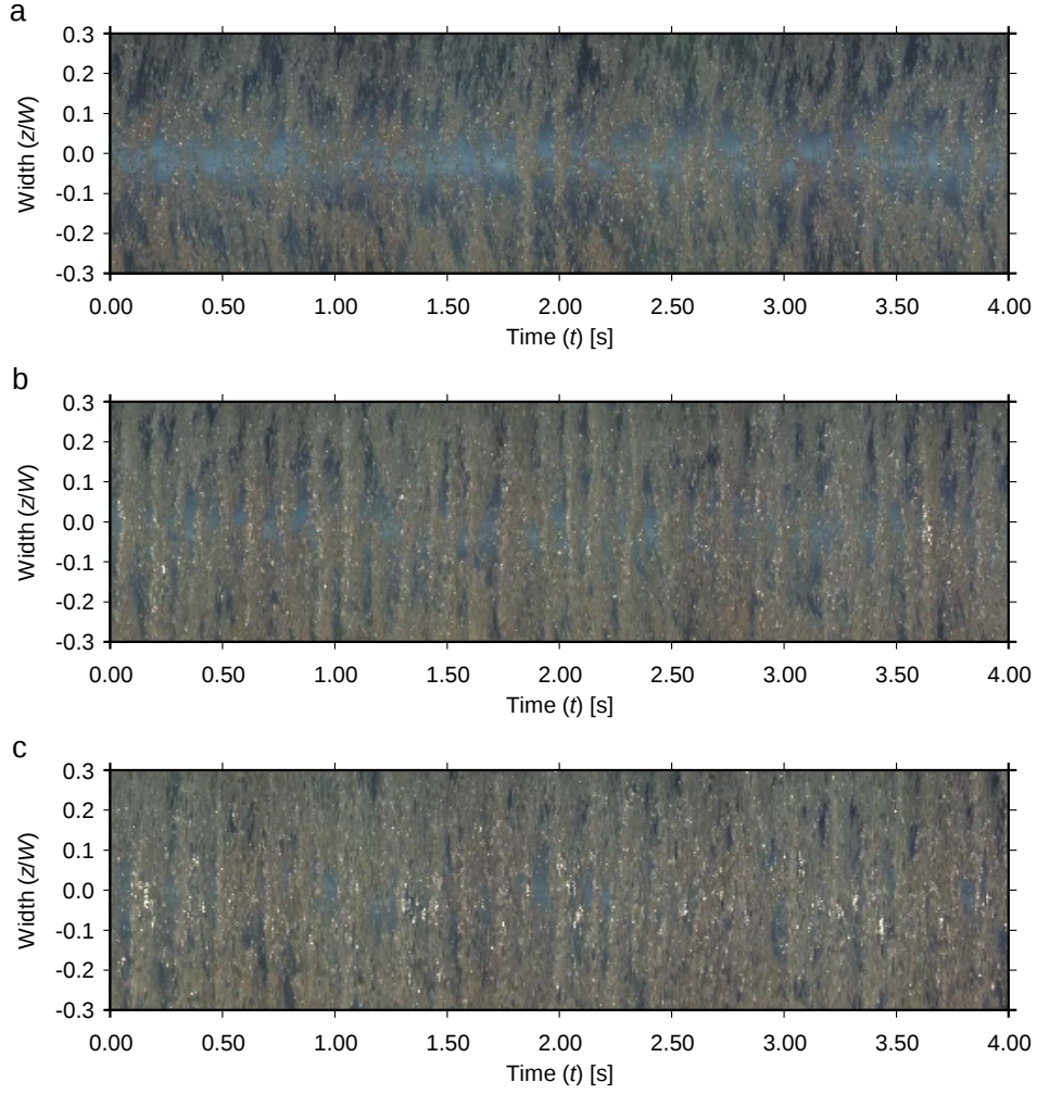
Fig. 13 Time-line scanning images taken at x \approx 3.7 m for U_{\text{main}} = 3.00 m/s; (a) Q_g \approx 0.83 \times 10^{-3} \text{ m}^3/\text{s} , (b) 1.67 \times 10^{-3} \text{ m}^3/\text{s} and (c) 2.50 \times 10^{-3} \text{ m}^3/\text{s} .
