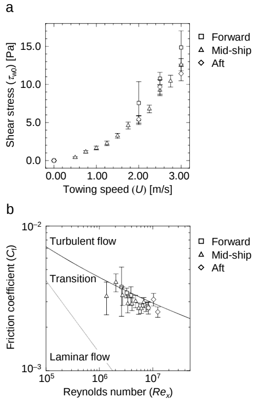
Fig. 6 Frictional drag of the model ship in single-phase flow conditions, where error bars indicate standard deviations of the temporal fluctuation; (a) local wall shear stress as a function of ship speed, and (b) coefficient of friction as a function of Reynolds number; the two curves represent the Blasius friction law for laminar flow and the empirical coefficient of friction for turbulent flow (Schlichting 1979).
