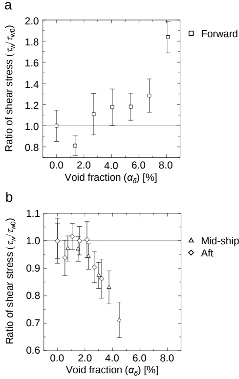
Fig. 7 Wall shear stress modified by bubble injection with respect to void fraction at a ship speed of U_{\text{main}} = 3.00 m/s; (a) forward, and (b) mid-ship and aft, where error bars indicate standard deviations.
