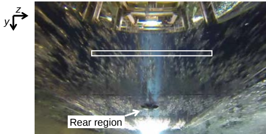
Fig. 12 Snapshot taken by the underwater camera; the framed area is located at x \approx 3.7 m and used to generate time-line scanning images.
