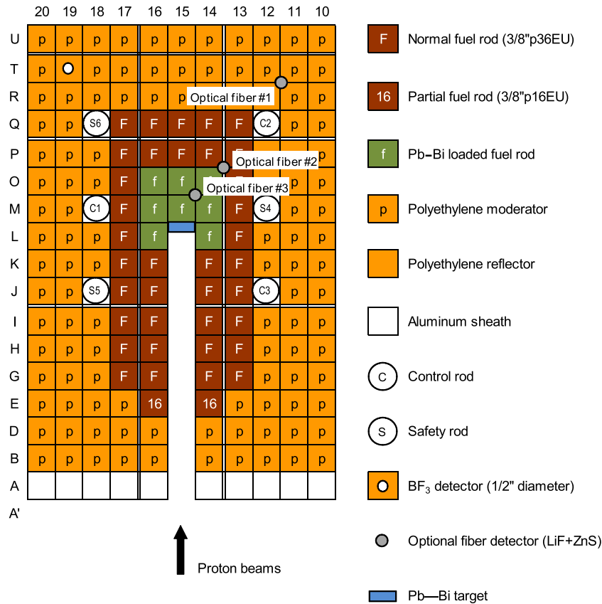
Fig. 4. Top view of ^{235}\text{U} -fueled and Pb-Bi-zoned core configuration in ADS-P experiments [6]. ADS-P, accelerator-driven system with proton; LiF, lithium-fluoride; Pb-Bi, lead-bismuth; ZnS, zinc sulfide.
