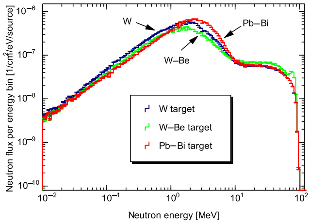
Fig. 3. Comparison between neutron spectra with the use of W, W-Be, and Pb-Bi targets in ADS-P experiments [5]. ADS-P, accelerator-driven system with proton; Pb-Bi, lead-bismuth; W, tungsten; W-Be, tungsten-beryllium.
