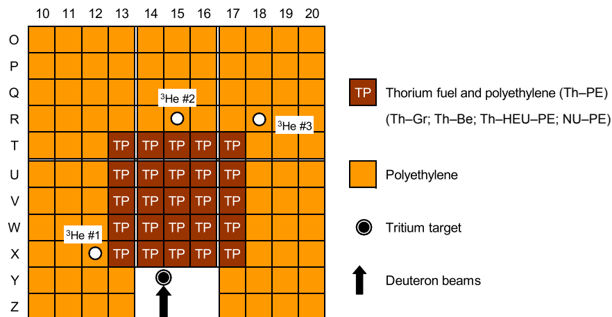
Fig. 5. Top view of ^{232}\text{Th} -loaded core configuration (Th-PE) in ADS-DT experiments [7, 10]. ADS-DT, accelerator-driven system with deuterium and tritium; ^3\text{He} , helium-3; NU-PE, natural uranium and polyethylene; PE, polyethylene; Th-Be, thorium and beryllium; Th-Gr, thorium and graphite; Th-HEU-PE, thorium and highly-enriched uranium.
