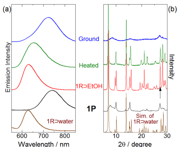
Fig. 4 Changes in the (a) luminescence spectra ( \lambda_{\text{ex}} = 400 nm) and (b) powder X-ray diffraction patterns ( \lambda = 1.5418 Å) of 1R →EtOH (red), 1R →EtOH after heating (green), and 1R →EtOH after heating and grinding (blue). The black lines in both panels show the emission spectrum and PXRD pattern of 1P . The bottom pattern in (b) is the simulated pattern calculated from the crystal structure of 1R →water. The arrow in (b) indicates the position of the (002) reflection.
