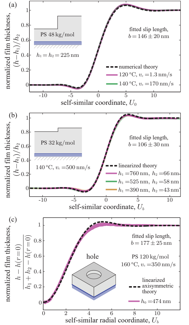
FIG. 2. Capillary leveling is a robust experimental probe to measure slip length. For three different sample geometries, the rescaled self-similar theoretical profiles (dashed lines) fit the experimentally measured ones (solid lines) with one free parameter, the slip length b . Parameters are indicated in legends, and theoretical details are provided in main text. In (c), the position x is replaced by the radial coordinate r .
