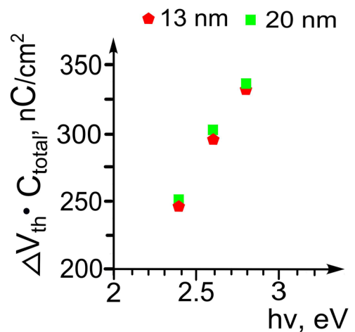
FIG. 8. Experimental dependencies of \Delta V_{th} \cdot C_{total} vs. h\nu for \text{Al}_2\text{O}_3/\text{InAlN}/\text{GaN} structures with d_l = 13 nm (from Ref. 33) and d_l = 20 nm.
