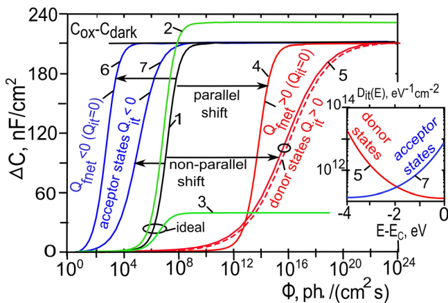
FIG. 5. \Delta C(\Phi) curves calculated according to the model from Sec. IV A, for \text{Al}_2\text{O}_3/\text{AlGaIn}/\text{GaIn} structure under V_G = -4 V, in the case of an ideal \text{Al}_2\text{O}_3/\text{AlGaIn} interface ( Q_{it}=0 , Q_{fnet}=0 ) (curves 1, 2, 3) and non-ideal interfaces with the positive Q_{fnet}=10^{12} q/cm 2 ( Q_{it}=0 ) (curve 4) with donor-like states ( Q_{it}>0 , Q_{fnet}=0 ) (curve 5), with the negative Q_{fnet}=-10^{12} q/cm 2 ( Q_{it}=0 ) (curve 6) and with acceptor-like states ( Q_{it}<0 , Q_{fnet}=0 ) (curve 7). Curves 1, 4–7 calculated for d_I=20 nm and d_B=25 nm, curve 2 for d_I=20 nm and d_B=35 nm, curve 3 for d_I=45 nm and d_B=25 nm. Solid lines correspond to \tau=10^{-7} s and dashed line to \tau=10^{-9} s. In the inset given D_{it}(E) assumed in calculations.
