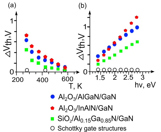
FIG. 7. Experimental dependencies of \Delta V_{th} vs. T under illumination with h\nu = 2 eV (a) and \Delta V_{th} vs. h\nu at RT (full symbols) (b). Dependencies for Schottky gate structures (open circles) given for comparison.
