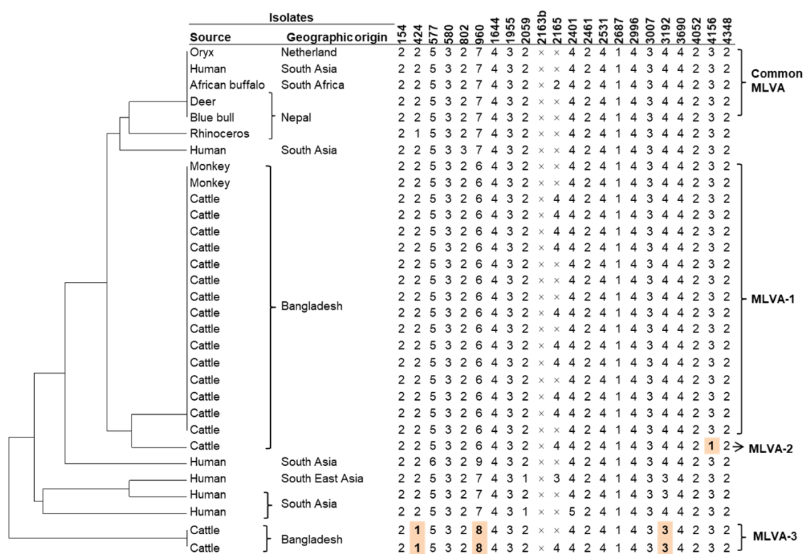
Figure 8. UPGMA dendrogram of M. orygis isolates based on MLVA analysis. The order of 22 MLVA loci are as follows, left to right: 154, 424, 577, 580, 802, 960, 1644, 1955, 2059, 2163b, 2165, 2401, 2461, 2531, 2687, 2996, 3007, 3192, 3690, 4052, 4156 and 4348.
