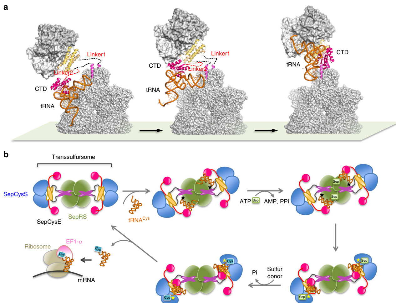
Fig. 5 Proposed mechanism of the tRNA-dependent cysteine biosynthesis by transsulfursome. a tRNA channeling for consecutive reactions of the transsulfursome. Only upper half of the transsulfursome is drawn here. (Left) The first reaction state (SepRS active form). This model was built by superposing the SepCysE(CTD)-tRNA Cys complex (present work) with the SepRS-tRNA complex (PDB:2DU3). The stretching of linker1 and linker2 allows the SepCysE(CTD)-tRNA Cys complex to reach the binding site on SepRS, while anchoring SepCysE(N-helix) to its binding site on SepRS. The anticodon of tRNA Cys is recognized by the site close to the SepCysE(N-helix) binding site. (Middle) The intermediate state. The mischarged Sep-tRNA Cys moves from the first reaction site on SepRS to the second reaction site on SepCysS without being released from bound SepCysE(CTD). Two flexible linkers of SepCysE allow the movement of Sep-tRNA Cys over this long distance. (Right) The second reaction state (SepCysS active form). The discriminator base of U73 and possibly the Sep moiety of Sep-tRNA Cys are recognized by SepCysS, followed by conversion to the canonical Cys-tRNA Cys . The anticodon of tRNA Cys may not be recognized by SepRS in this step. b A schematic drawing of the tRNA-dependent cysteine biosynthesis by transsulfursome. N-helix (purple) and NTD (orange) of SepCysE bridge the SepRS (green) and SepCysS (blue) to form ternary complex (transsulfursome) with a molar ratio of 4:4:4. SepCysE (CTD) (red) shuttles tRNA Cys between two distinct active sites on transsulfursome for sequential reactions catalyzed by SepRS and SepCysS. Each of the two enzymes recognizes tRNA Cys separately in the two steps. The released Cys-tRNA Cys is delivered to ribosome by EF1-α to finally incorporate a cysteine into proteins. Two tRNA substrates are bound to the opposite positions on transsulfursome. The recognition sites of tRNA Cys by SepRS and SepCysS are marked with black and yellow asterisks, respectively
