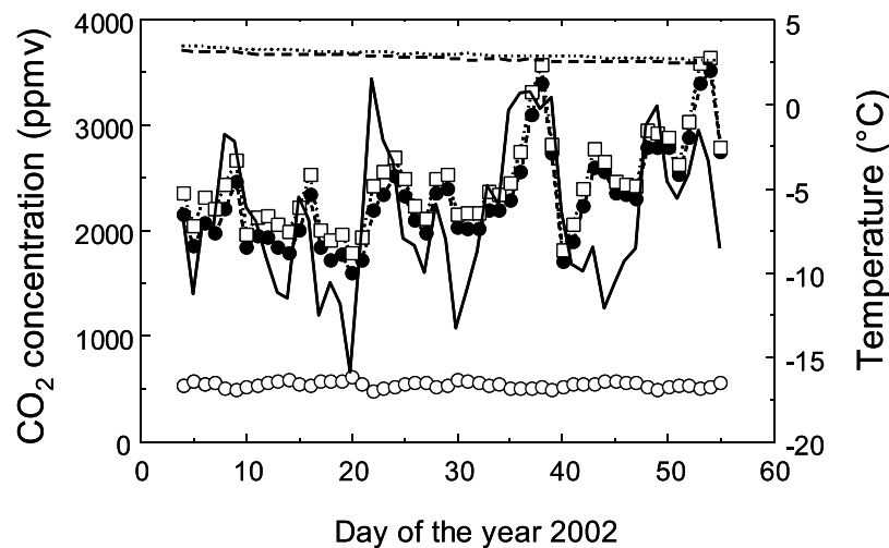
Figure 7. Time series of the daily averages of CO 2 concentration and temperature in the soil and the atmosphere. Open circles indicate the atmospheric CO 2 concentration at 1.5 m height from the ground, and solid circles and open squares indicate the concentration in the soil at 0.05 and 0.15 m deep, respectively. Solid line indicates air temperature at 2 m height, and dashed and dotted lines indicate soil temperatures at the depth of 0.05 and 0.15 m, respectively.
