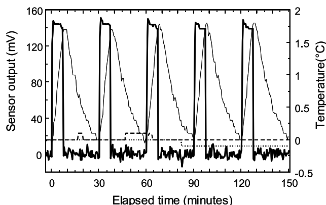
Figure 2. Effect of the power supply to the CO 2 sensor on the surrounding temperatures. Sensor output (thick solid line), sensor body temperature (thin solid line), sensor head temperature (dashed line), and snow temperature near the sensor head (dotted line).
