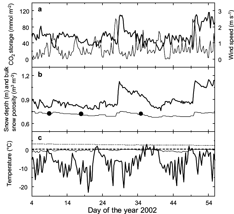
Figure 5. Relationship between CO 2 storage in snowpack and meteorology in midwinter. (a) Six-hour averages of CO 2 storage in snowpack (thick line) and wind speed at height of 2 m (thin line). (b) Observed snow depth (thick line) and observed (circles) and estimated (thin line) bulk snow porosity. (c) Six-hour averages of temperatures at heights of 1.5 m (thick solid line), 0.8 m (thin solid line), and 0.1 m (thick dashed line), and depth of 0.05 m in soil (thin dashed line). Sensors at heights of 0.8 and 0.1 m were in snowpack.
