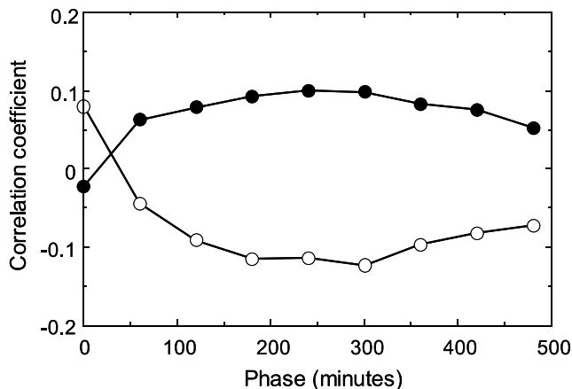
Figure 8. Change in the correlation coefficients between the CO 2 storage-change efflux and the wind speed (open circles) and between net ecosystem exchange and the wind speed (solid circles) with the change in the time lag. Thirty-minute-interval values ( n = 2048 ) were used for the analysis.
