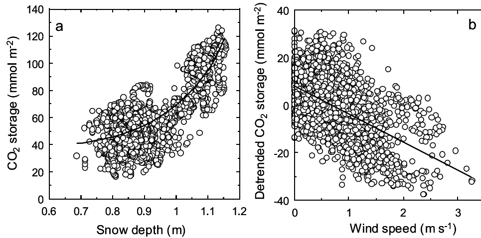
Figure 6. Relations of CO 2 storage (or the detrended value) to (a) snow depth and (b) wind speed. The regression lines in Figures 6a and 6b are Y = 34 + 0.14 \exp(5.5 X) , r^2 = 0.63 , n = 2496 and Y = -11.9 X + 7.8 , r^2 = 0.28 , n = 2496 , respectively. See text for the trend removing.
