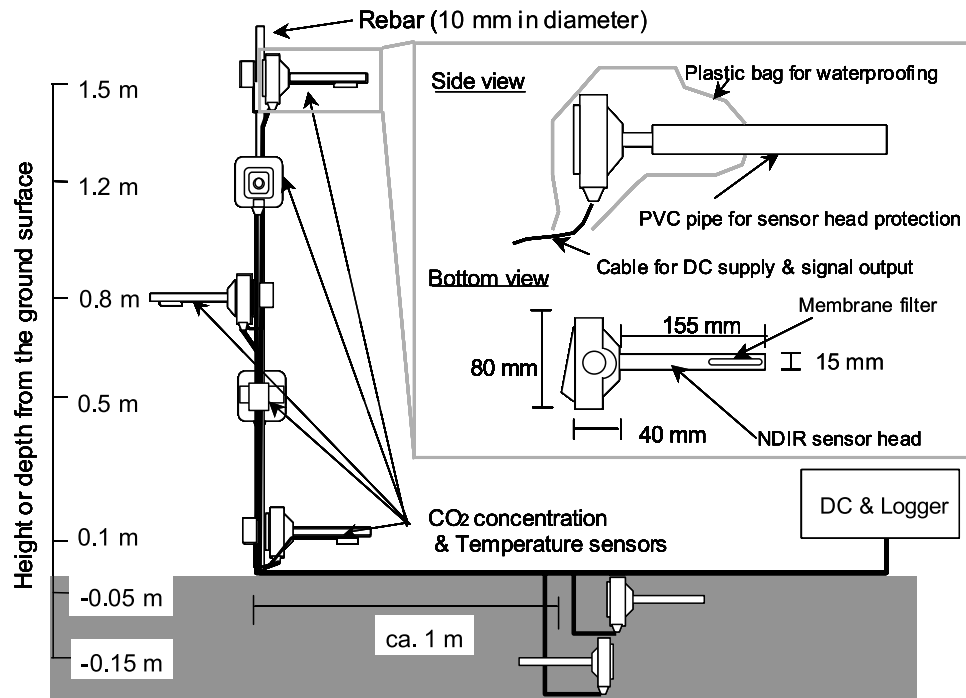
Figure 1. Schematic drawing of the observation system.
