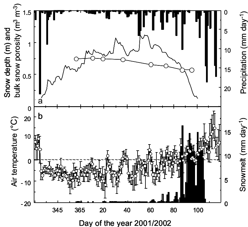
Figure 3. Seasonal changes of snowpack and microclimates. (a) Snow depth (solid line), bulk snow porosity (circles), and precipitation (bars). (b) Daily average air temperature at 30 m height (circles) and snowmelt (bars). Vertical bars across the circles represent maximum and minimum air temperatures for each day.
