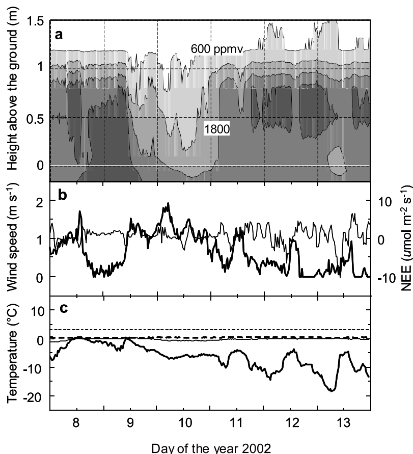
Figure 4. Time series of CO 2 concentrations under snow surface in relation to meteorological data. (a) CO 2 concentration profile. Concentrations were measured at five heights and two depths from the ground surface, and interpolated linearly. Sensors at heights of 0.8, 0.5, and 0.1 m were in snowpack. (b) Wind speed at 2 m height (thick line) and 1.5-hour running averages of net ecosystem exchange (NEE; thin line). (c) Temperatures at heights of 1.5 m (thick solid line), 0.8 m (thin solid line), and 0.1 m (thick dashed line), and at depth of 0.05 m in soil (thin dashed line). Sensors at heights of 0.8 and 0.1 m were in snowpack.
