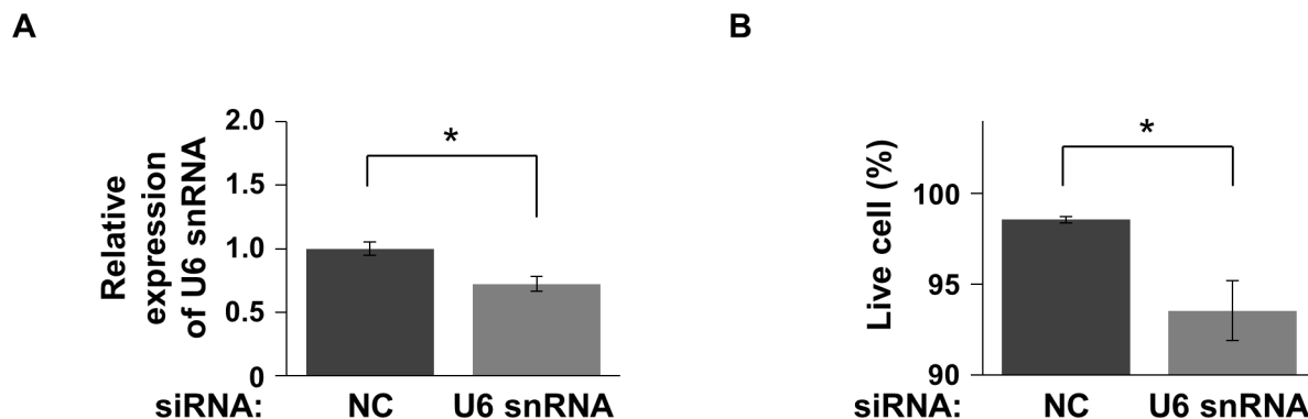
Fig 3. Viability of U6 snRNA-depleted cells. (A) Quantification of U6 snRNA expression at 72 h after transfection of U6-siRNA and NC-siRNA. The expression level of 18S rRNA was used as an internal control (mean \pm SEM, n = 3 ). Significance was tested by Student's t test: *p < 0.05 . (B) The proportion of live cells at 72 h after transfection of U6-siRNA and NC-siRNA (mean \pm SEM; n = 3 ). Significance was tested by Student's t test: *p < 0.05 .
