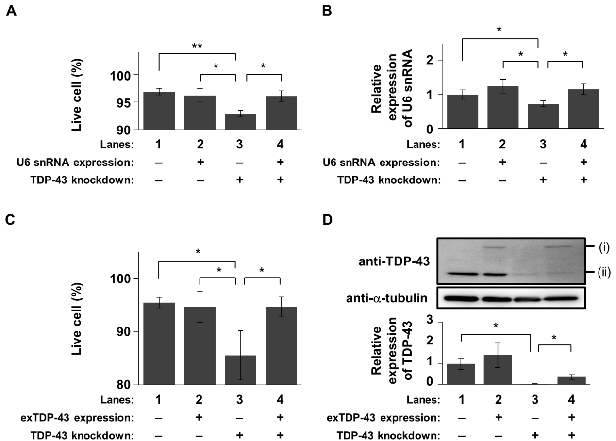
Fig 4. Amelioration of cell death by transient expression of U6 snRNA in TDP-43-knocked down cells. Significance indicated in the graph was tested by Student's t test: * p < 0.05 and ** p < 0.01 . (A) The proportion of live cells at 120 h after transfection of T43-siRNA or NC-siRNA among U6 snRNA-expressing or non-expressing cells (mean \pm SEM; n = 4 ). (B) Quantification of expression of U6 snRNA using qPCR at 72 h after transfection of U6 snRNA expression plasmid DNA or empty vector (mean \pm SEM; n = 4 ). (C) The proportion of live cells at 120 h after transfection of T43-siRNA or NC-siRNA among TDP-43-expressing or control cells (mean \pm SEM; n = 4 ). (D) Protein abundance of TDP-43 and \alpha -tubulin during transient expression of T43-GFP for 76 h. Top: Western blotting using an anti-TDP-43 or anti- \alpha -tubulin antibody. Bands (i) and (ii) indicate T43-GFP and endogenous TDP-43, respectively. Bottom: Quantification of relative expression of TDP-43 (mean \pm SEM; n = 4 ).
