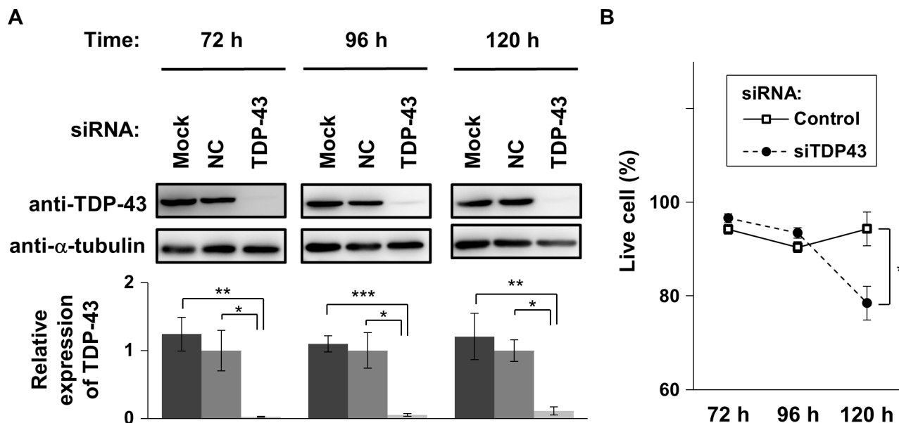
Fig 1. Time course of cell death during TDP-43 depletion. (A) Western blot analysis of endogenous protein expression of TDP-43 and \alpha -tubulin during siRNA-mediated TDP-43 knockdown. Time after transfection of T43-siRNA, NC-siRNA (NC), or no siRNA and transfection reagents (Mock) is indicated (72, 96, and 120 h). \alpha -tubulin was used to normalize band intensities of TDP-43. Bars in bottom graphs indicate the normalized amount of endogenous TDP-43 (mean \pm SEM; n = 3 ). Significance between indicated pairs was tested by Student's t test: * p < 0.05 , ** p < 0.01 , and *** p < 0.001 . (B) The proportion of live cells at 72, 96, and 120 h after transfection of T43-siRNA and NC-siRNA as a negative control (circle and square, respectively; mean \pm SEM; n = 3 ). Significance between T43-siRNA- and NC-siRNA-transfected cells was tested by Student's t test: * p < 0.05 .
