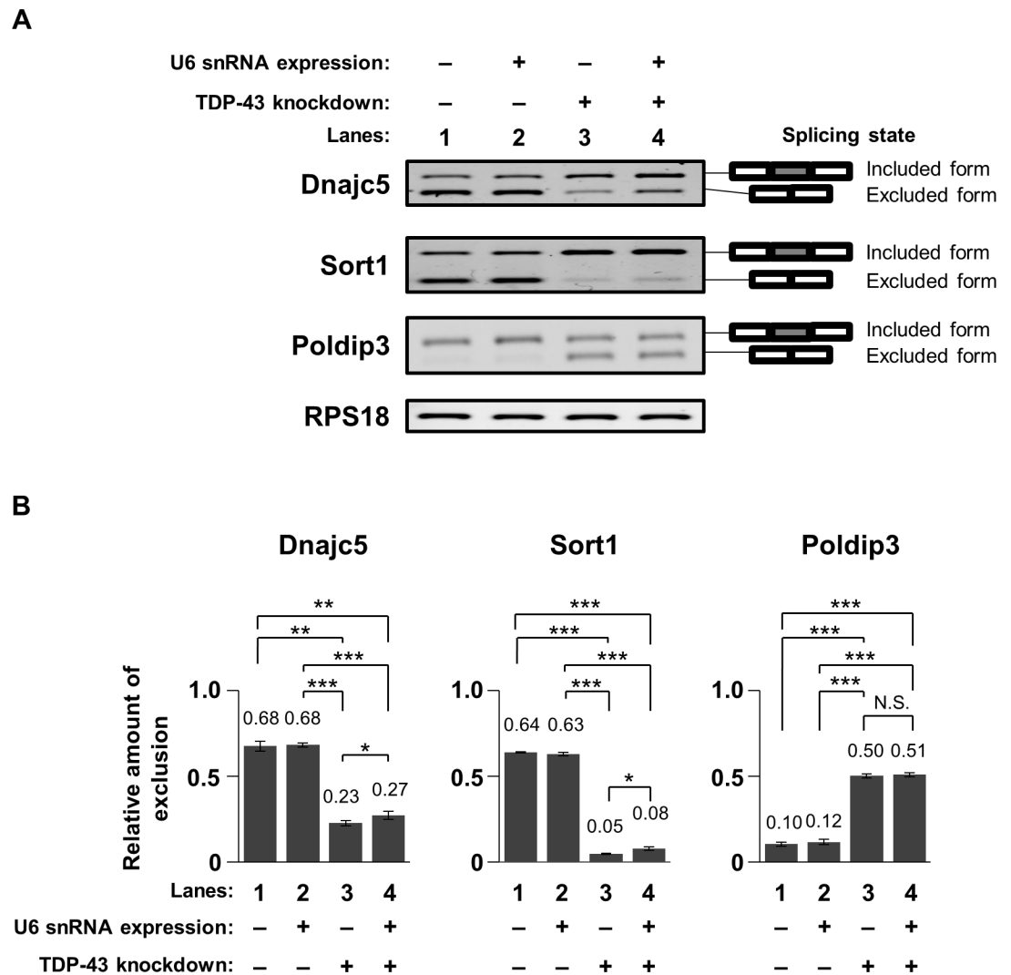
Fig 5. Change in the exon-exclusion state of transcripts during expression of U6 snRNA in TDP-43-knocked down cells. (A) Images of migrated bands of spliced forms of Dnajc5, Sort1, and Poldip3 transcripts. RPS18 was used as an internal loading control. Spliced forms of transcripts were distinguished using splicing-dependent pairs of PCR primers. (B) Relative amounts of the exon-excluded forms of Dnajc5, Sort1, and Poldip3 transcripts (mean ± SEM; n = 5). Significance was tested by Student's t test: * p < 0.05, ** p < 0.01, and *** p < 0.001. Numbers in each bar show mean values.
