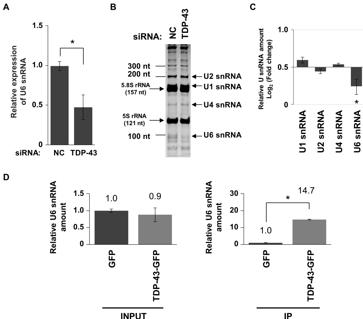
Fig 2. Downregulation of U6 snRNA in TDP-43-knocked down Neuro2A cells. (A–C) Quantification of the expression change of small RNAs during TDP-43 knockdown. Significance was tested by Student's t test: * p < 0.05. (A) Relative expression of U6 snRNA in T43-siRNA-transfected cells compared with that in NC-siRNA-transfected cells. The expression level of 18S rRNA was used as an internal control (mean ± SEM, n = 3). (B) Gel image of Urea-PAGE. Left bar indicates molecular size in nucleotides (nt) of marker. The two dominant bands correspond to 5.8S and 5S ribosomal RNA (rRNA). (C) Relative amount of U1, U2, U4, and U6 snRNAs in T43-siRNA-transfected cells compared with that in NC-siRNA-transfected cells (mean ± SEM, n = 3). (D) Quantification of the binding of U6 snRNA to TDP-43 by CLIP. The amount of U6 snRNA in the sample containing TDP-43-GFP was normalized against that in the sample containing GFP as a negative control in each input cell lysate (INPUT) or immunoprecipitated mixture (IP) (mean ± SEM; n = 3). Significance indicated in the graph was tested by Student's t test: * p < 0.05.
