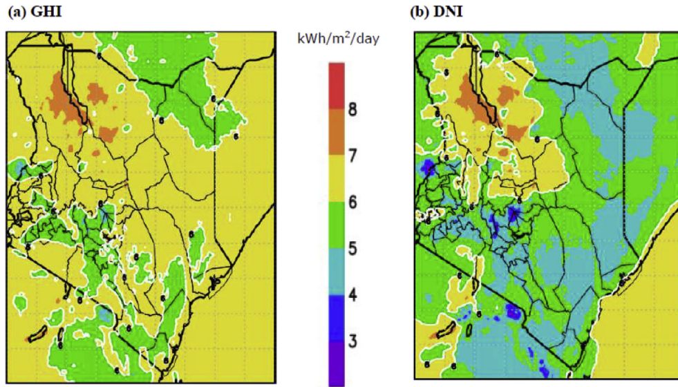
Fig. 3. Spatial distribution of the annual mean (a) GHI and (b) DNI averaged over 19 years (1995–2013).
