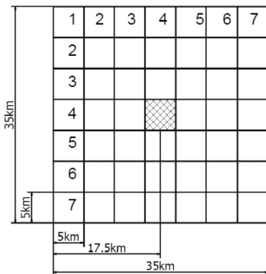
Fig. 7. Illustration of the spatial variability grid arrangement into 7 \times 7 grid matrix (central grid surrounded by 48 cells).
