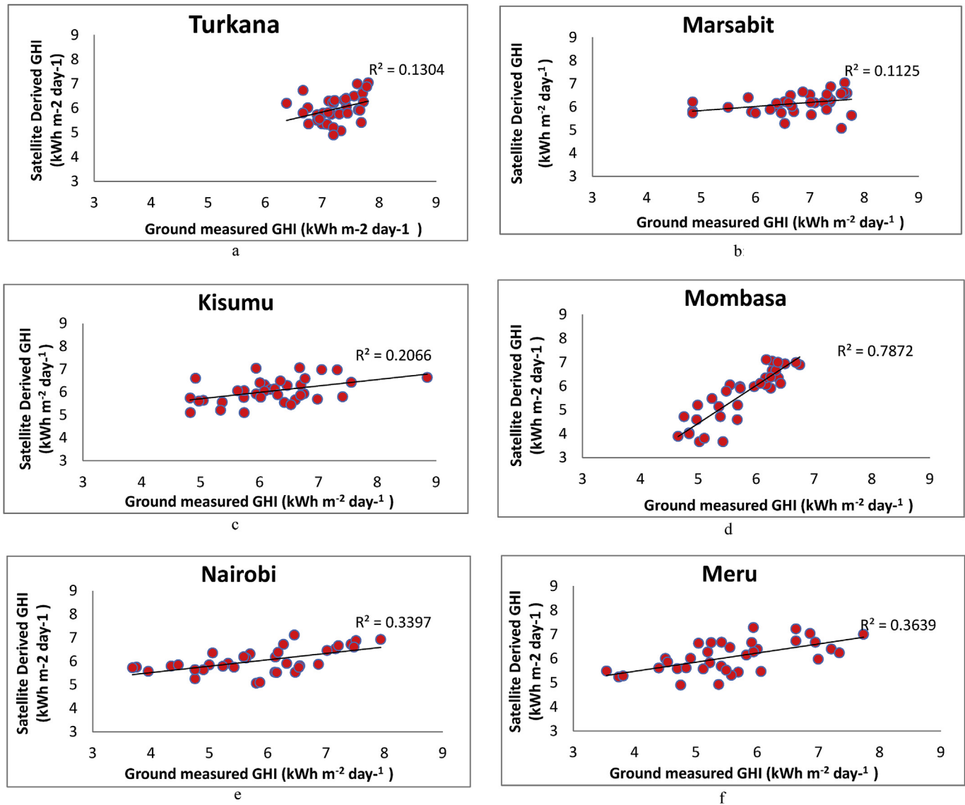
Fig. 2. a: Scatter plot of the ground measured and satellite derived monthly mean GHI during 2010–2013 for Turkana station. b: Same as 2a above but for Marsabit station. c: Same as 2a above but for Kisumu station. d: Same as 2a but for Mombasa station. e: Same as 2a but for Nairobi station. f: Same as 2a but for Meru station.
