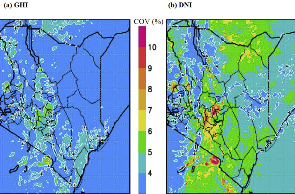
Fig. 6. Spatial distributions of COV_{time} for (a) GHI and (b) DNI.
