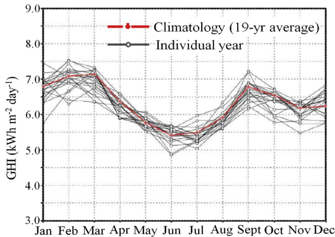
Fig. 4. Seasonal variation of GHI based on 19 years (1995–2013) satellite derived radiation data. Red line and black lines indicate climatology and each individual year, respectively. (For interpretation of the references to colour in this figure legend, the reader is referred to the web version of this article.)
