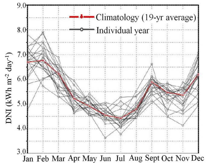
Fig. 5. Same as Fig. 4 but for DNI.
