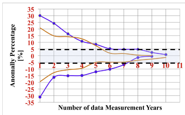
Fig. 9. A relationship between annual solar radiation anomaly with respect to 1995–2013 and the number of measurement years.
