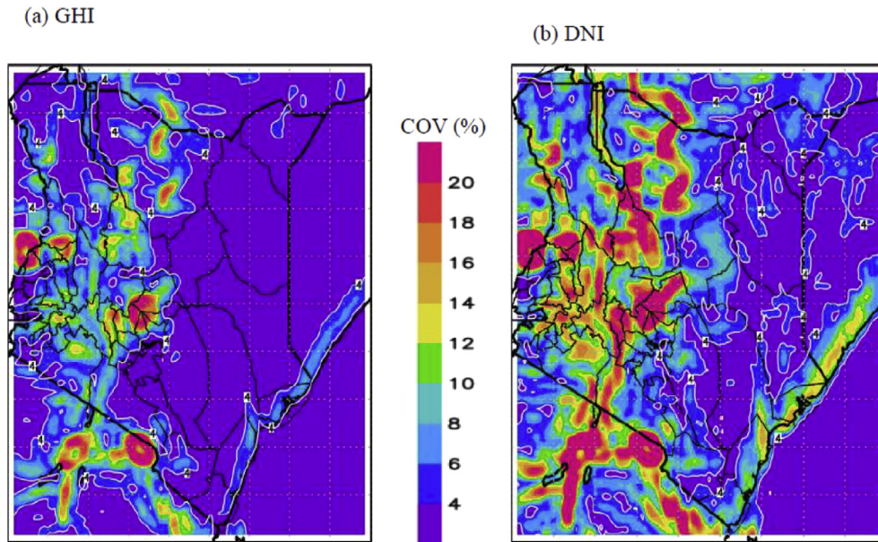
Fig. 8. Spatial distributions of COV_{space} for (a) GHI and (b) DNI.
