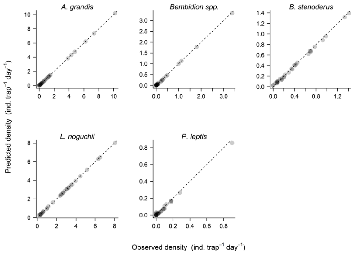
Figure S1 Comparison of predicted and observed density of ground beetles. The broken lines denote a 1:1 relationship.
