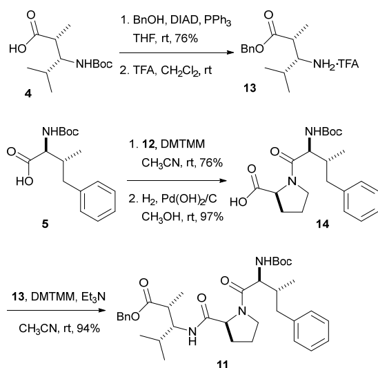
Scheme 2. Synthesis of southern segment 11 .
