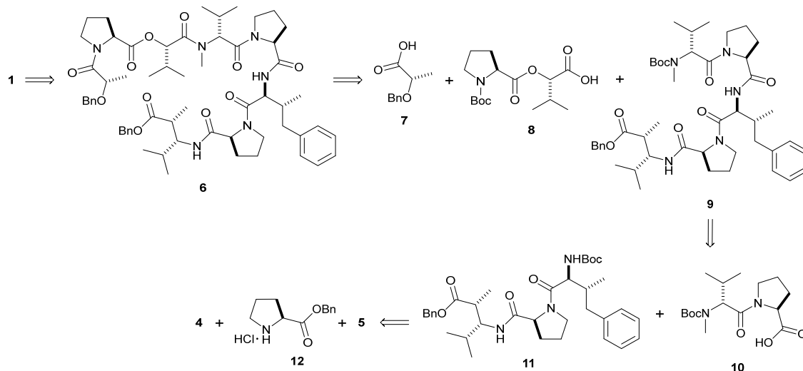
Scheme 1. Retrosynthetic analysis of dolastatin 16 ( 1 ).
