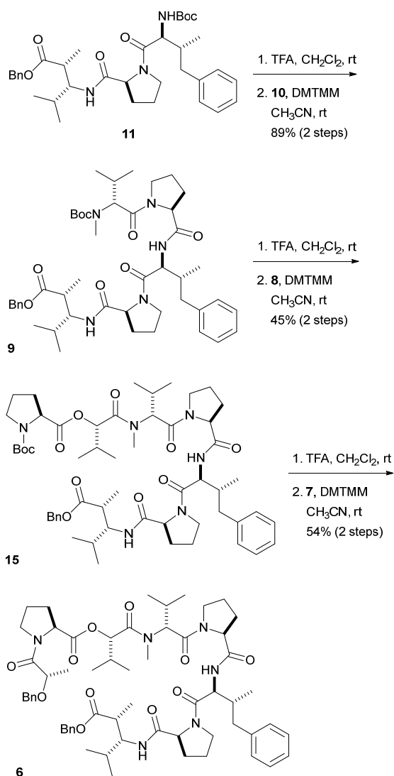
Scheme 3. Synthesis of 6 .
