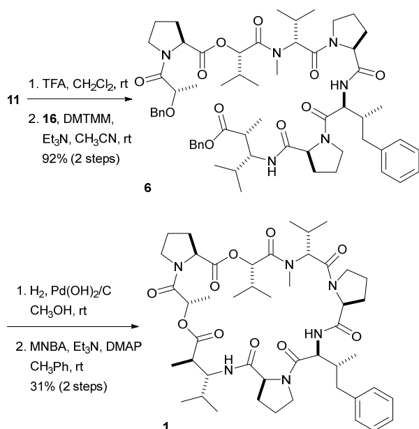
Scheme 7. Total synthesis of dolastatin 16 ( 1 ).
