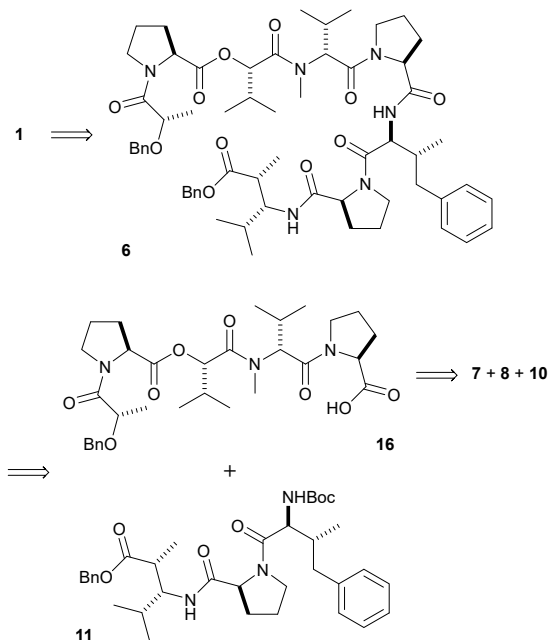
Scheme 4. Improved retrosynthetic analysis of dolastatin 16 ( 1 ).
