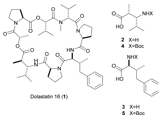
Figure 1. Structure of dolastatin 16 ( 1 ) and the unusual amino acids 2 and 3 .
