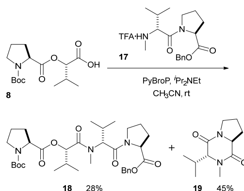
Scheme 5. Diketopiperazine formation.
