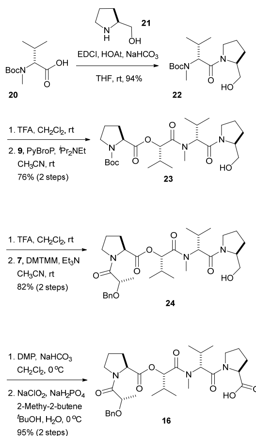
Scheme 6. Synthesis of northern segment 16 .
