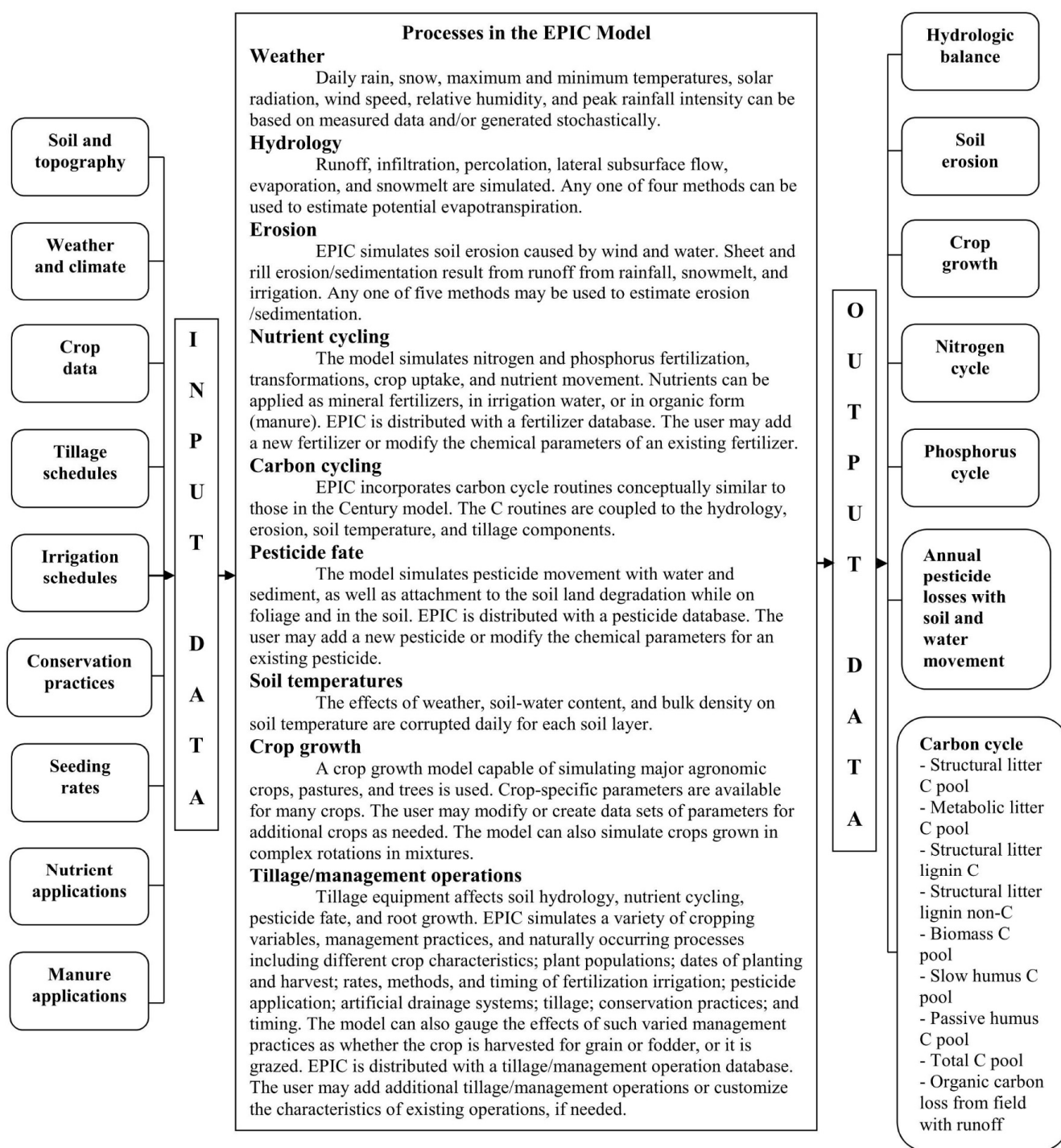
Figure 2-1 General schematic of the key processing steps required of the i-EPIC model
