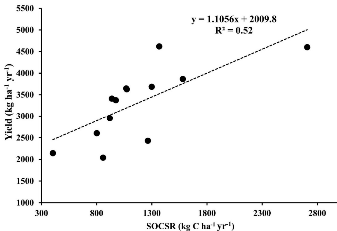
Figure 4-2 Relationship between rice yield and SOCSR for all sites
