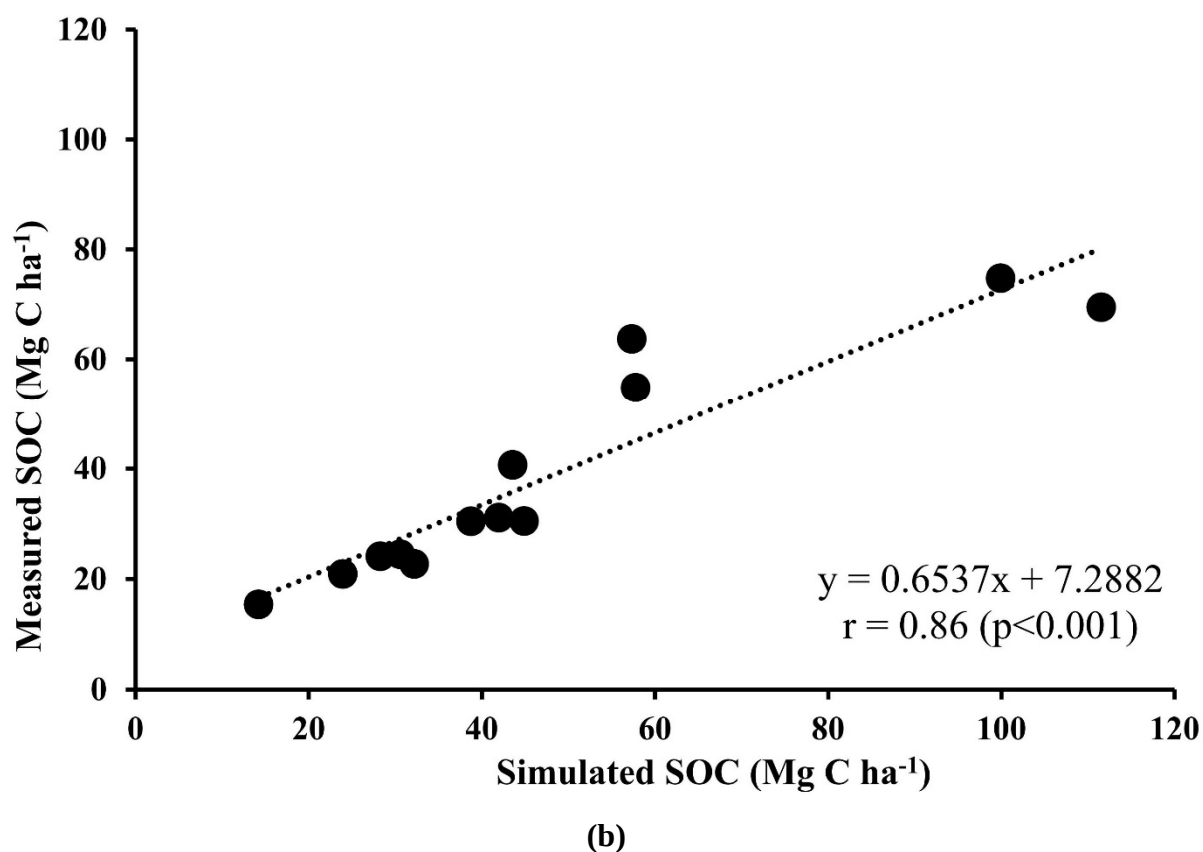
Figure 5-4 Result of calibration of the EPIC model for simulations of (a) rice yield and (b) SOC
