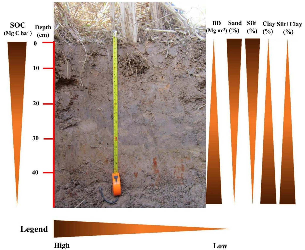
Figure 3-3 The distribution of soil physical properties in the soil profile. The example soil profile is from site R14. BD = Bulk density (Mg m -3 )
