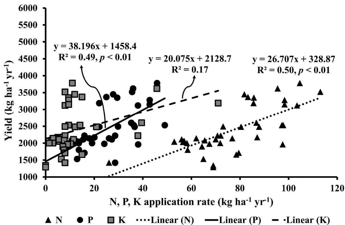
Figure 3-6 Relationship between rice yield and N, P, and K application rates: (a) irrigated areas; (b) rain-fed areas
