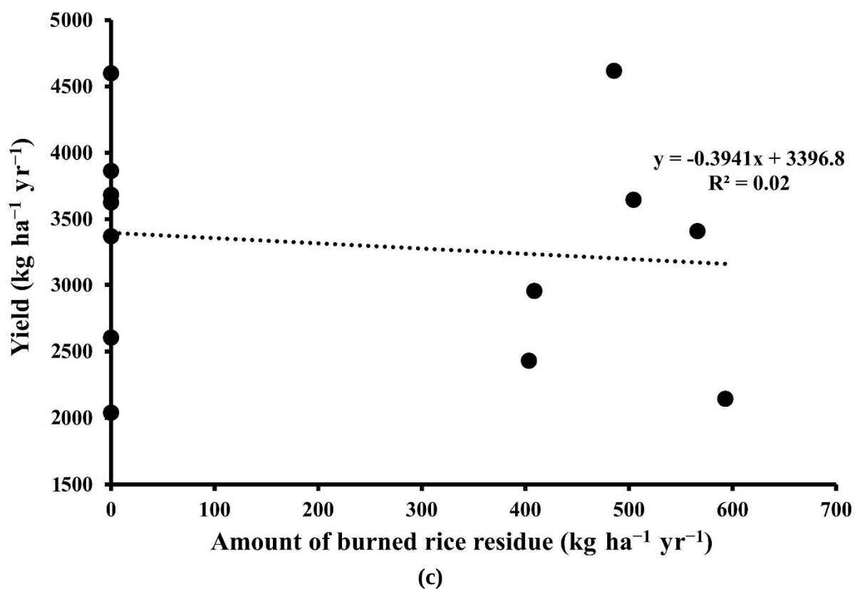
Figure 4-3 Relationship between pertinent practices and rice yield: (a) manure application, (b) fertilizer application, and (c) amount of burned rice residue
