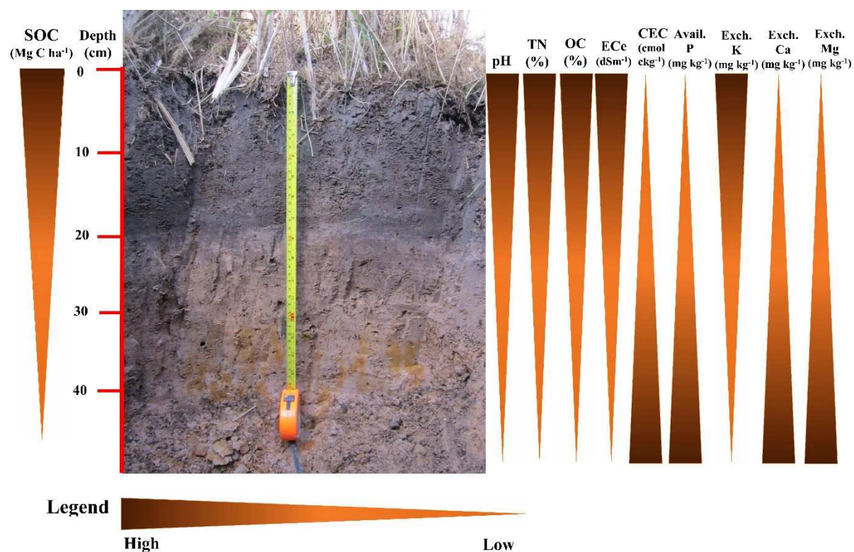
Figure 3-4 Distribution of soil chemical properties in the soil profile. The example soil profile is from site I2. TN = Total nitrogen (%), OC = Organic carbon (%), ECe = Electrical conductivity (dSm -1 ), CEC = Cation exchange capacity (cmol ckg -1 ), Avail. P = Available phosphorous (mg kg -1 ), Exch. K = Exchangeable potassium (mg kg -1 ), Exch. Ca = Exchangeable calcium (mg kg -1 ), Exch. Mg = Exchangeable magnesium (mg kg -1 )
