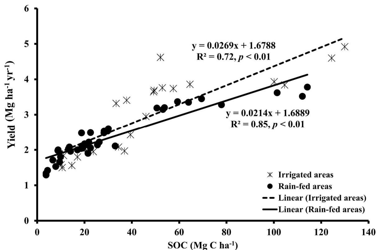
Figure 3-5 Relationship between rice yield and SOC at all sites. The dashed line and solid line were fitted by simple linear regression for irrigated and rain-fed areas, respectively
