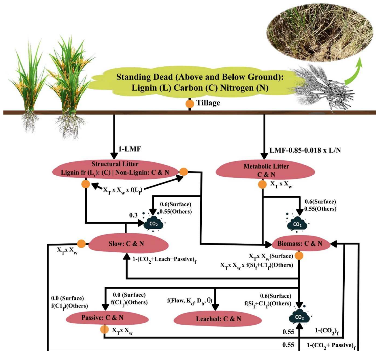
Figure 5-2 Carbon flows in the EPIC model. X_w and X_T refer to moisture and temperature controls on soil biological processes; LMF = fraction of the litter that is metabolic ( \text{kg kg}^{-1} );
