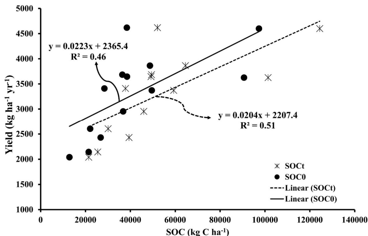
Figure 4-1 Relationship between rice yield and SOC t and SOC 0 for all sites
