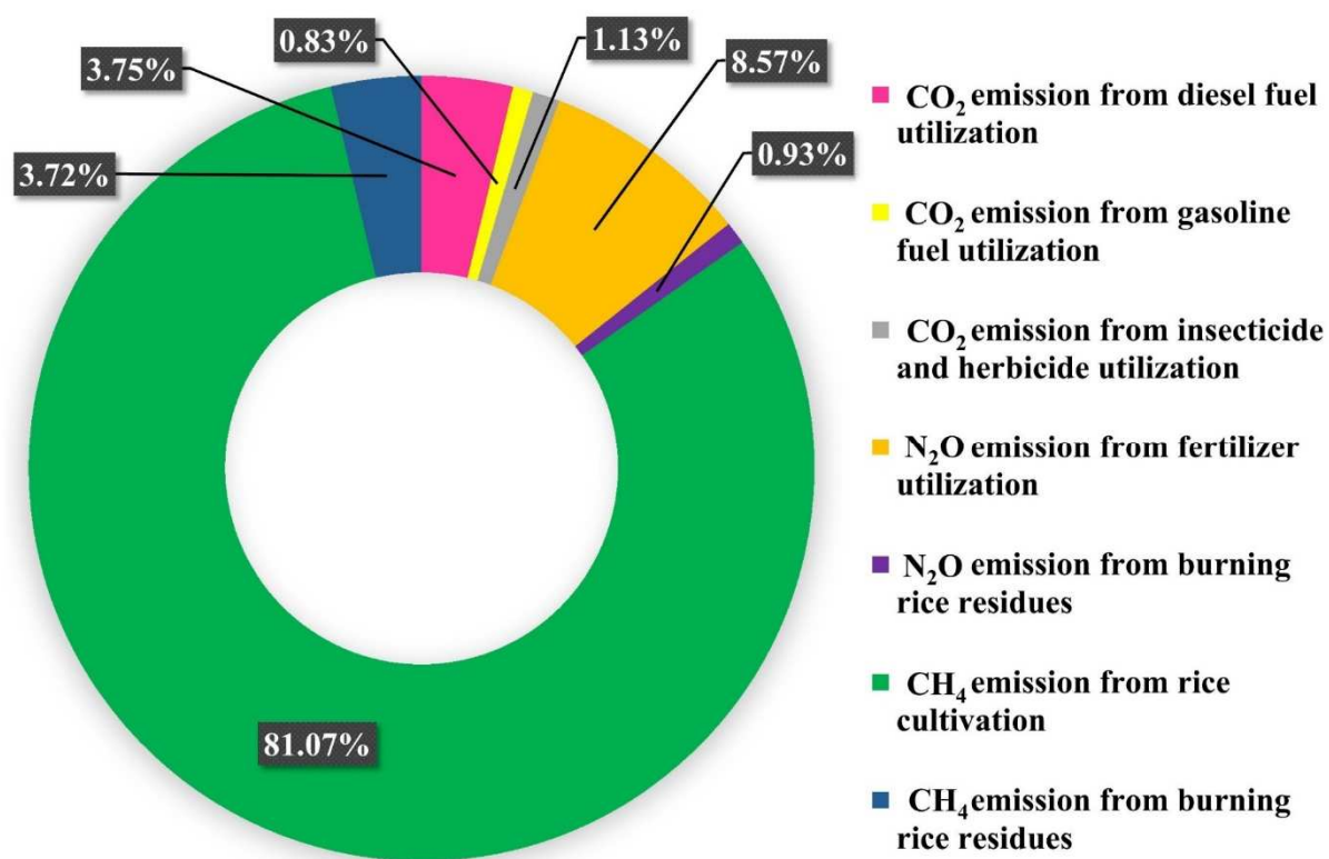
Figure 4-4 The contribution of GHG emission sources in each activity.
