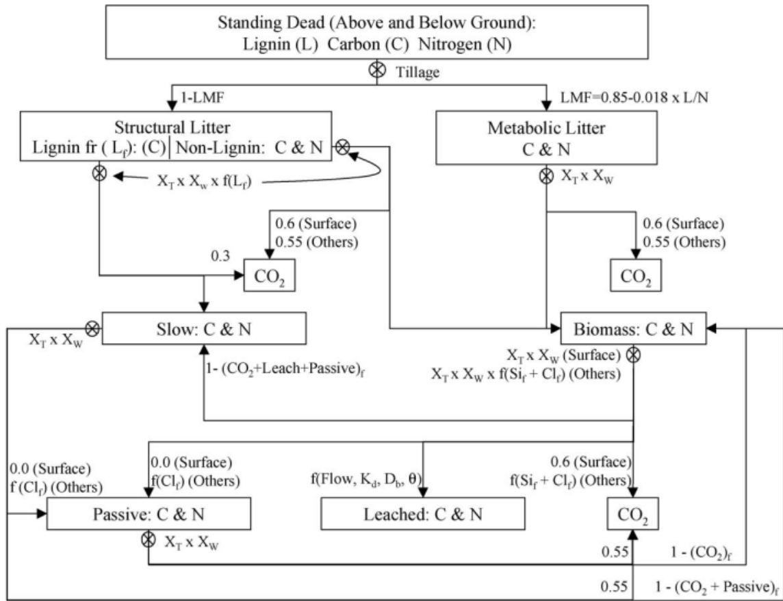
Figure 2-3 Carbon flows in EPIC. X_W and X_T refer to moisture and temperature control on soil biological processes, LMF = fraction of the litter that is metabolic ( kg\ kg^{-1} ) L_f = fraction of structural litter that is lignin ( kg\ kg^{-1} ); lower case f = “function of”, and subscript f = “fraction”; Sif = fraction of soil mineral component that is silt; Clf = fraction of soil mineral component that is clay; K_d = distribution coefficient of organic compounds between soil solid and liquid phases; DB = soil bulk density; \theta = soil volumetric water content (Izaurrealde et al., 2006)
