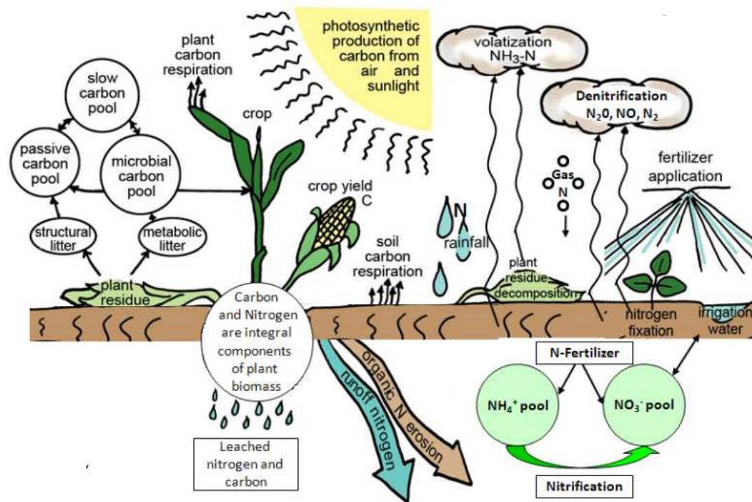
Figure 2-2 Biogeochemical components of the C and N budgets in EPIC (Cooter et al., 2012)
