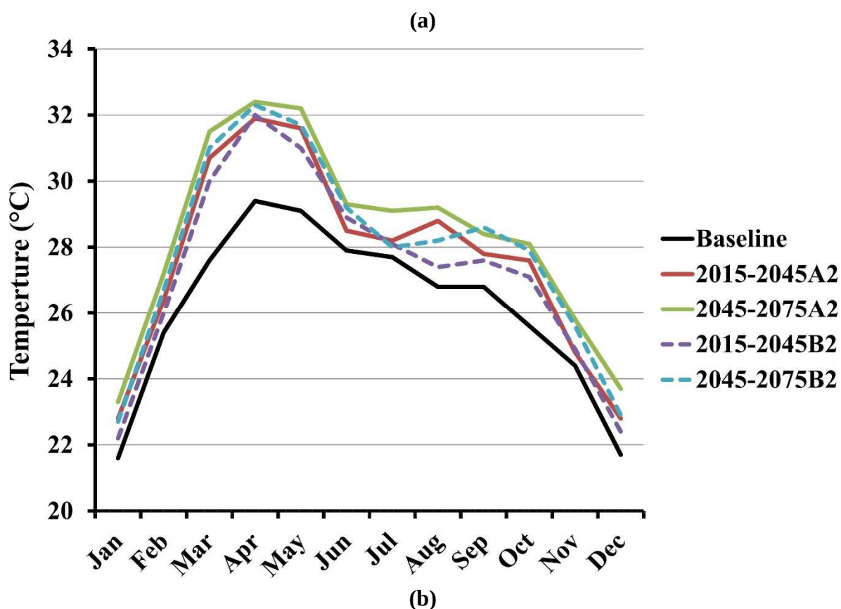
Figure 5-6 Monthly average values of (a) precipitation and (b) temperature for the baseline (1986–2014) and the A2 and B2 scenarios for 2015–2045 and 2045–2075
