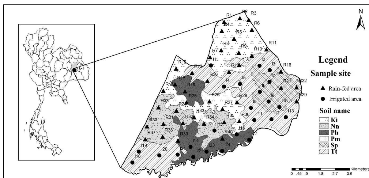
Figure 5-1. Study area and soil series (LDD, 2003)
