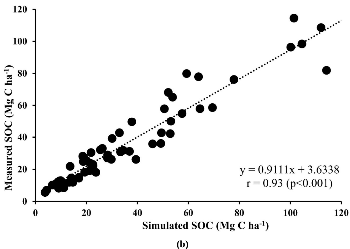
Figure 5-5 Comparison between measured and simulated values of (a) rice yield and (b) SOC
