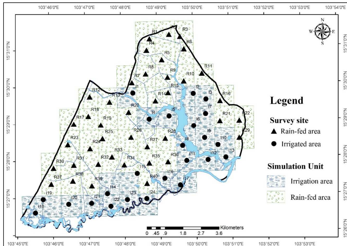
Figure 5-3 The location of data collection and simulation unit
