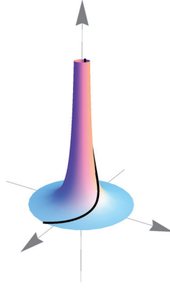
Figure 4.1: The curve of type (3) ( \kappa_1 = \kappa_2 = 0 ) and the surface (x^2 + y^2)z = 1 .
