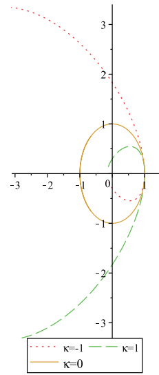
Figure 2.4: Centraffine plane curve (ii-4)
