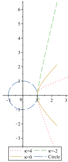
Figure 2.1: Centraffine plane curve (i)
