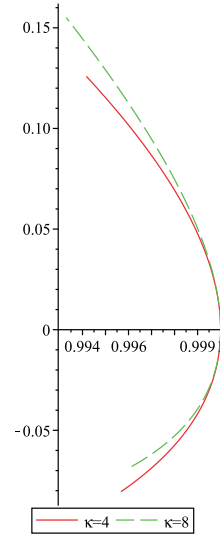
Figure 2.2: Centraffine plane curve (ii-1)
