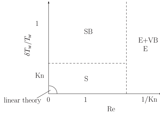
Figure 1: Fluid-dynamic-type equations in the plane (\text{Re}, \delta T_w / T_w) . ( \text{Re} : the Reynolds number, \delta T_w / T_w : the reference relative variation of the wall temperature)
