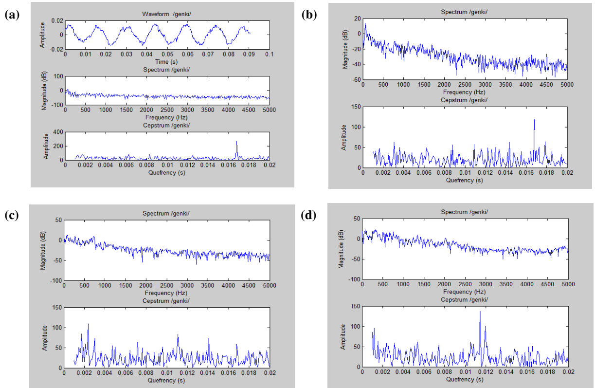
Figure 2.14: (a) The waveform, spectrum and cepstrum of clean speech /genki/ (b) Spectrum and Cepstrum with babble noise at 20 dB, (c) Spectrum and Cepstrum with babble noise at 10 dB (d) Spectrum and Cepstrum with babble noise at 0 dB SNR
