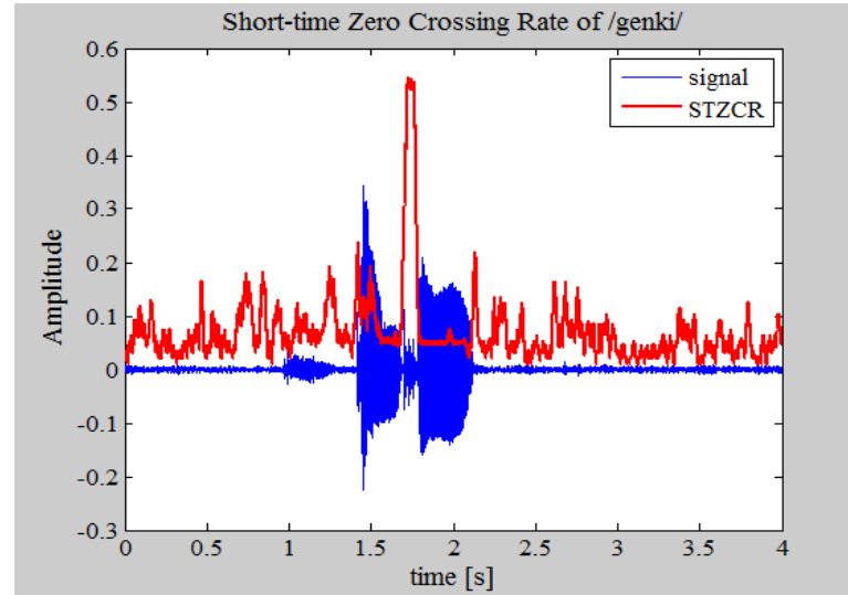
Figure 3.5: Zero-crossing rate of frames of clean speech phrase /genki/
