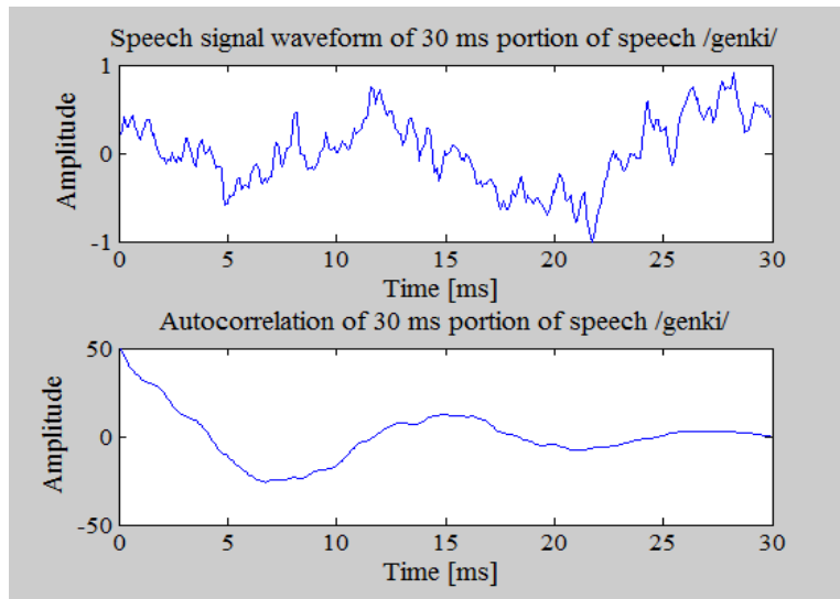
Figure 3.2: Waveform and Autocorrelation of 30 ms Unvoiced portion of speech /genki/
