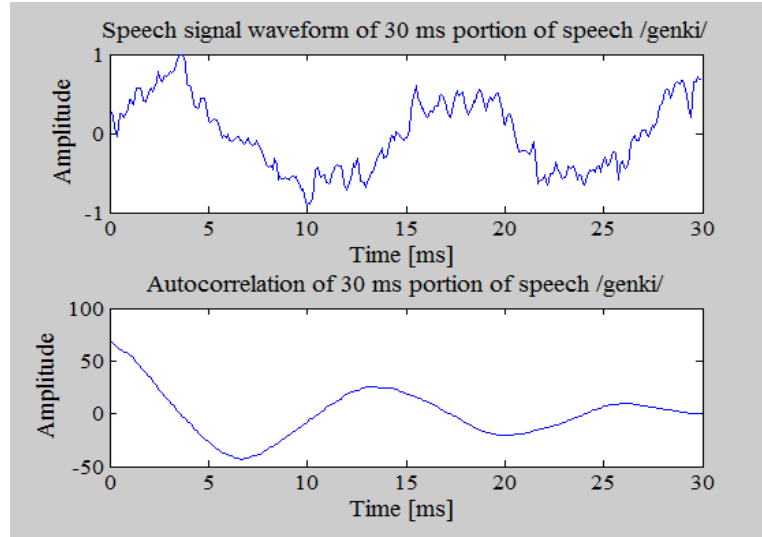
Figure 3.1: Waveform and Autocorrelation of 30 ms Voiced portion of speech /genki/
