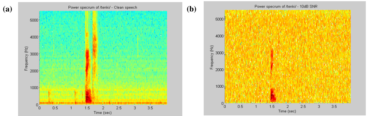
Figure 2.15: (a) The power spectrum of clean speech /tenki/ (b) power spectrum with white noise at 10 dB SNR
