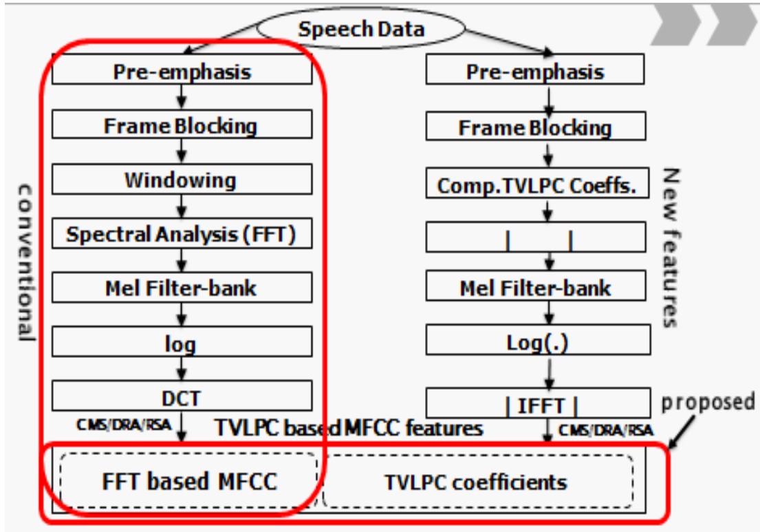
Figure 2.6: Feature estimation process using mel Filtered TVLCP Coefficients.
