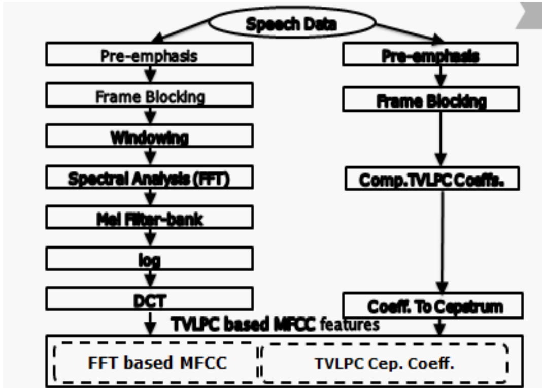
Figure 2.5: Feature estimation process with direct converted TVLPC coefficients.
