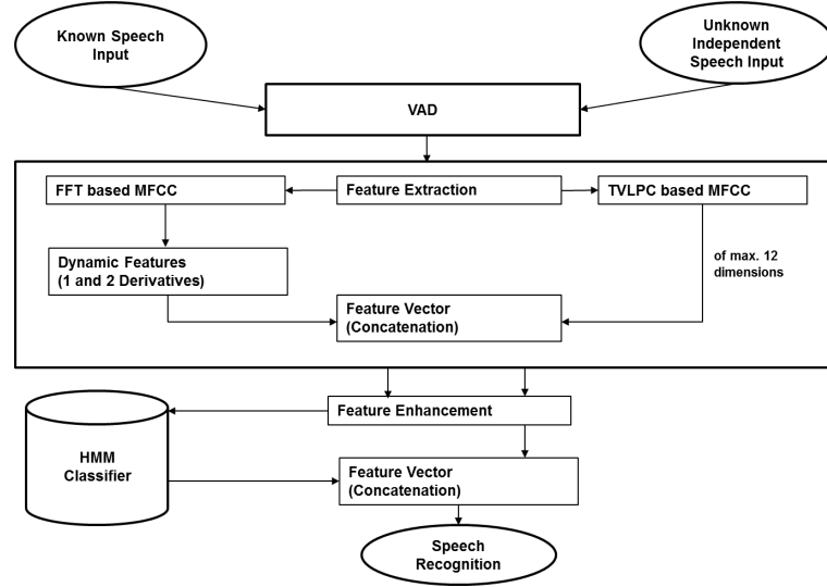
Figure 2.1: ASR system diagram
