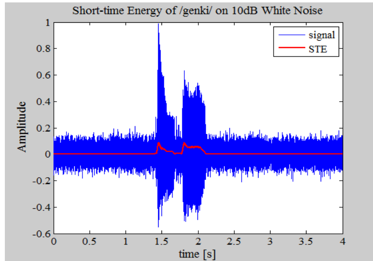
Figure 3.7: Short-time energy of frames of a noisy speech signal at 10 dB SNR
