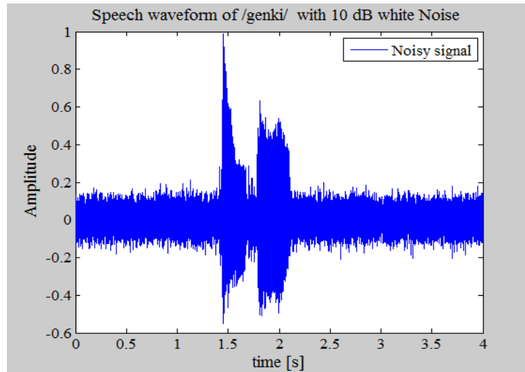
Figure 3.6: Noisy speech signal at 10 dB
