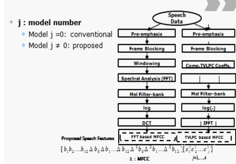
Figure 2.10: Proposed concatenated speech features, with model 0 as conventional approach.
