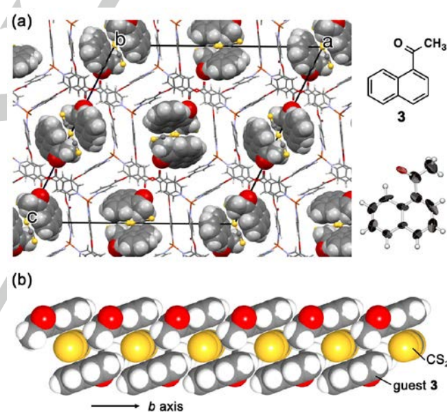
Figure 4. (a) Crystal structure of inclusion complex 3·2 (left: packing structure viewed along the b axis; guest 3 , solvent \text{CS}_2 , and host 2 are drawn as CPK, ball-and-stick, and stick models, respectively; right: ORTEP drawing of guest 3 with 50% thermal ellipsoids). (b) Double-line arrangement of guests 3 with \text{CS}_2 molecules inside the 1D channel of host 2 .
