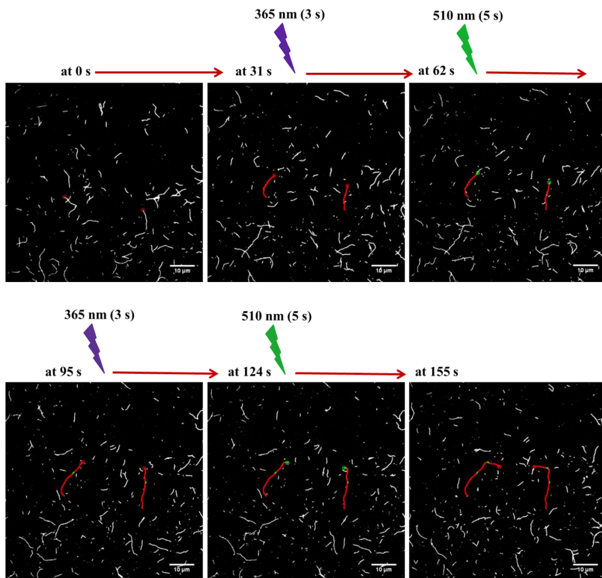
Figure 5. Fluorescence images of F-actin motility driven by trans and cis state of AzoTP (40 \mu M) by in-situ photo-regulation experiment with alternating irradiation at 365 nm (3 s) and 510 nm (5 s). The distance moved by two actin filaments is indicated in lines by tracking the path of filament heads; red circles denote the position of actin filament heads before irradiation ( trans state), green and red lines denote the distance treaded by F- actin after UV (365 nm) and Vis (510 nm) irradiations respectively.
