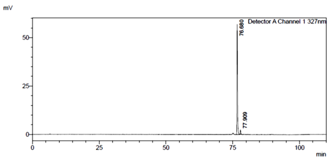
Figure 3. HPLC profile of DimethylazoTP showing > 95% purity.
