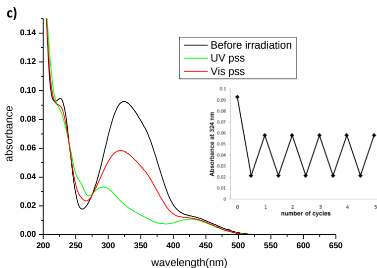
Figure 2. UV-Vis absorption spectra of AzoTP molecules a) DimethylAzoTP, b) AzoethylTP in BRB-80 buffer solution at 25 °C; before irradiation (black line), UV PSS (red line), Vis PSS (green line) and c) AzoethoxyTP in water at 25%. Insets show the absorbance changes a) at 341 nm, b) at 325 nm and c) at 324 nm after the alternate irradiations of 365 and 436 nm for 5 cycles.
