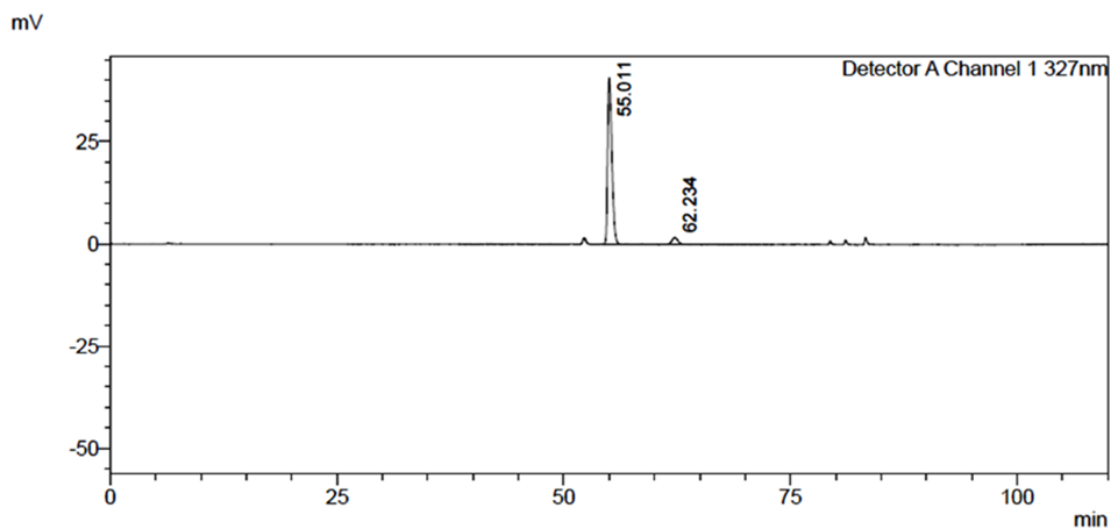
Figure 2. HPLC profile of AzoethoxyTP showing 95% purity.
