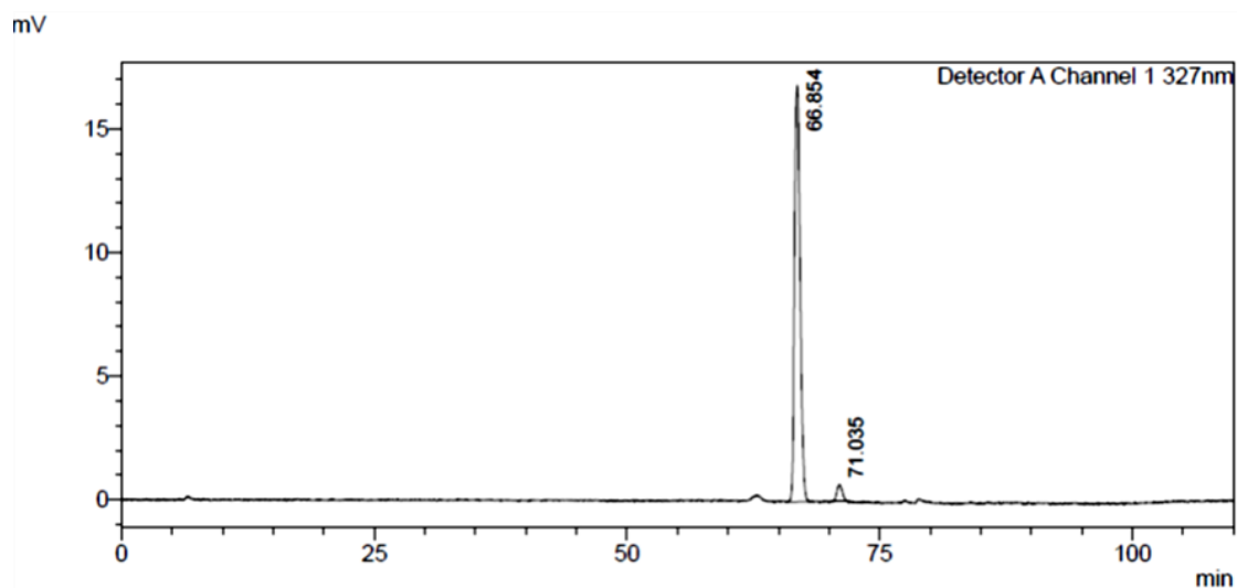
Figure 1. HPLC profile of AzoTP showing > 95% purity.
