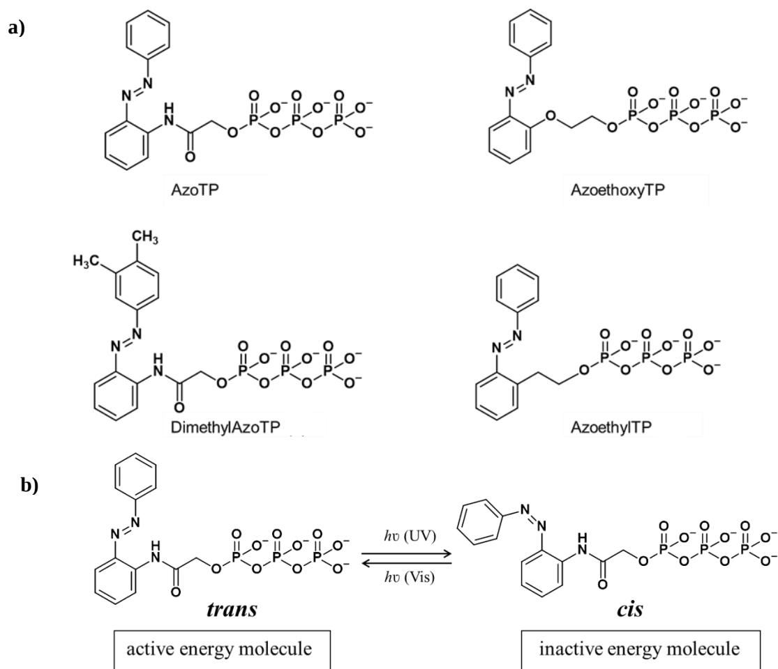
Figure 1. a) Structures of azobenzene based non-nucleoside triphosphates - AzoTP, AzoethoxyTP, DimethylAzoTP and AzoethylTP. b) Reversible photo-isomerization of AzoTP.
