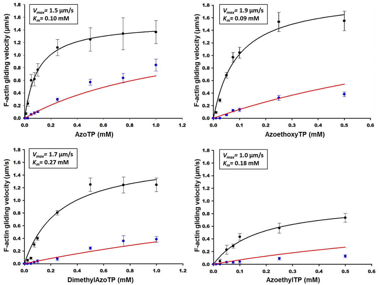
Figure 6. Gliding velocity of actin filaments as a function of AzoTPs concentration. (Black solid circles: velocities before irradiation; black line: curve fitted using Michaelis–Menten equation; Blue circles: velocities after irradiating at 365 nm; red line: theoretical curve derived from the black line for remaining trans in the cis -rich state.) Error bars: standard deviations for 10 actin filaments.
