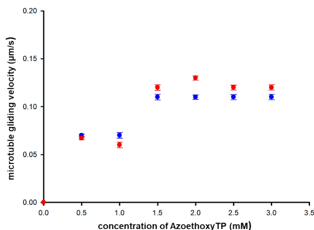
Figure 7. Gliding velocity of microtubules with respect to the concentration of AzoethoxyTP. Blue circles: velocity before irradiation ( trans state), red circles: velocity after 365nm irradiation ( cis state). Error bars: standard deviations for 10 actin filaments.
