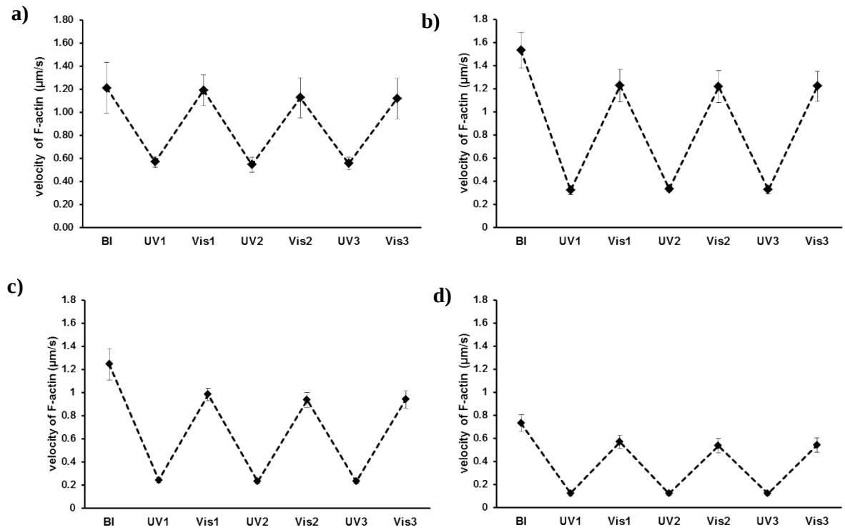
Figure 4. Repeated complete and reversible photoregulation of F-actin gliding velocity induced by a) AzoTP, b) AzoethoxyTP, b) DimethylazoTP and d) AzoethylTP at saturated concentration of 0.5, 0.25, 0.5 and 0.5 mM respectively. (BI: before irradiation; UV: after irradiation with 365 nm light; Vis: after irradiation with 436 nm light). Error bars: standard deviation for 10 actin filaments.
