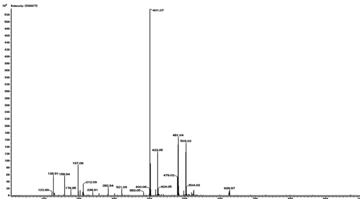
Figure 5. ESI mass spectrum of AzoethoxyTP, the peaks at m/z = 504.03 , 503.02 , 479.02 and 481.04 assigned to the [M-H]^- ions of monosodium tetraprotonated, monosodium triprotonated, diprotonated and tetraprotonated AzoethoxyTP species respectively (calculated mass [M-H]^- for these fragments C_{14}H_{17}N_2O_{11}NaP_3 , C_{14}H_{16}N_2O_{11}NaP_3 , C_{14}H_{15}N_2O_{11}P_3 and C_{14}H_{17}N_2O_{11}P_3 is 504.03 , 503.02 , 479.02 and 481.04 respectively). The peaks at m/z = 424.05 , 423.05 and 401.07 assigned to [M-H]^- ions of monosodium triprotonated, monosodium diprotonated and triprotonated AzoethoxyDP species respectively (calculated mass [M-H]^- for these fragments C_{14}H_{16}N_2O_8NaP_2 , C_{14}H_{15}N_2O_8NaP_2 , C_{14}H_{16}N_2O_8P_2 is 424.05 , 423.05 and 401.07 respectively).
