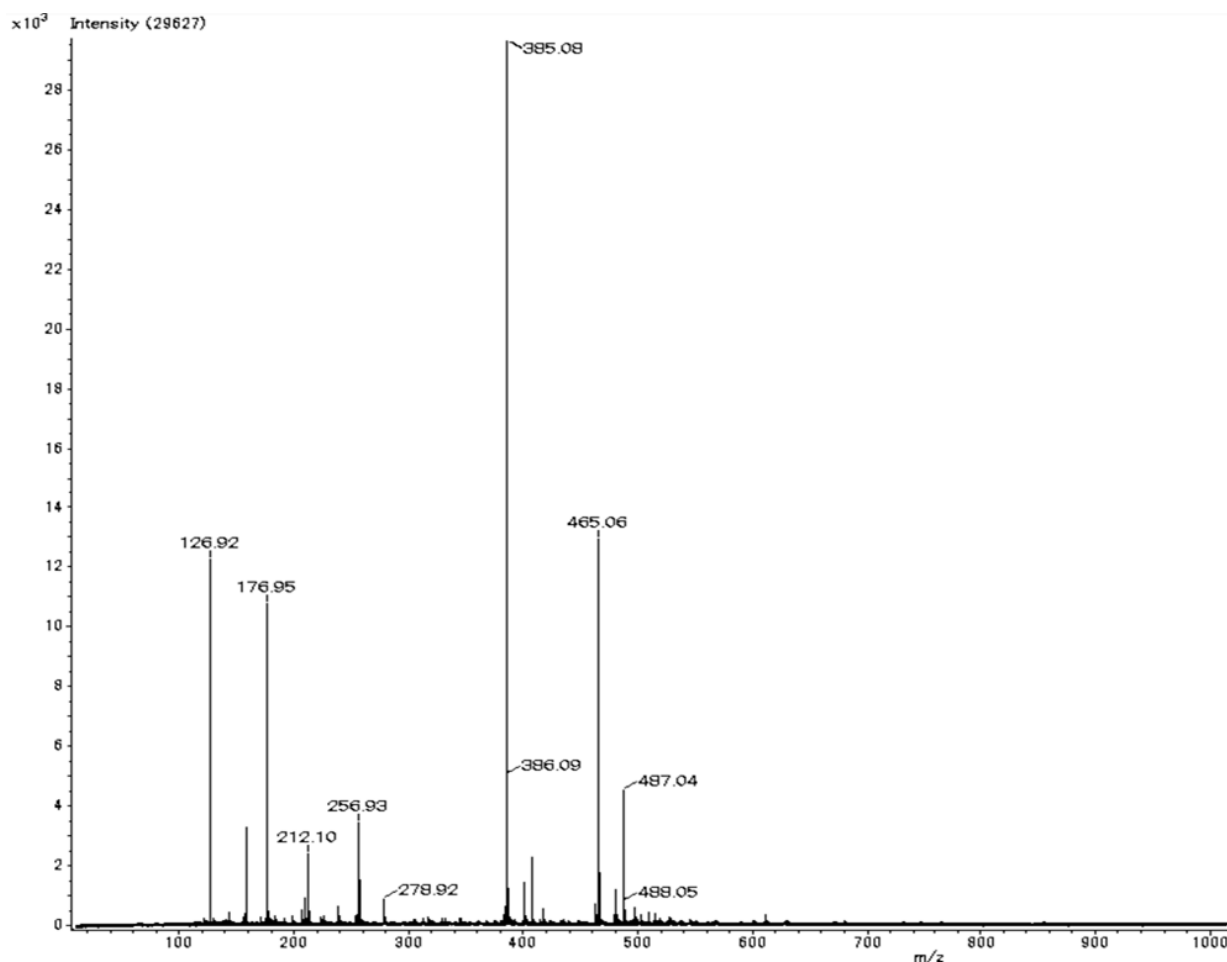
Figure 7. ESI mass spectrum of AzoethylTP, the peaks at m/z = 487.04 , 465.06 and 385.08 can be assigned to the [M-H]^- ions of monosodium triprotonated, tetra-protonated AzoethylTP and tri-protonated AzoethylDP species respectively (calculated mass [M-H]^- for these fragments C_{14}H_{16}N_2O_{10}NaP_3 , C_{14}H_{17}N_2O_{10}P_3 , C_{14}H_{16}N_2O_7P_2 is 487.04 , 465.06 and 385.08 respectively).
