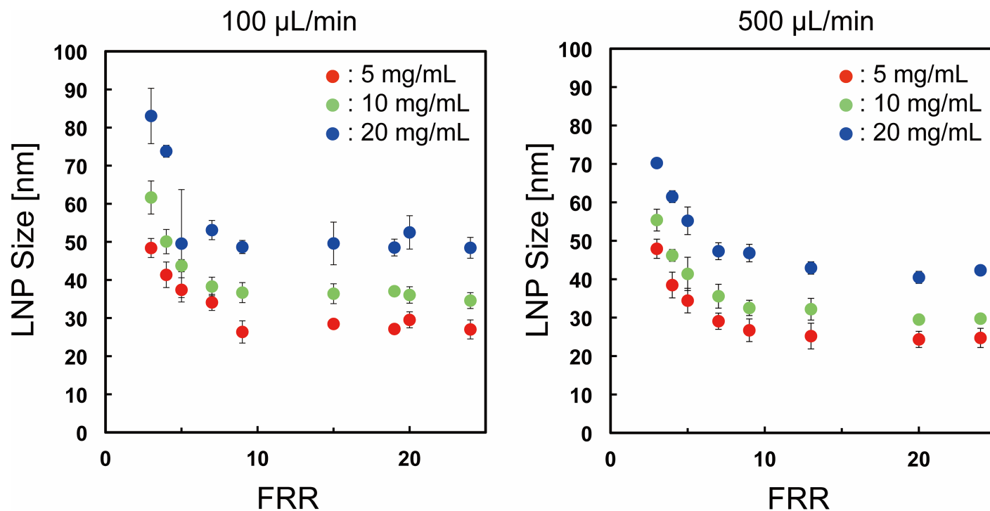
Fig 3. The effect of lipid concentration on LNP size under different flow conditions. The error bars represent the standard deviation calculated from repeating each LNP formation experiment at least three times.
