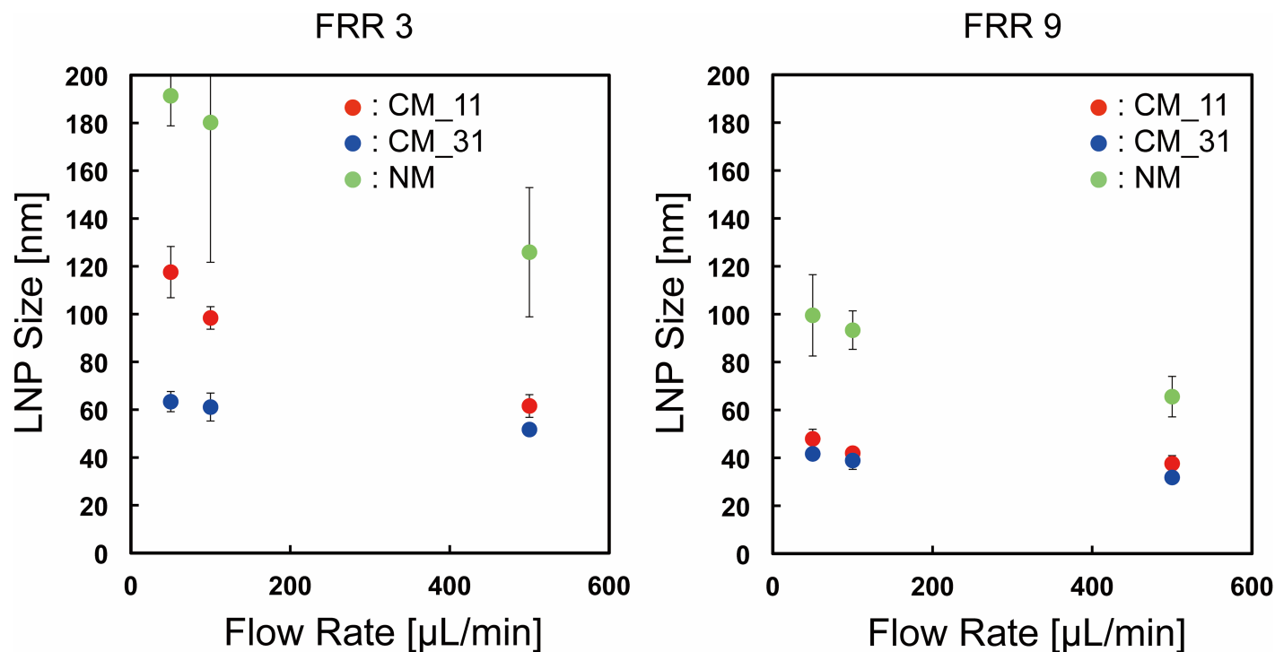
Fig 5. The effect of mixer structures on the LNP size at different flow conditions. The error bars represent the standard deviation calculated from repeating each LNP formation experiment at least three times.
