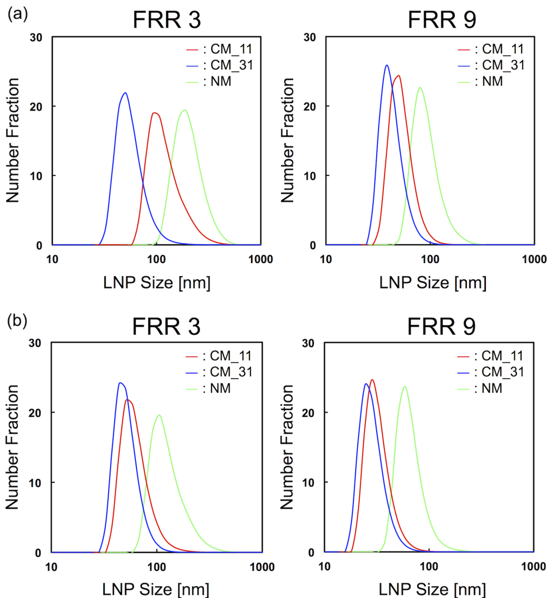
Fig 4. Size distributions of LNPs formed in the microfluidic devices at FRR of 3 and 9. The flow rates were (a) 50 \mu\text{L}/\text{min} and (b) 500 \mu\text{L}/\text{min} .
