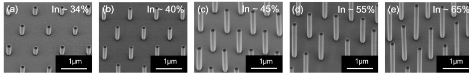
FIG. 1. 30°-tilted SEM image view showing growth results of InGaAs NWs on Si with d_0=150 nm and a=1000 nm. The In composition of vapor phase is (a) 34%, (b) 40%, (c) 45%, (d) 55%, and (e) 65%.
