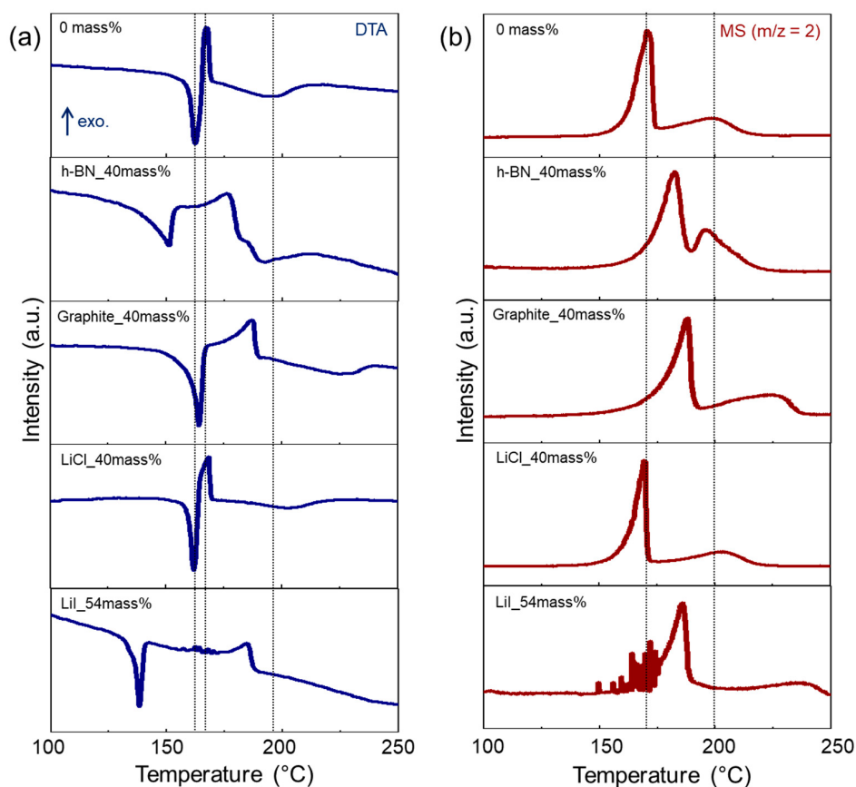
Figure 7. Hydrogen desorption profiles of \text{LiAlH}_4/\text{X} ( \text{X} = graphite, LiCl, and LiI) composites. The profiles of milled \text{LiAlH}_4 and \text{LiAlH}_4/\text{h-BN} composites are shown as the references: (a) DTA and (b) MS ( m/z = 2 , \text{H}_2 ) profiles. Heating rate was 5 \text{ }^\circ\text{C}\cdot\text{min}^{-1} .
