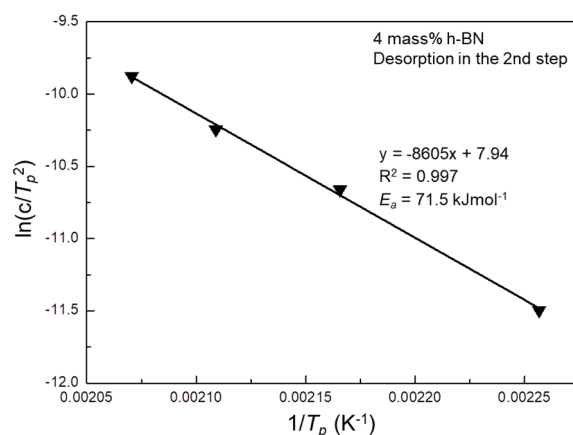
Figure 6. Kissinger plots for the hydrogen desorption in the second step of \text{LiAlH}_4 /4 mass % h-BN composite. Heating rates were 2, 5, 8, and 12 \text{ }^\circ\text{C}\cdot\text{min}^{-1} .
