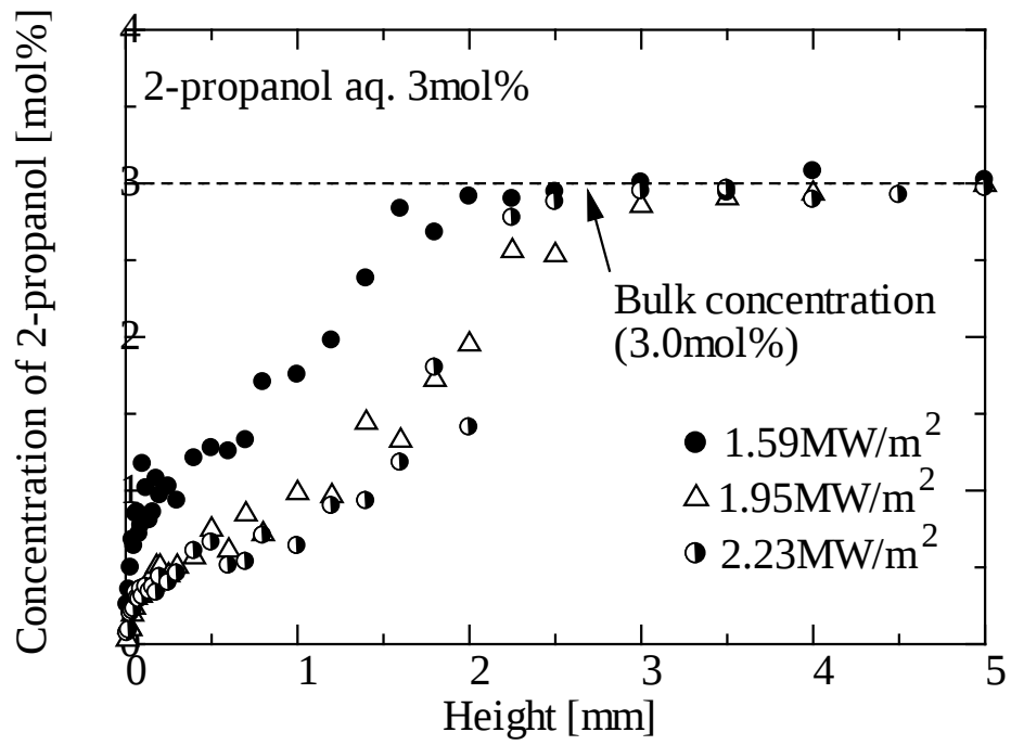
Fig.14 Vertical distributions of 2-propanol concentrations at r=0 mm
