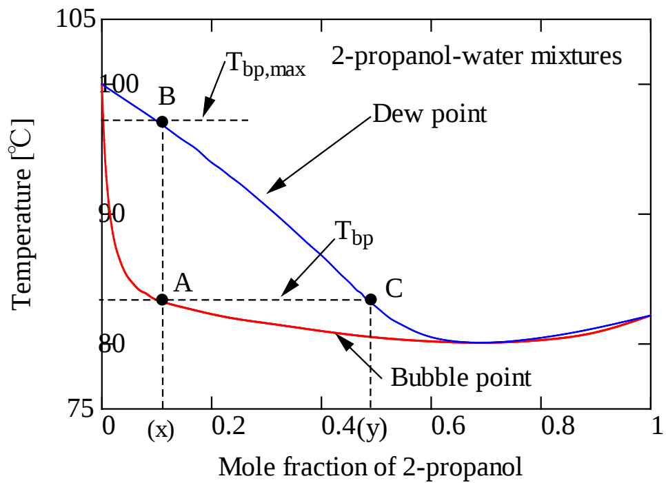
Fig.3 Phase equilibrium diagram of 2-propanol/water mixtures
