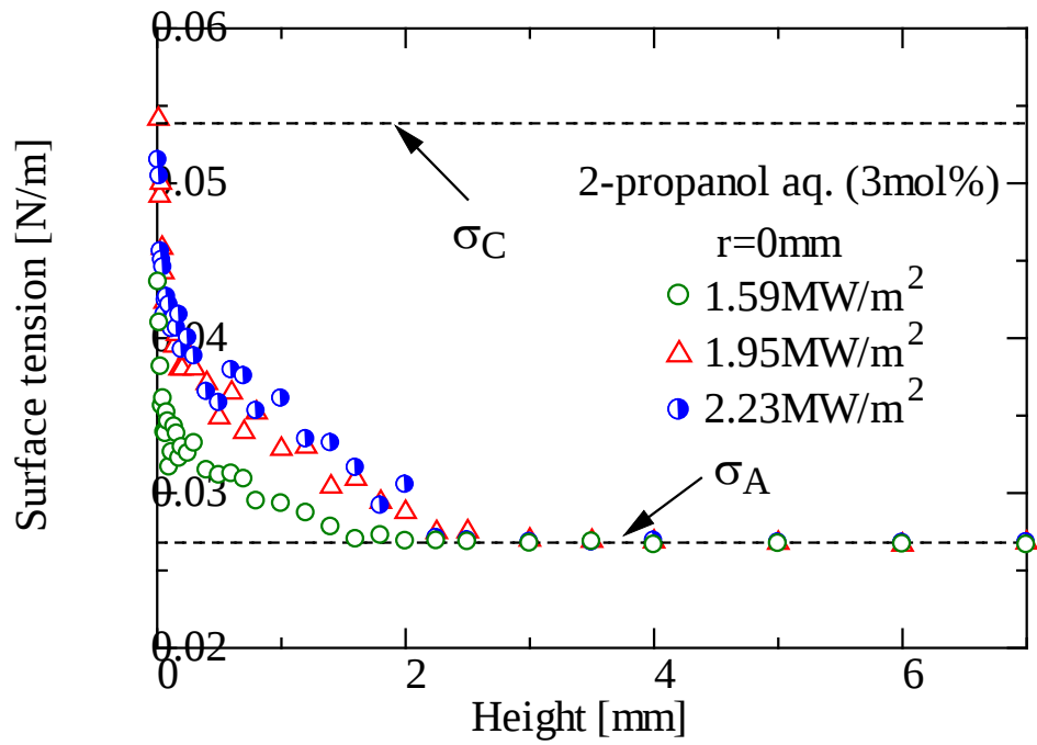
Fig.16 Vertical distributions of surface tension of 2-propanol-water mixture
