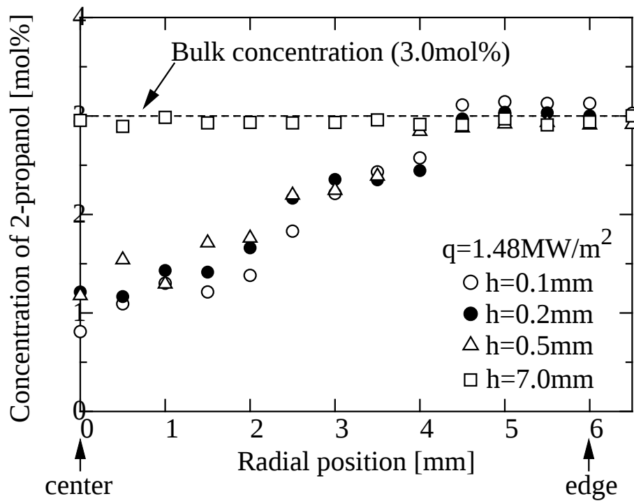
Fig.15 Radial distributions of 2-propanol concentrations
