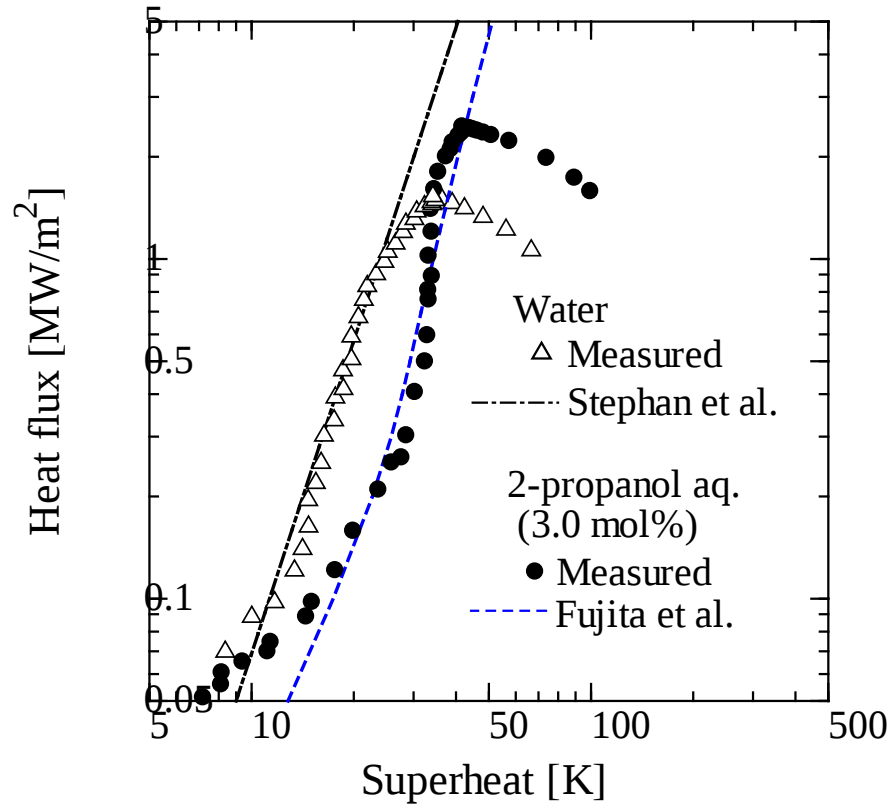
Fig.5 Measured and predicted boiling curves for water and 2-propanol-water mixture (3 mol%)
