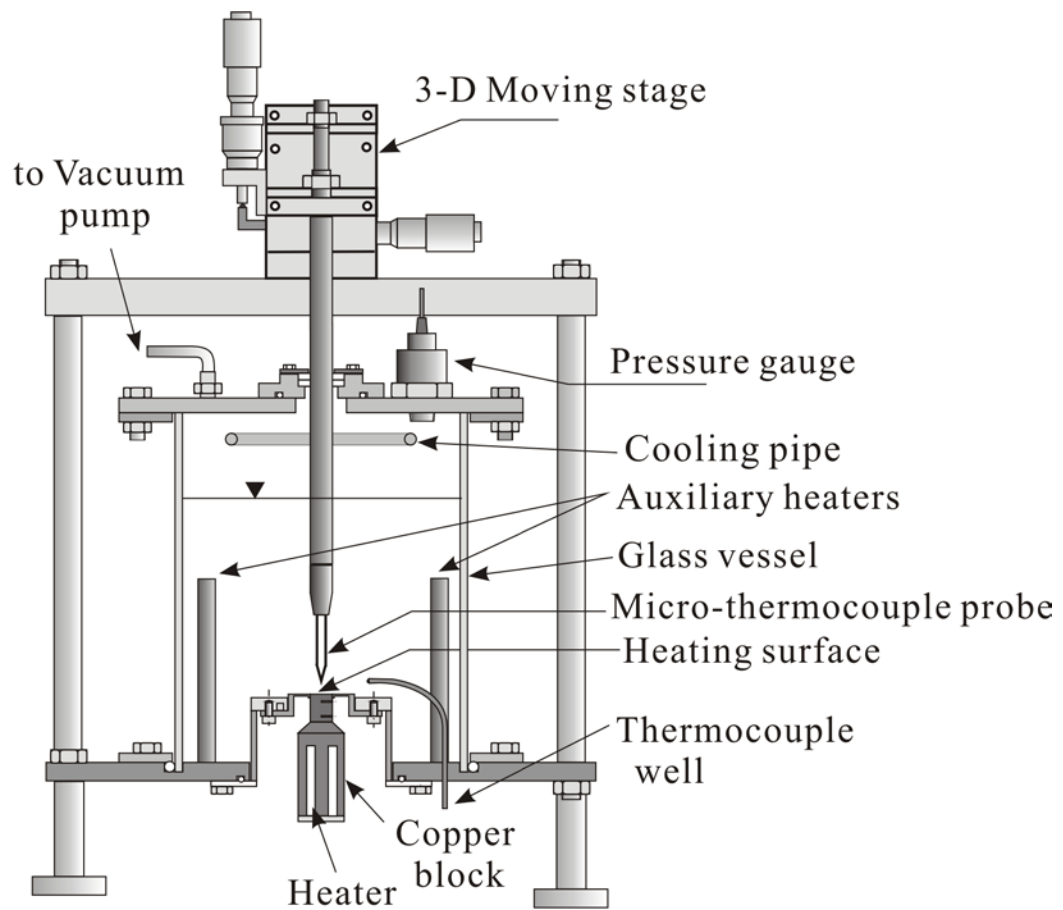
Fig.1 Experimental apparatus
