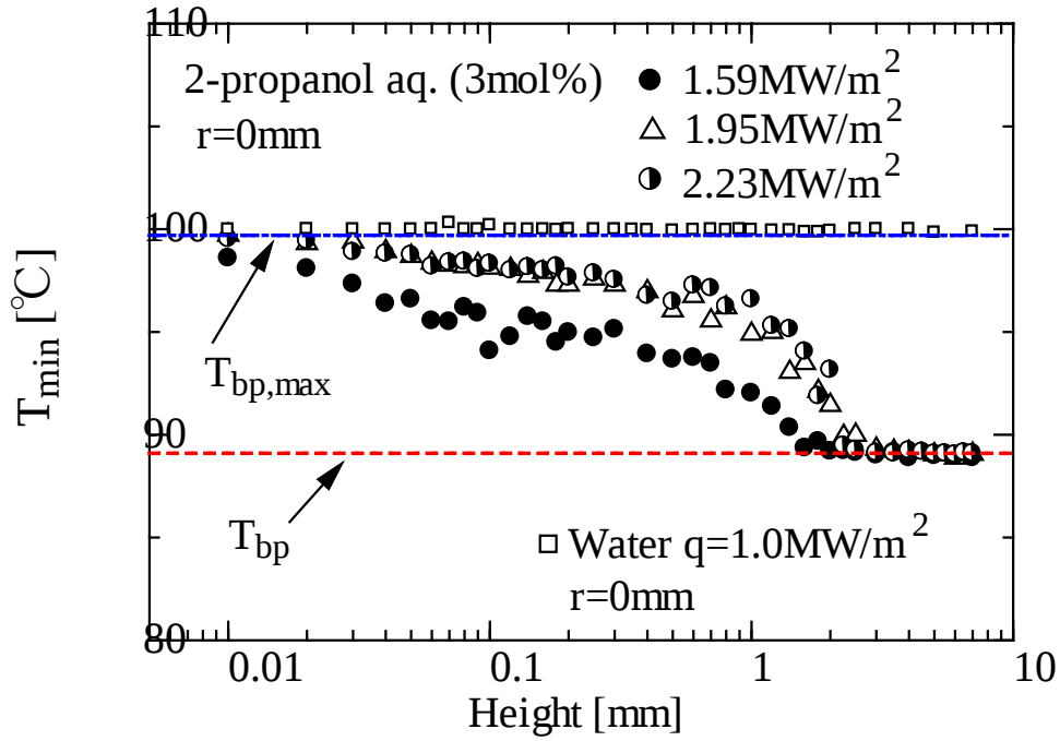
Fig.12 Vertical distributions of T_{\min} for different heat fluxes at r=0 mm (Semi-logarithmic plot)
