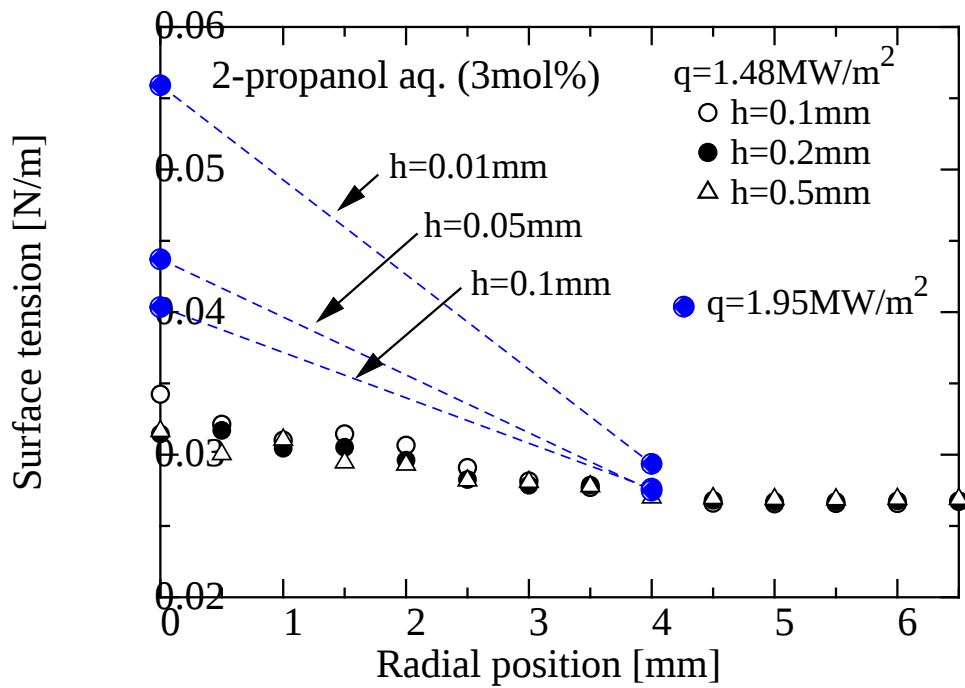
Fig.17 Radial distributions of surface tension of 2-propanol-water mixture
