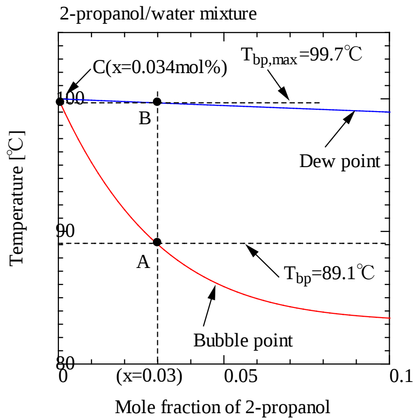
Fig.4 Phase equilibrium diagram of 2-propanol/water mixtures in the range of mole fractions of 2-propanol 0 to 0.1
