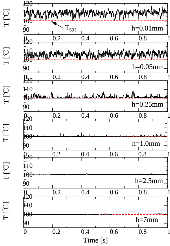
Fig.7 Temperature traces for water measured at r=0 mm ( q=1.0 MW/m 2 )
