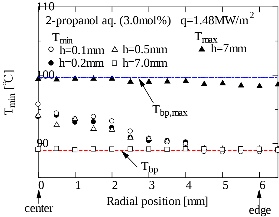
Fig.13 Radial distributions of minimum temperatures (3 mol% 2-propanol/water mixture, q=1.48 MW/m 2 )
