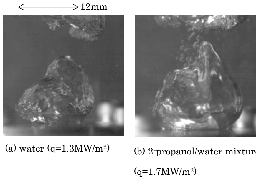
Fig.6 Boiling appearances of (a) water and (b) 2-propanol-water mixture (3 mol%) at high heat fluxes
