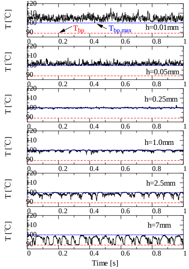
Fig.8 Temperature traces for the 2-propanol/water mixture measured at r=0 mm (3 mol%, q=1.95 MW/m 2 )
