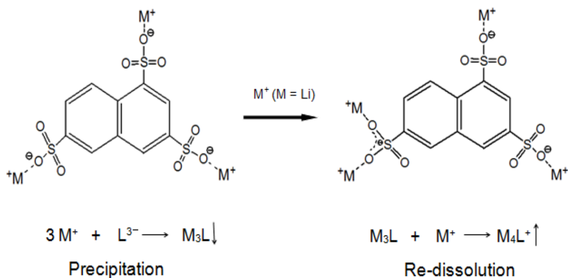
Scheme 1. Successive formation of M_3L and M_4L^+ ( M = Li ) for the 1,3,6-naphthalenetrisulfonate ion in MeCN.
