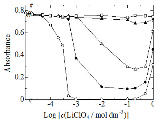
Fig. 5. Absorbance ( \lambda = \text{ca. } 238 \text{ nm} ) of 1.0 \times 10^{-4} \text{ mol dm}^{-3} 1,3,6-naphthalenetrisulfonate in the presence of \text{LiClO}_4 in MeCN-MeOH mixtures: ( \circ ) 0; ( \bullet ) 5.0; ( \Delta ) 7.0; ( \blacktriangle ) 10; ( \square ) 20% (v/v) of MeOH.
