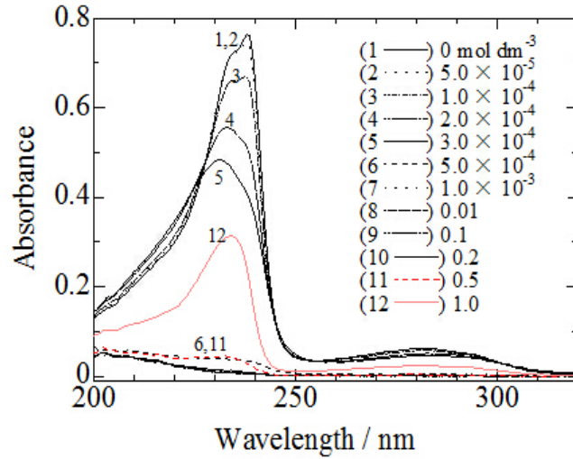
Fig. 1. The UV spectra of 1.0 \times 10^{-4} \text{ mol dm}^{-3} 1,3,6-naphthalenetrisulfonate ion (0.1 cm path-length) with increasing concentration of LiClO_4 in MeCN.
