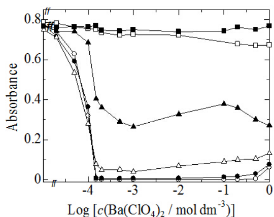
Fig. 11. Absorbance ( \lambda = ca. 238 \text{ nm} ) of 1.0 \times 10^{-4} \text{ mol dm}^{-3} 1,3,6-naphthalenetrisulfonate ion in the presence of \text{Ba}(\text{ClO}_4)_2 in MeCN- \text{H}_2\text{O} mixtures: ( \circ ) 0; ( \bullet ) 5.0; ( \Delta ) 10; ( \blacktriangle ) 15; ( \square ) 20; ( \blacksquare ) 30 % (v/v) of \text{H}_2\text{O} .
