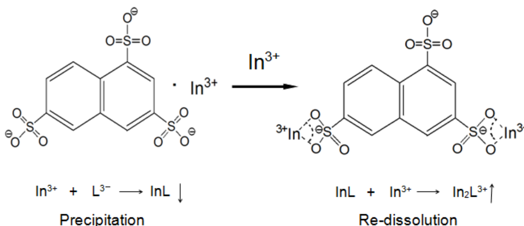
Scheme 2. Successive formation of \text{InL} and \text{In}_2\text{L}^{3+} for the 1,3,6-naphthalenetrisulfonate ion in MeCN- \text{H}_2\text{O} or sole alcohols.
