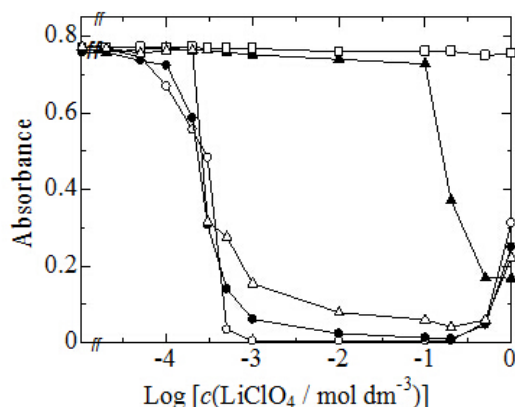
Fig. 4. Absorbance ( \lambda = \text{ca. } 238 \text{ nm} ) of 1.0 \times 10^{-4} \text{ mol dm}^{-3} 1,3,6-naphthalenetrisulfonate in the presence of \text{LiClO}_4 in MeCN- \text{H}_2\text{O} mixtures: ( \circ ) 0; ( \bullet ) 1.0; ( \Delta ) 2.0; ( \blacktriangle ) 5.0; ( \square ) 10% (v/v) of \text{H}_2\text{O} .
