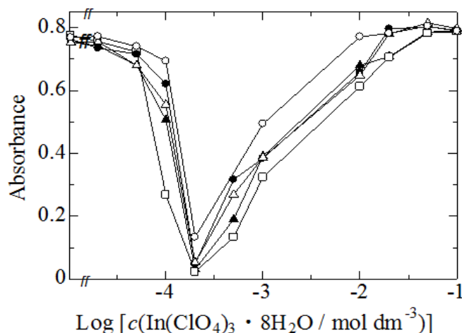
Fig. 14. Absorbance ( \lambda = ca. 238 nm) of 1.0 \times 10^{-4} mol dm -3 1,3,6-naphthalenetrisulfonate in the presence of In(ClO 4 ) 3 ·8H 2 O in primary alcohols: (○) MeOH; (●) EtOH; (Δ) 1-PrOH; (▲) 1-BuOH; (□) 1-HexOH.
