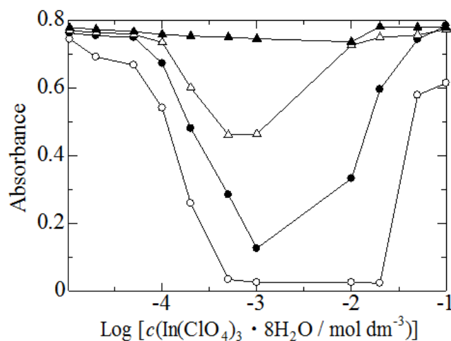
Fig. 13 Changes in absorbance ( \lambda = ca. 238 \text{ nm} ) of 1.0 \times 10^{-4} \text{ mol dm}^{-3} 1,3,6-naphthalenetrisulfonate ion with increasing concentration of \text{In}(\text{ClO}_4)_3 \cdot 8\text{H}_2\text{O} in MeCN- \text{H}_2\text{O} mixtures: (○) 10; (●) 30; (△) 50; (▲) 100% (v/v) of \text{H}_2\text{O} .
