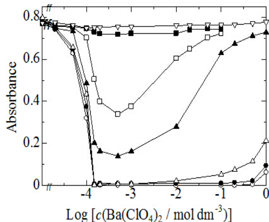
Fig. 12. Absorbance ( \lambda = ca. 238 \text{ nm} ) of 1.0 \times 10^{-4} \text{ mol dm}^{-3} 1,3,6-naphthalenetrisulfonate ion in the presence of \text{Ba}(\text{ClO}_4)_2 in MeCN-MeOH mixtures: ( \circ ) 0; ( \bullet ) 10; ( \Delta ) 20; ( \blacktriangle ) 40; ( \square ) 50; ( \blacksquare ) 70; ( \nabla ) 100 % (v/v) of MeOH
