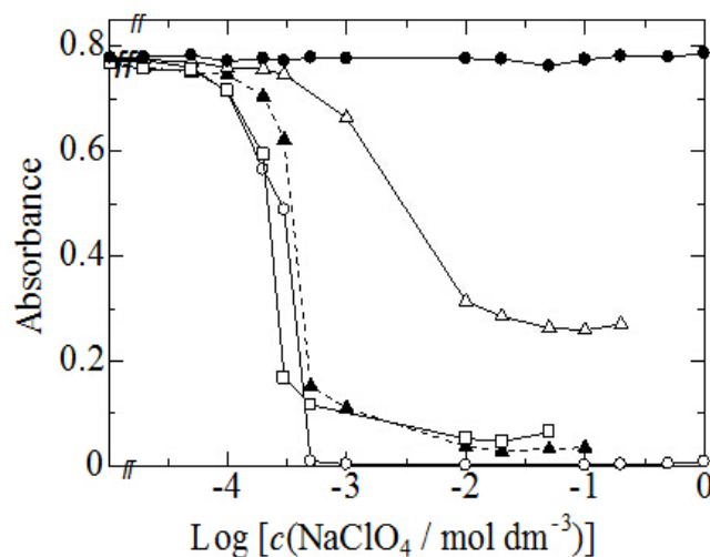
Fig. 3. Changes in absorbance ( \lambda = \text{ca. } 238 \text{ nm} ) of 1.0 \times 10^{-4} \text{ mol dm}^{-3} 1,3,6-naphthalenetrisulfonate ion with increasing concentration of \text{NaClO}_4 in different solvents: (●) EtOH; ( \Delta ) 1-PrOH; ( \blacktriangle ) 1-BuOH; ( \square ) 1-HexOH; ( \circ ) MeCN.
