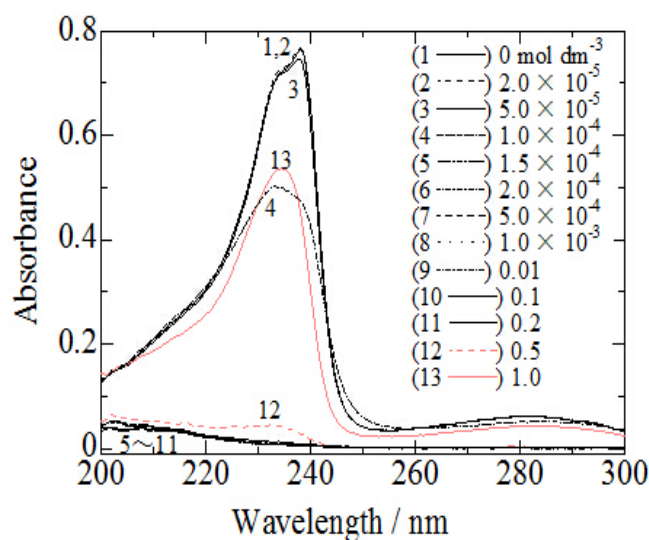
Fig. 6. UV spectra of 1.0 \times 10^{-4} \text{ mol dm}^{-3} 1,3,6-naphthalenetrisulfonate ion (0.1 cm path-length ) with increasing concentration of \text{Mg}(\text{ClO}_4)_2 in MeCN.
