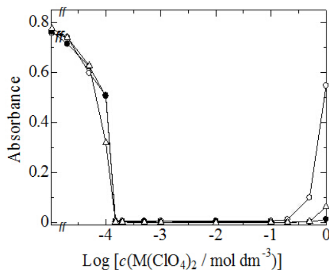
Fig. 7. Changes in absorbance ( \lambda = ca. 238 \text{ nm} ) of 1.0 \times 10^{-4} \text{ mol dm}^{-3} 1,3,6-naphthalenetrisulfonate ion with increasing of alkaline earth metal ions in MeCN: ( \circ ) \text{Mg}(\text{ClO}_4)_2 ; ( \bullet ) \text{Ca}(\text{ClO}_4)_2 ; ( \Delta ) \text{Ba}(\text{ClO}_4)_2 .
