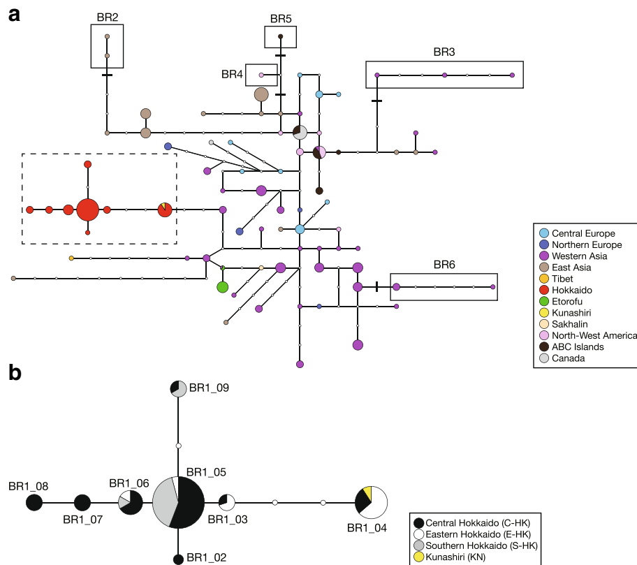
Fig. 2 a Median-joining haplotype network for brown bears, based on Y-chromosomal compound haplotypes combined with Y-linked SNPs from a 3.1 kb data set and Y-linked microsatellites. Haplotypes enclosed by a dashed line are from Hokkaido (including one Kunashiri brown bear). Haplotypes enclosed by solid lines denote the same haplotypes (BR2–BR6) as those distinguished by only the 3.1 kb Y-linked data set. The remaining haplotypes have the same haplotype (BR1) distinguished by only the 3.1 kb data set. Each color represents a different brown bear population. Each black bar crossing a network line denotes a single mutational step revealed by a single nucleotide polymorphism. Small, open circles indicate intermediate haplotypes not actually observed; each line connecting two haplotype circles represents single microsatellite mutational steps. The size of each colored haplotype circle is proportional to the number of individuals having that haplotype. b MJ network for Hokkaido brown bears (including one from Kunashiri Island), based on the same data as above. Symbols and conventions are as for (a)
