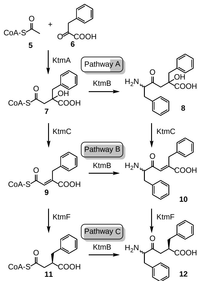
Figure 2. Proposed biosynthetic pathways for the pseudodipeptide in ketomemicins B3 and B4.
