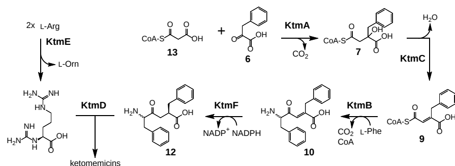
Figure 6. Biosynthesis of ketomemicins
