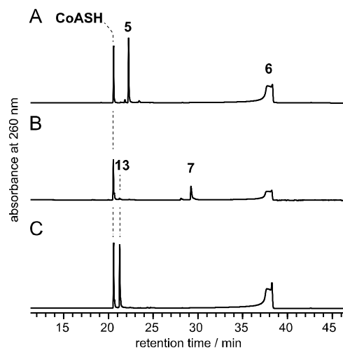
Figure 3. HPLC analysis of the recombinant KtmA reaction. (A) Reaction between acetyl-CoA ( 5 ) and phenylpyruvate ( 6 ). (B) Reaction between malonyl-CoA ( 13 ) and phenylpyruvate. (C) Control reaction without the enzyme.
