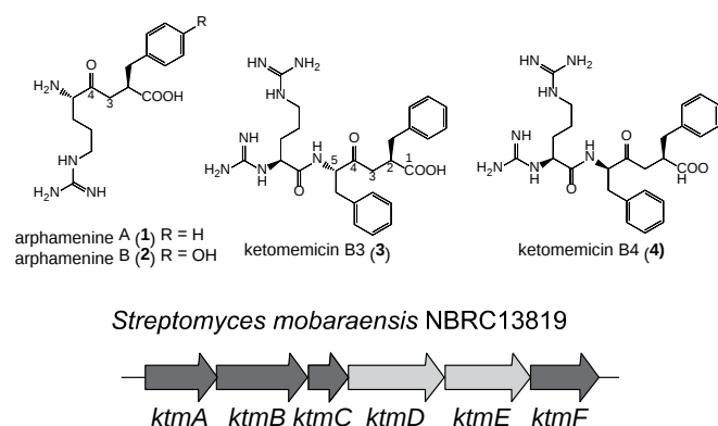
Figure 1. (A) Structures of arphamenines and ketomemicins, and (B) the ketomemicin biosynthetic gene cluster of S. mobaraensis .
