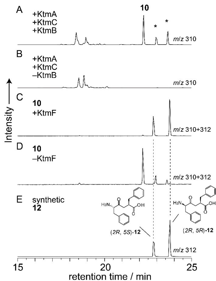
Figure 5. LC-MS analysis of enzyme reactions. (A) Reaction of KtmA + KtmC + KtmB and (B) control reaction without KtmB. The LC-MS profile was monitored at m/z 310 ( 10 , [M+H]^+ ). Compounds with an asterisk are likely stereo- and positional isomers of 10 and we observed interconversion among three compounds upon incubation in the reaction buffer. (C) Reaction of KtmF with purified 10 , (D) control reaction without KtmF. The LC-MS profile was monitored at m/z 312 ( 12 , [M+H]^+ ) and 310 ( 10 , [M+H]^+ ). (E) Synthetic standard 12 . The LC-MS profile was monitored at m/z 312 ( 12 , [M+H]^+ ).
