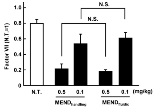
Figure 2. Comparison of the silencing efficiency on handling and fluidic preparation. To compare the silencing effect of the YSK-MEND prepared using the microfluidic device (YSK05/chol 70/30, PEG-DMG 1 mol%, MEND fluidic ) with that of YSK-MEND prepared by the handling method (YSK05/chol 70/30, PEG-DMG 3 mol%, MEND handling ), mice were treated with both MENDs at a dose of 0.1 and 0.5 mg/kg. When the P-value (Student's t-test) exceeded 0.05, the difference was considered to not be significant between MENDs at the same dose. Data represent the mean \pm standard deviation (n=3).
