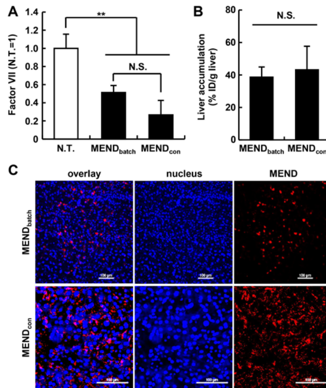
Figure 5. Evaluation of the MEND by large-scale preparation. A) Silencing effect of MEND prepared by traditional batch method (MEND batch ) and MEND prepared by fluidic mixing, TFF purification and sterilization (MEND con ). MENDs were systemically administered into ICR mice at a dose of 0.5 mg/kg, and then FVII mRNA expression level was determined by qRT-PCR. When P-value (Student's t-test) was over 0.05, we considered the difference not significant between MENDs at the same dose. Data represents mean \pm standard deviation (n=3). **:P<0.01 (ANOVA followed by SNK test). B) Liver accumulation of MENDs. Accumulation amount of both MENDs after systemic injection was determined by fluorescent intensity derived from lipid
