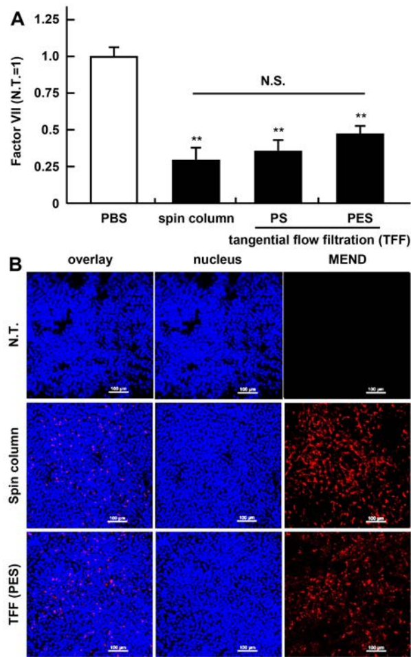
Figure 3. The effect of purification method and membrane material on the silencing effect and efficiency of delivery to liver tissue. A) Silencing effect of MENDs purified by a spin column, TFF (polysulfone) and TFF (polyethersulfone) in the liver tissue. MENDs were administered into ICR mice at a dose of 0.5 mg/kg, and the FVII expression level in the liver tissue was then determined. Data represents the mean \pm standard deviation (n=3). **:P<0.01 (ANOVA, followed by SNK test). B) The distribution of MENDs in liver tissue. Mice were administered fluorescently labeled
