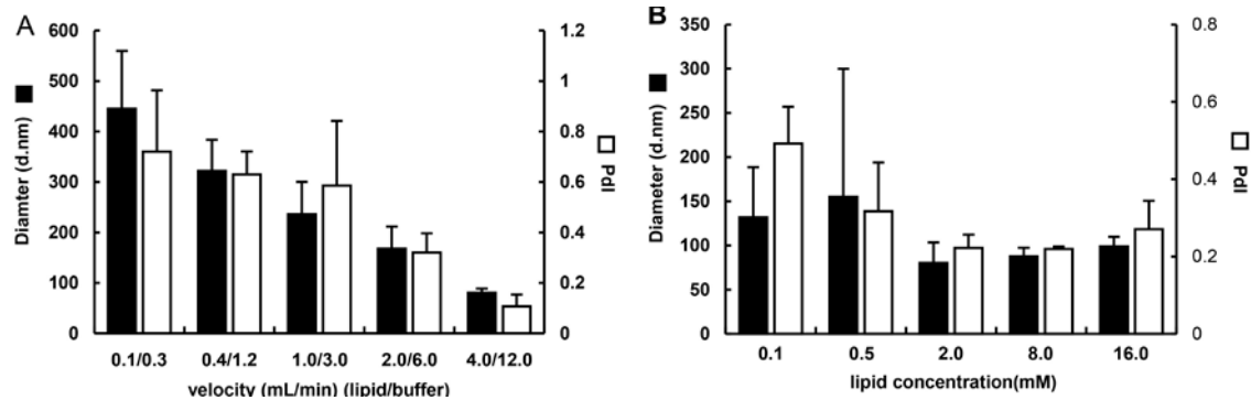
Figure 1. Preparation of PEGylated Liposomes with Fluidic Device. Liposomes
