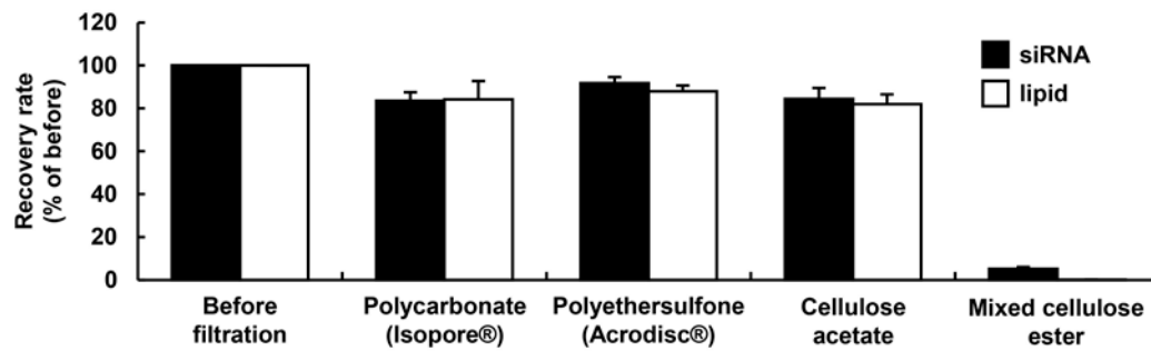
Figure 4. Sterilization of MENDs by filtration. After subjecting the MENDs to sterilization by 0.2 mm-pore filter, siRNA and the lipid envelope recovery rate was determined by comparing fluorescent intensity. Filtration using a filter consisting of polycarbonate (PC), polyethersulfone (PES), cellulose acetate (CA) and mixed cellulose ester (CE) were compared in terms of recovery rate. Data represent the mean \pm standard deviation (n=3).
