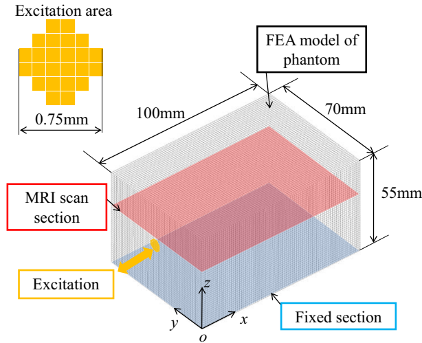
Fig. 3 FEA model [100 mm ( x ) \times 70 mm ( y ) \times 55 mm ( z )] of the tissue phantom and boundary conditions
