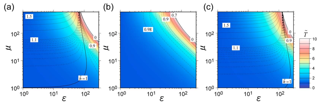
Figure 6. Model calculations showing dimensionless temperature \tilde{T} (color shading) and water level \tilde{h} (contours) at a model time of 100 days. Crater topography is assumed to be a circular-conical shape. The lake-sustainable conditions are largely consistent with the line \tilde{h} = 1 . (a) \lambda = \infty and \gamma = \infty ; i.e., seeping flux and precipitation inflow are negligible. (b) \lambda = 1 and \gamma = \infty ; i.e., the masses of the seepage and bottom input are equal. (c) \lambda = \infty and \gamma = 1 ; i.e., the mass of precipitation is the same as that of the bottom input.
