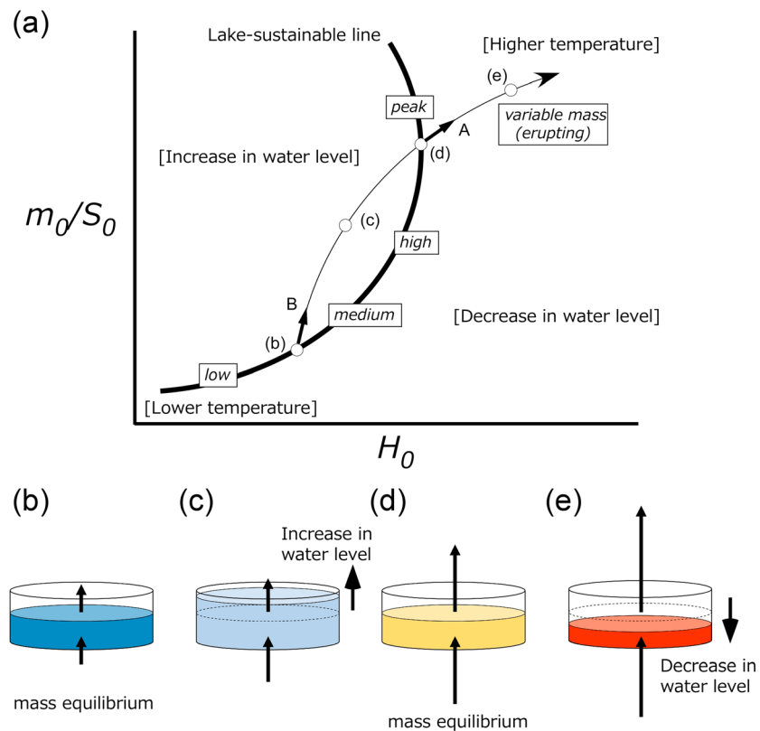
Figure 9. Summary of a variety of volcanic lakes. (a) Diagram of lake-sustainable conditions and patterns of change in water temperature and level. We discuss the behavior of water level in section 5.2 using the examples denoted by arrows A and B. (b–e) Illustrations of mass equilibria of volcanic lakes. Each set of volcanic lake conditions is denoted by letters b–e in Figure 9a. Arrows from lake bottoms and from lake surfaces represent fluid injection and evaporation mass, respectively.
