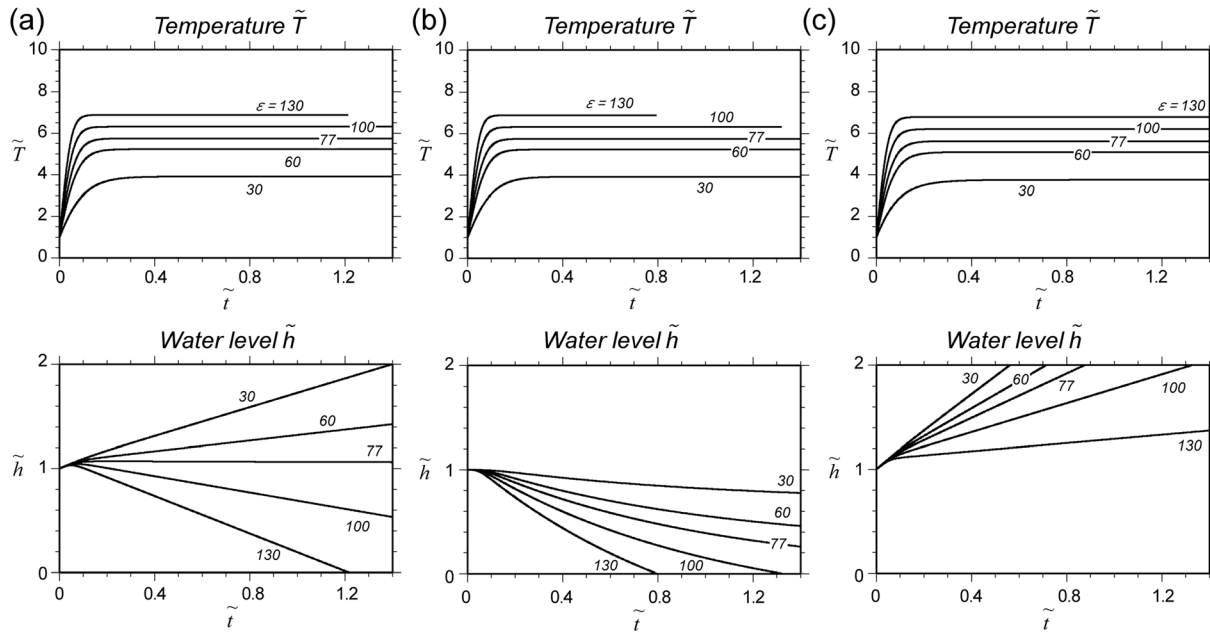
Figure 2. Computed dimensionless water temperature \tilde{T} and level \tilde{h} with a cylindrical topography (Figure 1a). We show five sets of results per pair of subfigures, corresponding to \varepsilon = 30, 60, 77, 100 , and 130 , with \mu = 200 (see text for parameter descriptions). Atmospheric conditions are constant during calculations: air temperature T_a = 10^\circ\text{C} , relative humidity is 80%, air pressure P_a = 8.8 \times 10^4 \text{ Pa} , and wind speed u = 2 \text{ m s}^{-1} . (a) \lambda = \infty and \gamma = \infty ; i.e., seeping output and precipitation input are negligible. (b) \lambda = 1 (seepage mass = bottom input mass) and \gamma = \infty . (c) \lambda = \infty and \gamma = 1 (precipitation mass = bottom input mass).
