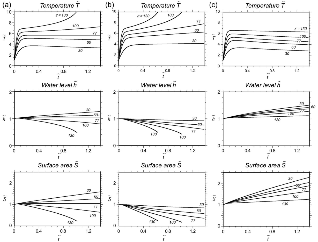
Figure 5. Computed dimensionless water temperature \tilde{T} , level \tilde{h} , and surface area \tilde{S} for crater lakes with conical topographies. The five sets of sample results shown correspond to \varepsilon = 30, 60, 77, 100 , and 130 , with the parameter \mu = 200 (see text for definitions and explanations). Atmospheric conditions are constant during calculations. Computations are ended if the dimensionless water temperature \tilde{T} exceeds 10, corresponding to 100^\circ\text{C} under conditions with T_a = 10^\circ\text{C} . (a) \lambda = \infty and \gamma = \infty ; i.e., seeping output and precipitation input are negligible. (b) \lambda = 1 and \gamma = \infty ; i.e., the seepage and bottom input masses are equal. (c) \lambda = \infty and \gamma = 1 ; i.e., the precipitation mass is the same as the bottom input mass.
