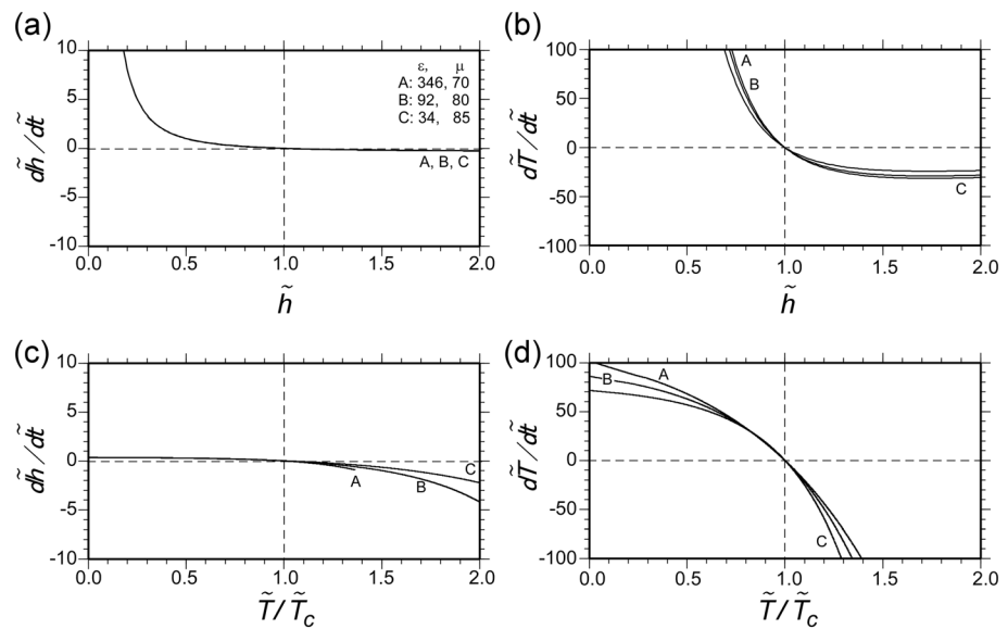
Figure 8. Stability tests of a crater lake with a conical topography, showing (a) d\tilde{h}/d\tilde{t} and (b) d\tilde{T}/d\tilde{t} as functions of \tilde{h} and (c) d\tilde{h}/d\tilde{t} and (d) d\tilde{T}/d\tilde{t} as functions of \tilde{T}/\tilde{T}_c . Three pairs of \epsilon and \mu (labeled A–C in the subfigures) are shown, each of which maintains lake-sustainable conditions. Seepage and precipitation mass are negligible relative to bottom input mass (i.e., \lambda = \infty and \gamma = \infty ).
