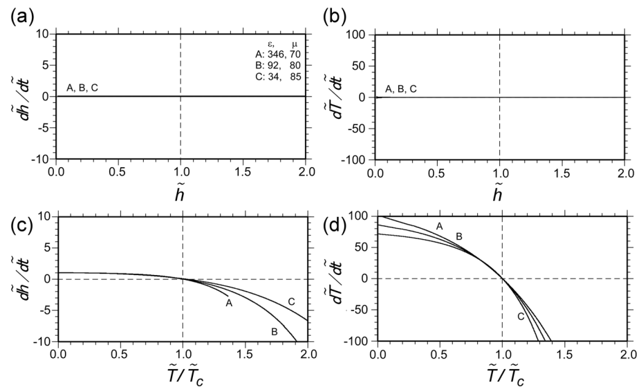
Figure 7. Stability tests of a crater lake with a cylindrical topography, showing (a) \frac{dh}{dt} and (b) \frac{dT}{dt} as functions of \tilde{h} and (c) \frac{dh}{dt} and (d) \frac{dT}{dt} as functions of \tilde{T}/\tilde{T}_c . Three pairs of \epsilon and \mu (represented by A–C) are shown, in which lake sustainable conditions are achieved. Seepage and precipitation mass are negligible relative to bottom input mass (i.e., \lambda = \infty and \gamma = \infty ).
