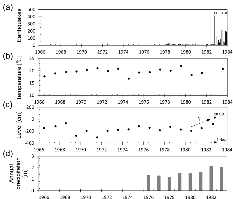
Figure 11. Observation records at Kusatsu-Shirane volcano. (a) Monthly numbers of microearthquakes with maximum amplitudes of >0.05 \mu\text{m} , S-P times of <2 \text{ s} , and the UD component of seismic station “Mizugama Hokuto,” 1 km north-east of Mizugama crater. Data were provided by the Japan Meteorological Agency (JMA). (b) Water temperature measured at the southern shore of Yugama crater lake in June or July of each year [after Ohba et al. , 2008]. (c) Relative changes in the water level of Yugama crater lake, measured at almost the same time as water temperature [after Tokyo Institute of Technology and Sophia University, 1984]. The increase in water level on 28 October 1982 was followed by a rapid decrease in water level. A water level of -859 \text{ cm} was measured on 28 January 1983 because the lake water drained to the new vent that formed on the northern shore of Yugama [Tokyo Institute of Technology and Sophia University, 1984]. (d) Annual precipitation at Kusatsu town, 6 km east of Yugama crater lake, as measured by JMA.
