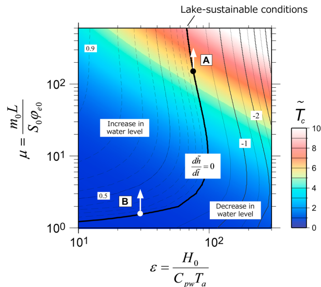
Figure 3. Constant temperature \tilde{T}_c (color) and d\tilde{h}/d\tilde{t} (contours) when water temperature reaches \tilde{T}_c . Crater topography is assumed to be a cylindrical shape. Seeping output and precipitation inflow are negligible relative to the bottom input mass m_0 (i.e., \lambda = \infty and \gamma = \infty ). Lake-sustainable conditions are represented by the line d\tilde{h}/d\tilde{t} = 0 , meaning mass and energy equilibria are simultaneously achieved. We discuss the behavior of the water level in section 3.1.1 using the examples denoted by arrows A and B.
