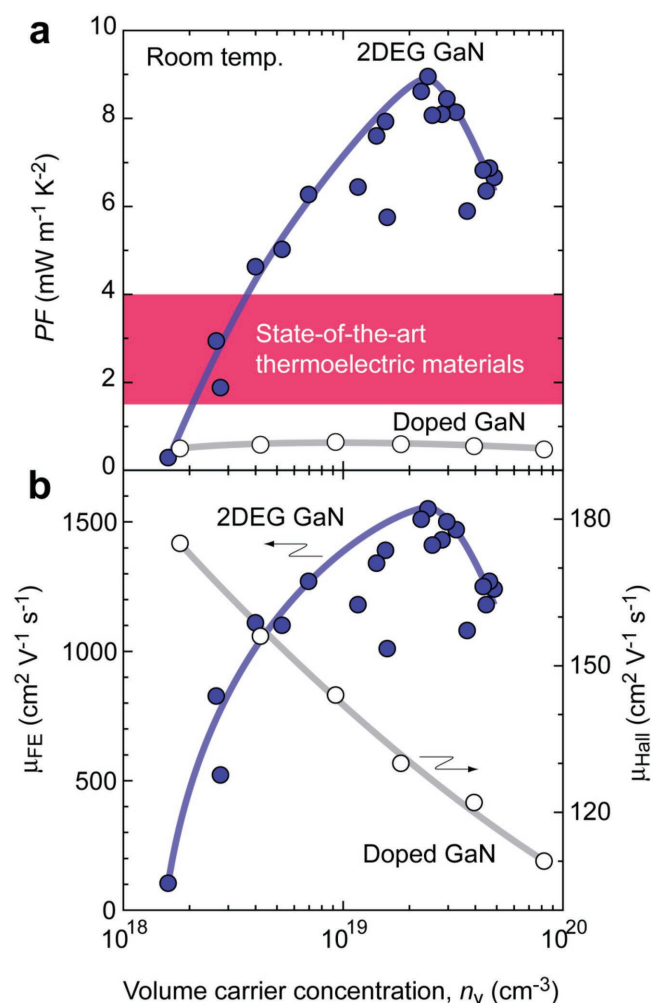
Figure 5. High thermoelectric power factor of high-mobility 2DEG at AlGaIn/GaN interface. Carrier concentration dependence of a) PF and b) carrier mobility ( \mu ) for 2DEG GaN and conventional impurity doped n-type GaN. Maximized PF of the 2DEG with n_v \approx 2.5 \times 10^{19} \text{ cm}^{-3} is \approx 9 \text{ mW m}^{-1} \text{K}^{-2} at room temperature, which is an order magnitude greater than that of doped GaN bulk [19] and a factor of 2–6 greater than that state-of-the-art practical thermoelectric materials ( 1.5\text{--}4 \text{ mW m}^{-1} \text{K}^{-2} ).
