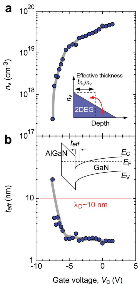
Figure 6. Effective thickness of 2DEG at the AlGaIn/GaN interface. Changes in a) the volume carrier concentration ( n_v ) and b) the effective thickness, which is defined as n_s/n_v , as a function of V_g . n_v means the average volume carrier concentration of 2DEG as schematically shown in the inset of (a). Definition of the effective thickness is shown in the inset of (b).
