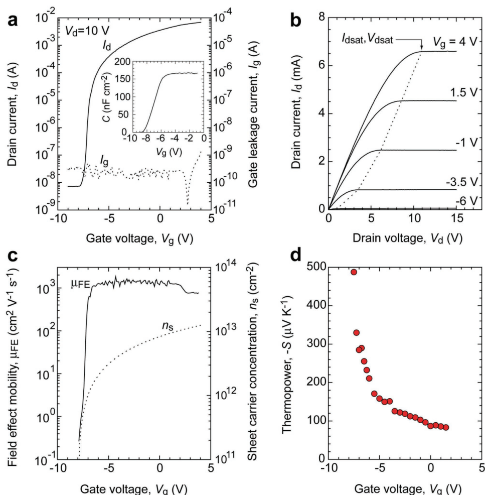
Figure 3. Carrier transport properties of 2DEG in AlGaIn/GaN MOS-HEMT at room temperature. a) Transfer I_d - V_g characteristic at V_d = 10 \text{ V} . I_g - V_g characteristic is also plotted. Inset shows the C_i - V_g characteristic. b) Output I_d - V_d characteristics ( -6 \text{ V} \leq V_g \leq +4 \text{ V} ). Pinch-off and current saturation behaviors are clearly observed. c) Changes in the field effect mobility ( \mu_{\text{FE}} ) and the sheet carrier concentration ( n_s ) as functions of V_g . d) Change in the thermopower ( S ) as a function of V_g .
