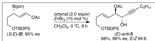
Scheme 3 Aldehyde Allylation with Optically Active \gamma -Acetoxyallylboronate ( S,E )- 2f a
