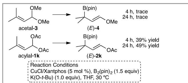
Scheme 2 \gamma -Borylation of Trisubstituted Allyl Acetal and Acylal with CuCl/Xantphos Catalyst System a
