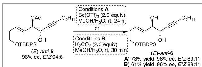
Scheme 4 Deprotection of the Acetyl Group in the Allylation Products under Acidic and Basic Conditions
