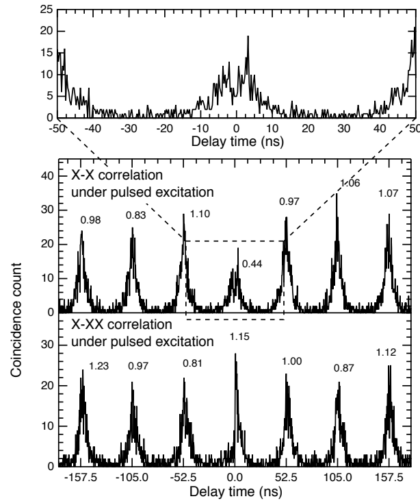
Fig. 7. Results of photon-correlation measurement of a NW-QD under pulsed excitation. (a) X-X correlation and (b) X-XX correlation. Numbers represent normalized counts in 4.8 ns time bins.
