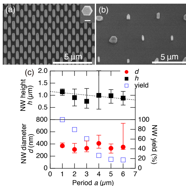
Fig. 1. (Color online) SEM images of InP NWs with (a) a=1\ \mu\text{m} and (b) a=5\ \mu\text{m} . The top-right inset in (a) is a top-view SEM image and the scale bar is 200 nm. (c) Average diameter d and height h of NWs and their formation rate. Bars indicate the maximum and minimum sizes of the NWs measured among 10 to 20 samples. The dotted line is the result of a least-mean-square linear fit for h , indicating that the diameter decreases with increasing a .
