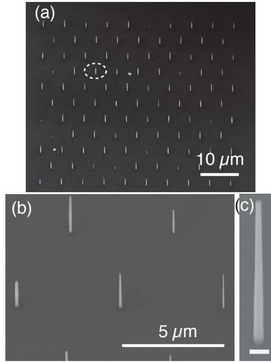
Fig. 4. SEM images of InP/InAsP/InP NW-QD array with period a=5\ \mu\text{m} . The NW enclosed by the white circle in (a) is the one whose PL results are shown in Fig. 5. The scale bar in (c) is 200 nm.
