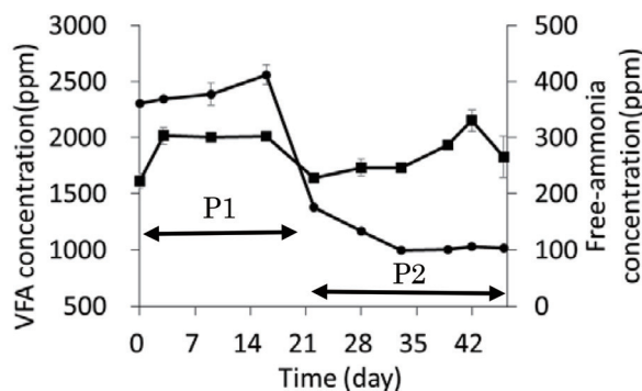
(c) VFA and free-ammonia concentration (■ : VFA concentration, ● : free-ammonia concentration)
