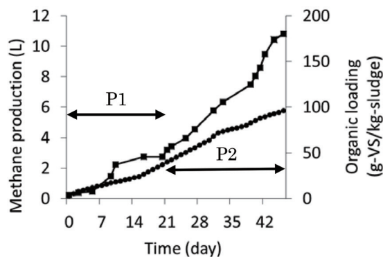
(a) Cumulative methane production and cumulative organic loading (■ : methane production, ● : organic loading)
