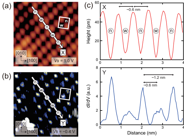
Fig. 4. (a), (b) Two-pass scan images ( 5.0 \times 5.0 \text{ nm}^2 ). First, an unoccupied-state STM image (a) was taken at a set point of +1.0 V and 0.3 nA. Second, a dI/dV image (b) was taken at a bias voltage of -0.4 V (the topography recorded in (a) was played with a z-offset of 100 pm toward the surface). The narrow and wide sections are marked as “n” and “w”, respectively. (c) Line profiles taken along the arrows marked as X and Y in (a) and (b), respectively.
