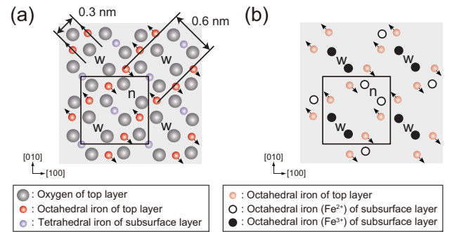
Fig. 1. Model of the B-terminated surface structure (a) and the subsurface charge-ordered structure (b) of \text{Fe}_3\text{O}_4(001) . The black arrows indicate the directions of the displacements of octahedral iron atoms of the top layer. The (\sqrt{2} \times \sqrt{2})R45^\circ reconstructed unit cell is indicated by the black square. The narrow and wide sections are marked as “n” and “w”, respectively.
