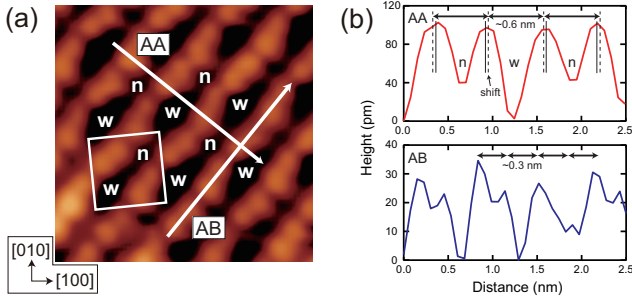
Fig. 2. (a) STM image ( 3.5 \times 3.5 \text{ nm}^2 ) of the \text{Fe}_3\text{O}_4(001) film surface. The STM image was taken with a W-tip at a set point of +1.0 V and 0.3 nA. The (\sqrt{2} \times \sqrt{2})R45^\circ reconstructed unit cell is indicated by the white square. The narrow and wide sections are marked as “n” and “w”, respectively. (b) Line profiles corresponding to the lines AA and AB in (a).
