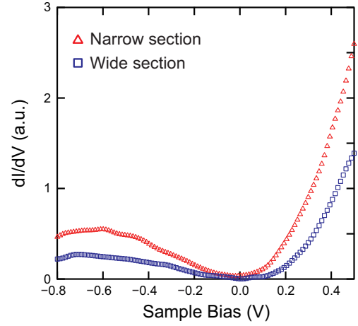
Fig. 3. dI/dV spectra obtained at the narrow and wide sections of the (\sqrt{2} \times \sqrt{2})R45^\circ surface reconstruction perpendicular to the \text{Fe}_B rows. These spectra were obtained with a z-offset of 300 pm toward the surface with respect to the original set point of +1.2 V and 0.3 nA.
