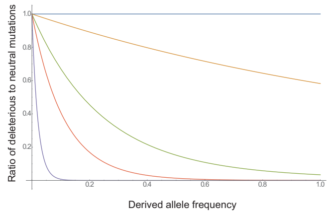
Fig. 3. Predicted frequency spectrum of deleterious mutations relative to neutral mutations. Blue, orange, green, red and purple lines represent scaled selection coefficient ( S ) values of 0 (neutral), -1 , -5 , -10 and -50 , respectively.
