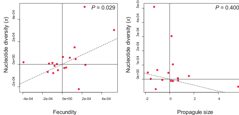
Fig. 2. Correlation between nucleotide diversity ( \pi ) and life history traits. To eliminate phylogenetic dependence, standardized contrasts or phylogenetically independent contrasts (PIC; Felsenstein, 1985) were employed. PIC analysis was performed using the APE package in R (Paradis et al., 2004). Branch length and life history traits were retrieved from Perelman et al. (2011) and Tacutu et al. (2013), respectively. A) Correlation between \pi and fecundity (inverse of the averaged inter-litter interval in females), B) correlation between \pi and propagule size (average volume of infants at the time of weaning).
