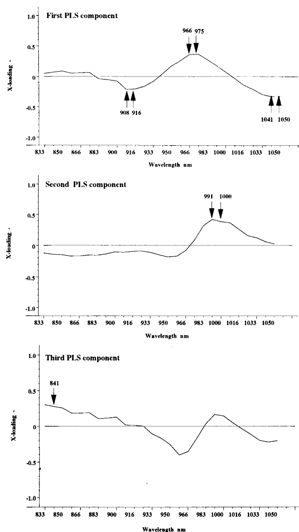
Fig. 5. PLS loading spectra for narrow AAC range in milled rices ( japonica type rices). AAC range: 13.1–20.7 (%).
