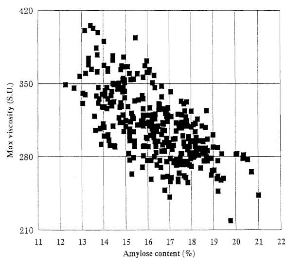
Fig. 11. Relationship between milled rice AAC and maximum viscosity.
