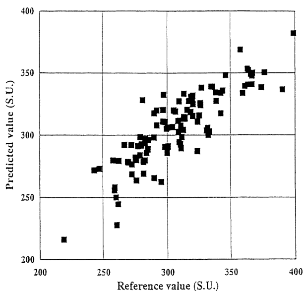
Fig. 8. Relationship between reference values of japonica type rice and predicted maximum viscosity for those rice.
