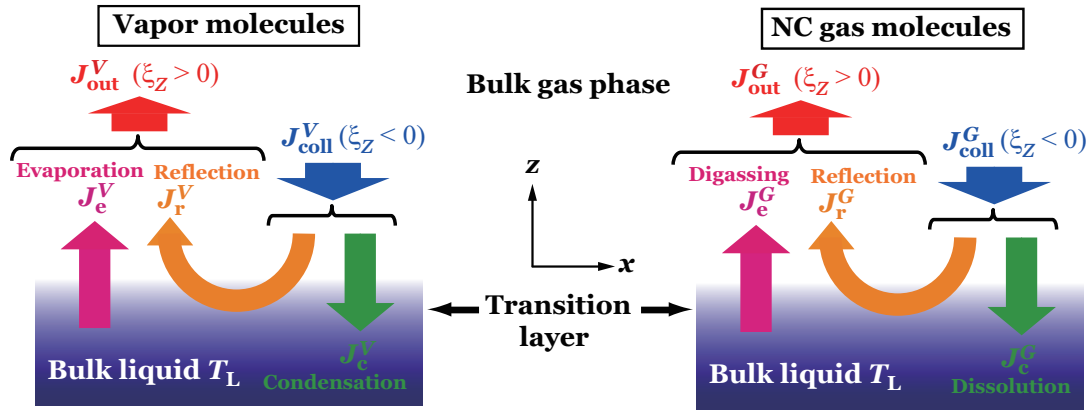
Fig. 1 Molecular mass flux relation at gas–liquid interface. Left: mass fluxes for vapor molecules, and right: mass fluxes for NC gas molecules, respectively.
