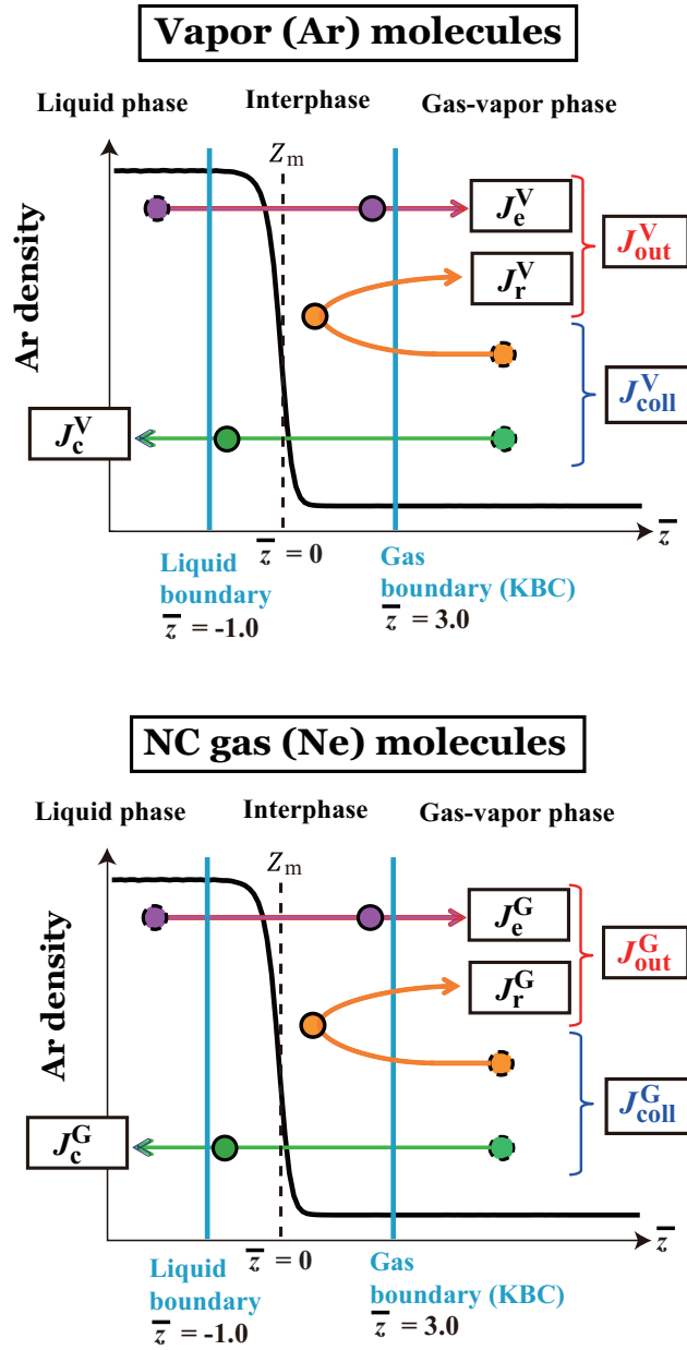
Fig. 3 Molecular mass fluxes at a gas–liquid interface. There are gas and liquid boundaries in the vicinity of the density transition layer of Ar molecules. \bar{z} is the normalized z axis.
