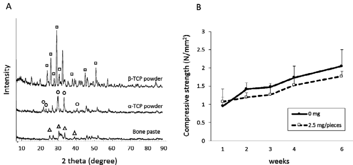
Figure 2 (A) X-ray diffraction patterns of \beta -tricalcium phosphate ( \beta -TCP) powder, \alpha -tricalcium phosphate ( \alpha -TCP) powder and bone paste emulsion. \square : \beta -TCP, \circ : \alpha -TCP and \Delta : hydroxyapatite. (B) Compressive strength of pure bone paste and simvastatin-containing bone paste (2.5 mg/pieces).
