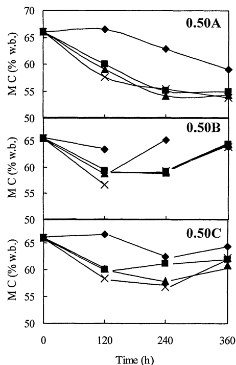
Fig. 6 Moisture content changes of layers for aeration of 0.50 L/min.kgdm (runs 0.50A, 0.50B, and 0.50C)
