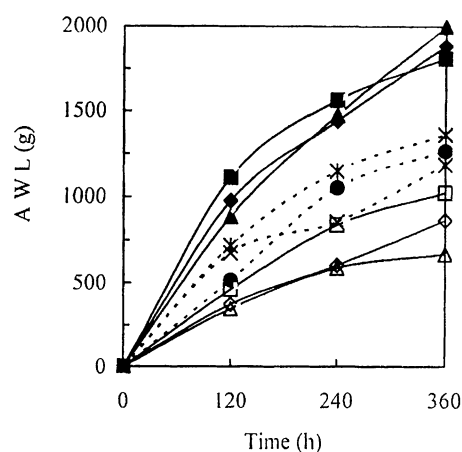
Fig. 8 Accumulated weight loss (AWL) during 360 h of composting with different aeration rates and turning patterns (—◇— : 0.05A; —□— : 0.05B; —△— : 0.05C; —×— : 0.15A; —*— : 0.15B; —-·- : 0.15C; —◆— : 0.50A; —■— : 0.50B; —▲— : 0.50C)
