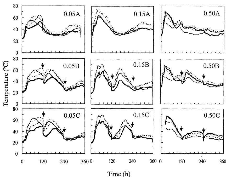
Fig. 4 Effect of aeration rates and turning patterns on the temperature distribution of compost materials (— : L1; ····· : L2; - - - : L3; — : L4; — : ambient temperature; → : turning)
