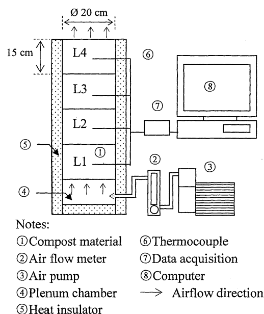
Fig. 1 Compost reactor setup
