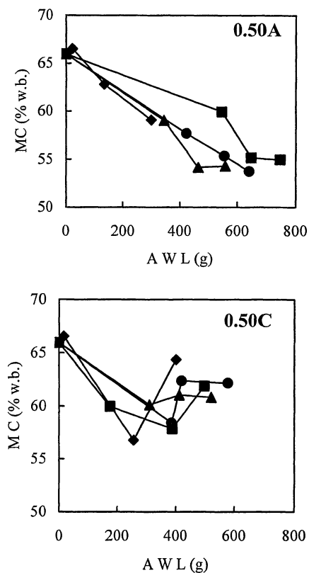
Fig. 9 Relationship between accumulated weight loss (AWL) and moisture content change (—●— : L1; —▲— : L2; —■— : L3; —◆— : L4)
