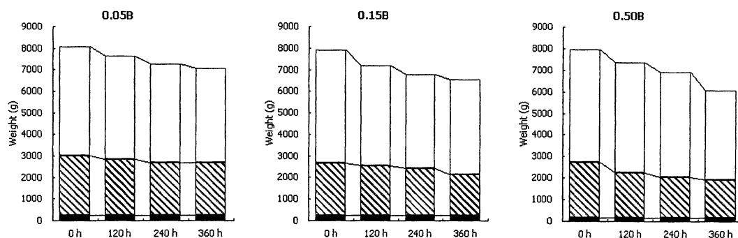
Fig. 10 Composition of water, organic matter, and ash in compost material during 360 h of composting (□ : water; ▨ : organic matter; ■ : ash)
