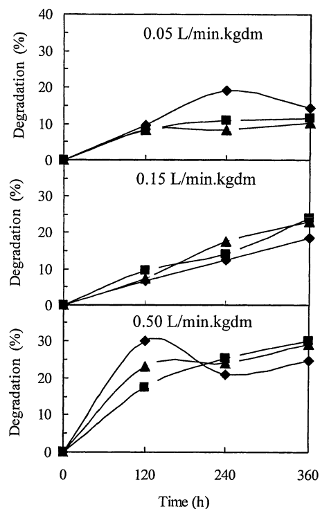
Fig. 7 Degradation of organic matter during 360 h of composting with different aeration rates and turning patterns (—◆— : A; —■— : B; —▲— : C)
