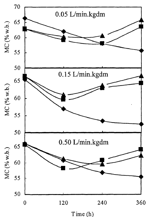
Fig. 5 Moisture content changes during 360 h of composting with different aeration rates and turning patterns (—◆— : A; —■— : B; —▲— : C)
