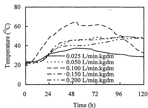
Fig. 3 Effect of aeration rates on average temperature of compost material during 120 h of composting
