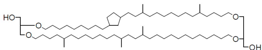
GDGT IIIb (1048)
