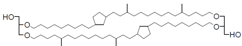
GDGT IIIc (1046)
