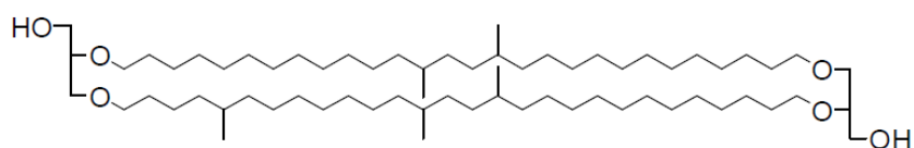
GDGT II (1036)
