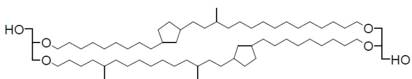
GDGT IIc (1032)
