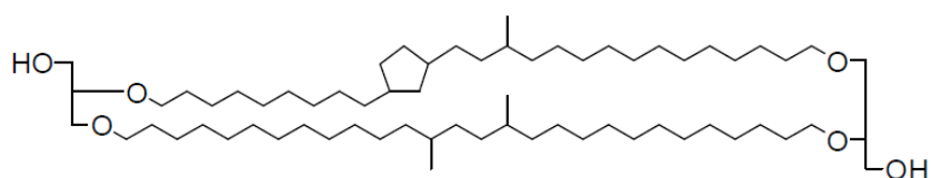
GDGT Ib (1020)
