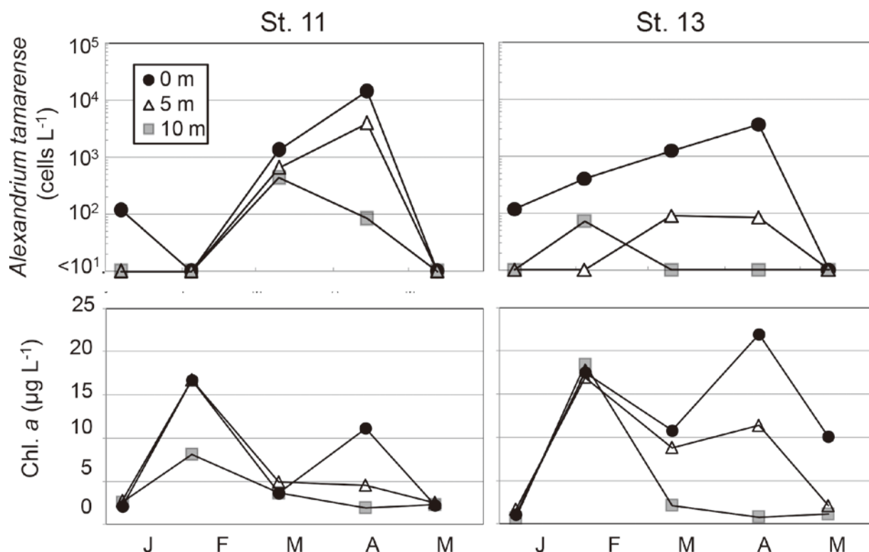
Fig. 3. Seasonal changes in the cell densities of the toxic dinoflagellate Alexandrium tamarens (cells L -1 ) and chlorophyll a (Chl. a ; µg L -1 ) at Sts. 11 and 13 in the eastern part of Osaka Bay from January to May 2008. N.D.= not detected.
