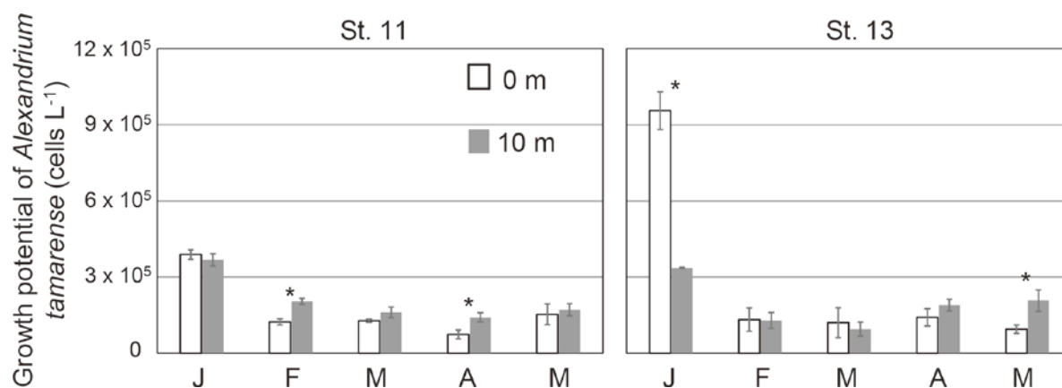
Fig. 4. Results of the bioassay with Alexandrium tamarens to determine the growth potentials of seawater samples collected at 0 and 10 m in depth at Sts. 11 and 13 in the eastern part of Osaka Bay from January 2008 to May 2008. An asterisk (*) indicates a significant difference between growth potentials at 0 and 10 m ( P < 0.05 ). Error bars indicate standard deviation.
