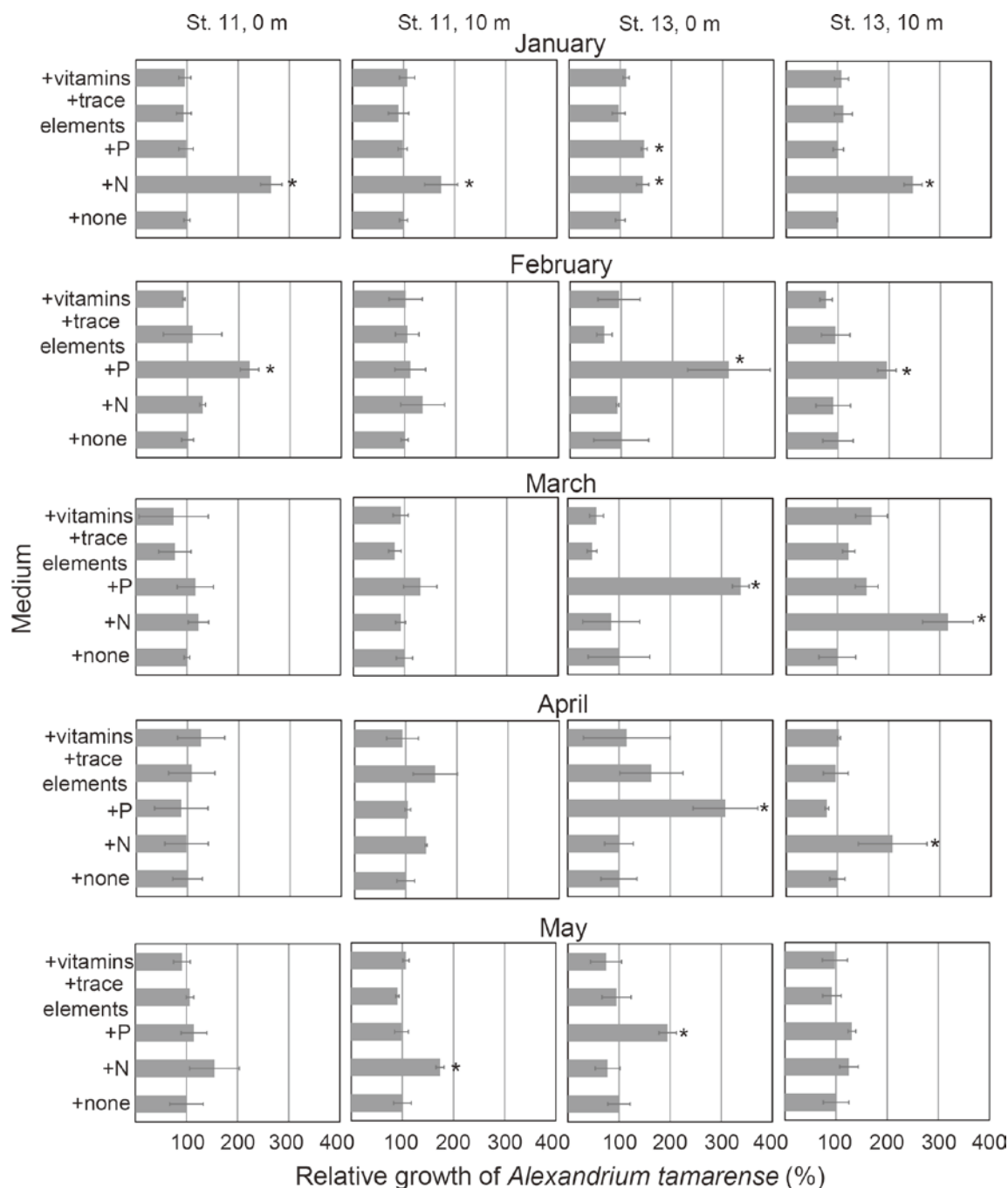
Fig. 5. Results of the bioassay with Alexandrium tamarens to determine the growth-limiting nutrients of seawater samples collected from 0 and 10 m in depth at Sts. 11 and 13 in the eastern part of Osaka Bay from January 2008 to May 2008. An asterisk (*) next to a nutrient-added medium indicates a significant increase of the treatment mean over that of the +none treatment. Treatment means were analyzed using Dunnett's multiple comparison test ( P < 0.05 ). Error bars indicate standard deviation. Data represent the means of n = 3 replicates.
