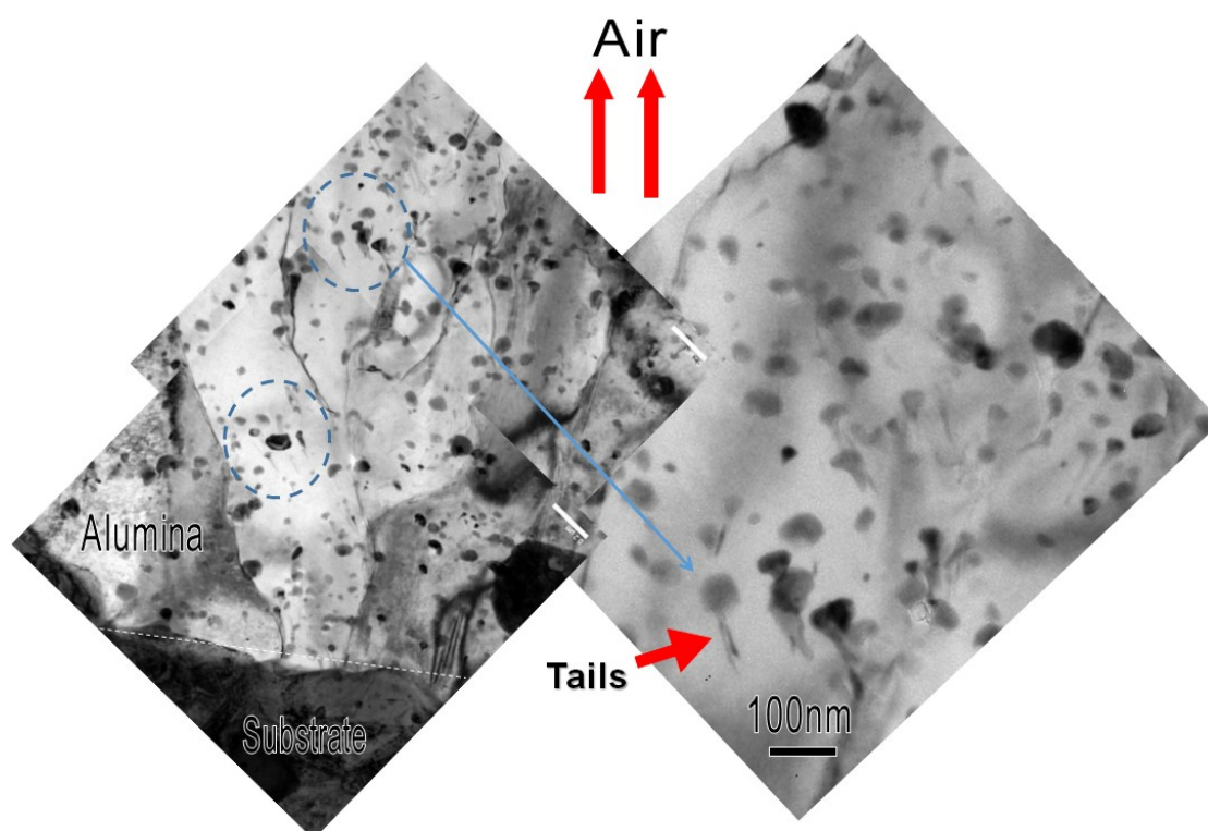
Fig. 5.13 TEM images of 10AlCrY sample oxidized at 900 °C in 225 h. A special structure of dispersoids with spherical head region and long tail could be observed.
