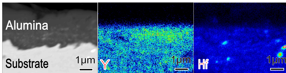
Fig. 5.34 EPMA elemental mappings of Y and Hf in alumina scales of the 10AlCrY samples oxidized at 900 °C for 100 h.
