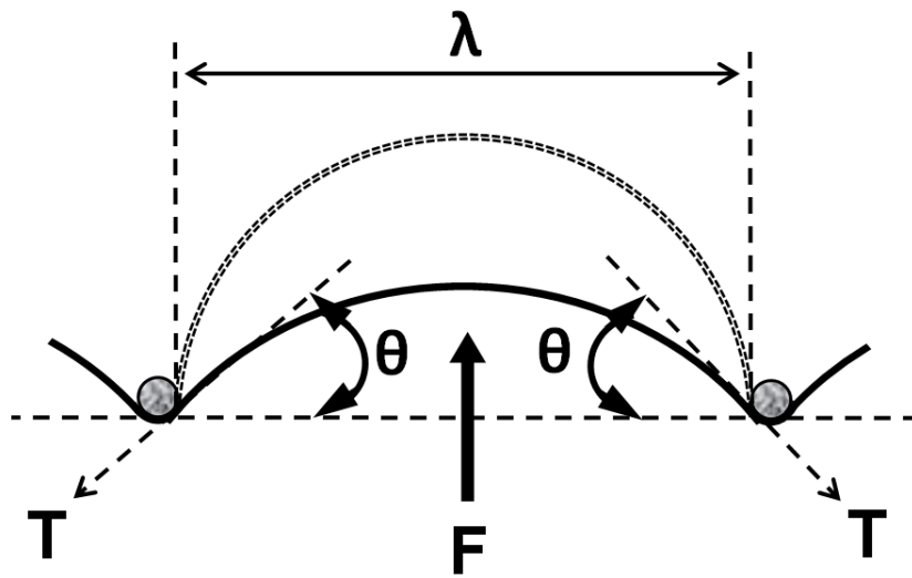
Fig. 2.3 Equilibrium model between the dislocation and particles
