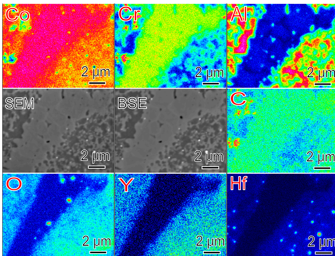
Fig. 4.15 SEM / BSE micrographs and corresponding EPMA elemental maps obtained from 10AlCrY sample consolidated with Hot Press.
