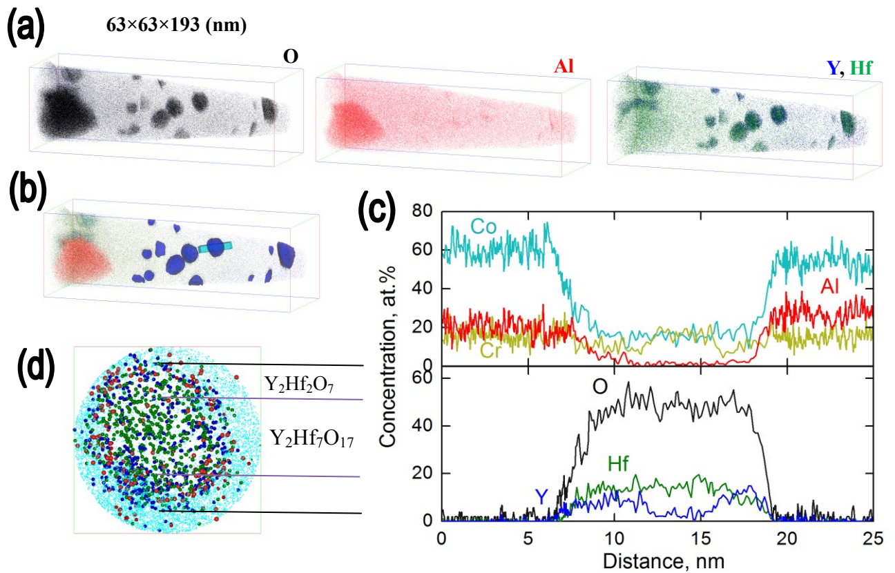
Fig. 4.10 The 3DAP atoms map (a) (b) obtained in B2 phase in 10 AlCrY, (c) is 1D compositional profile along light blue cuboid shown in (b), (d) exhibits core-shell structure consisted of Y_2Hf_7O_{17} in the center and Y_2Hf_2O_7 at the periphery.
