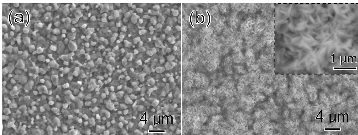
Fig. 5.20 Surface morphologies of oxide scales oxidized in 25 h at 900 °C, (a) for 10AlY sample and (b) for 10AlCrY.
