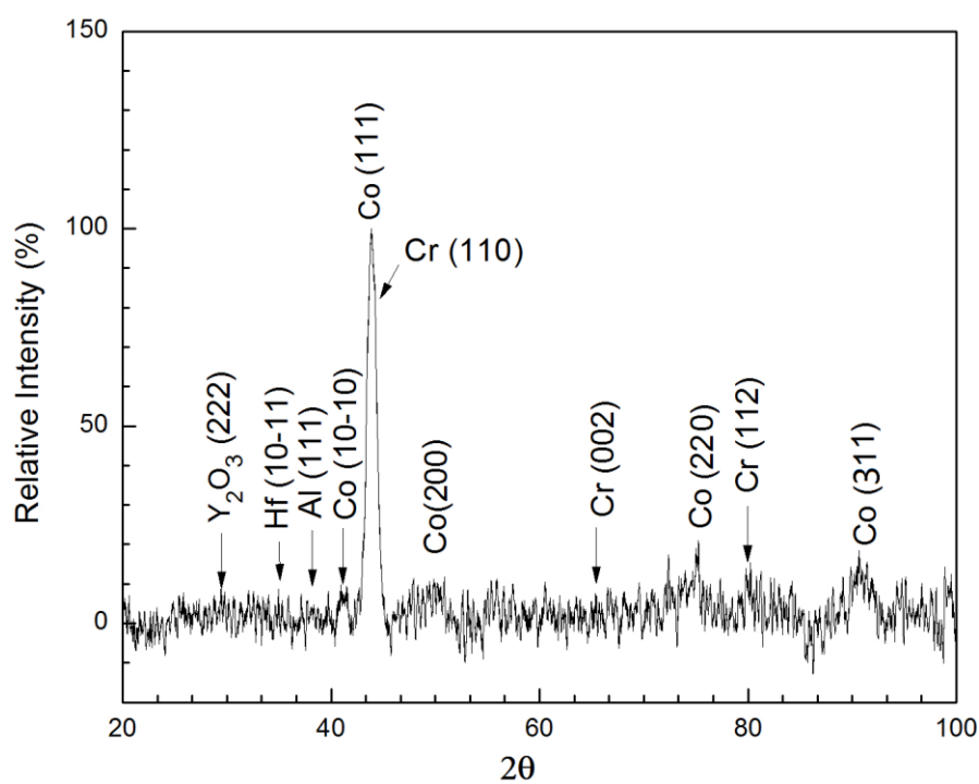
Fig. 4.2 XRD pattern of 5AlCrY powder milled for 48 h.
