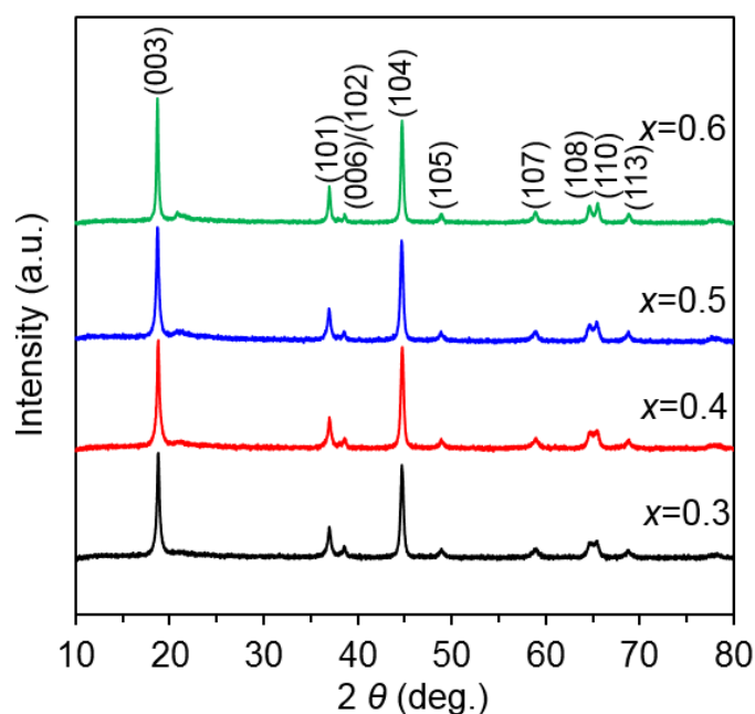
Fig. 5-1 XRD patterns of x\text{Li}_2\text{MnO}_3-(1-x)\text{LiNi}_{1/3}\text{Co}_{1/3}\text{Mn}_{1/3}\text{O}_2 ( x=0.3, 0.4, 0.5, 0.6 ) samples.
