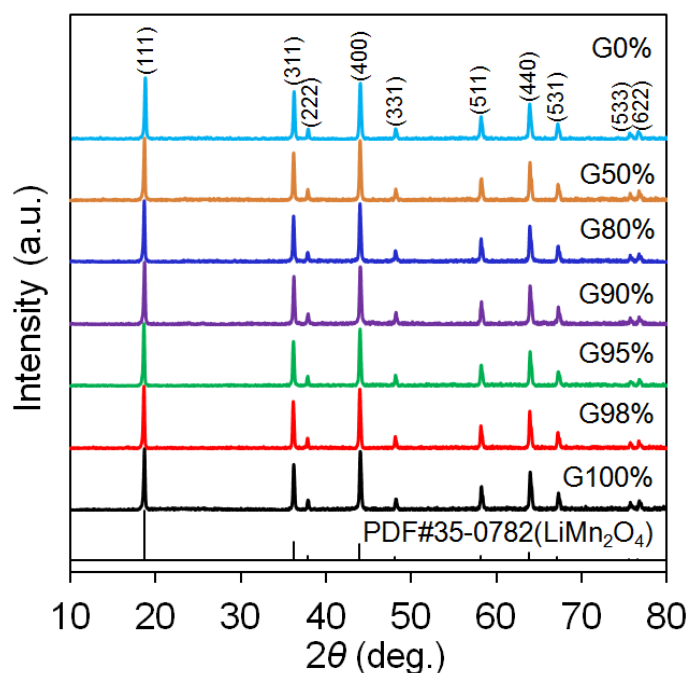
Fig. 2-5 XRD patterns of powders with different glycine/sucrose ratios calcined in air at 800 °C for 24 h. All the diffraction peaks match well with those of the LiMn 2 O 4 phase.
