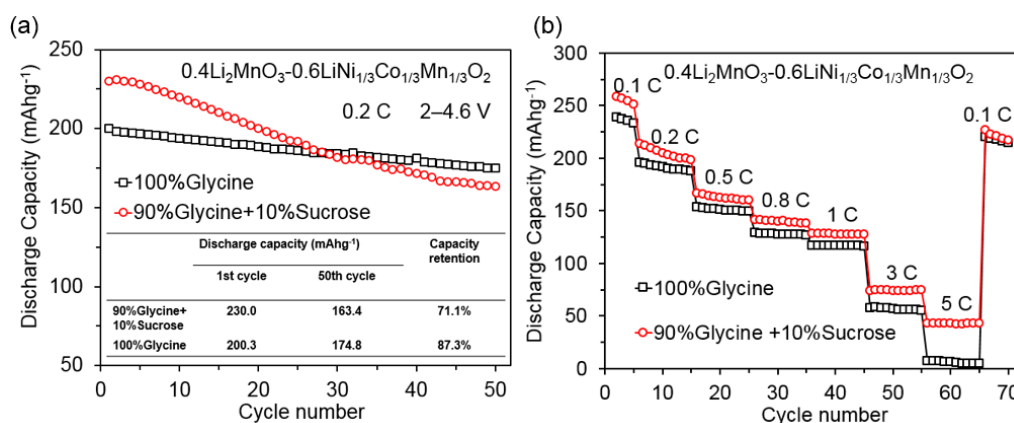
Fig. 5-8 (a) discharge capacity vs. cycle number, (b) rate capability of 0.4\text{Li}_2\text{MnO}_3\text{-}0.6\text{LiNi}_{1/3}\text{Co}_{1/3}\text{Mn}_{1/3}\text{O}_2 sample by using 100%Glycine, and 90%Glycine+10%Sucrose as fuels.
