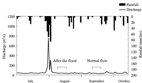
Fig. 2. Temporal changes in water discharge and daily rainfall in Yurappu River from July to October, 1999. □ indicates sampling period.
