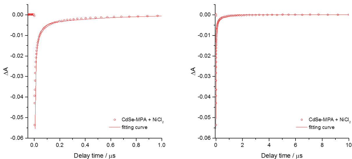
Figure 3-12. Analysis of kinetic trace of transient bleach about the mixture of CdSe-MPA and \text{NiCl}_2 in (left) short temporal window and (right) long temporal window. Circle: measured data, line: the result of analysis.
