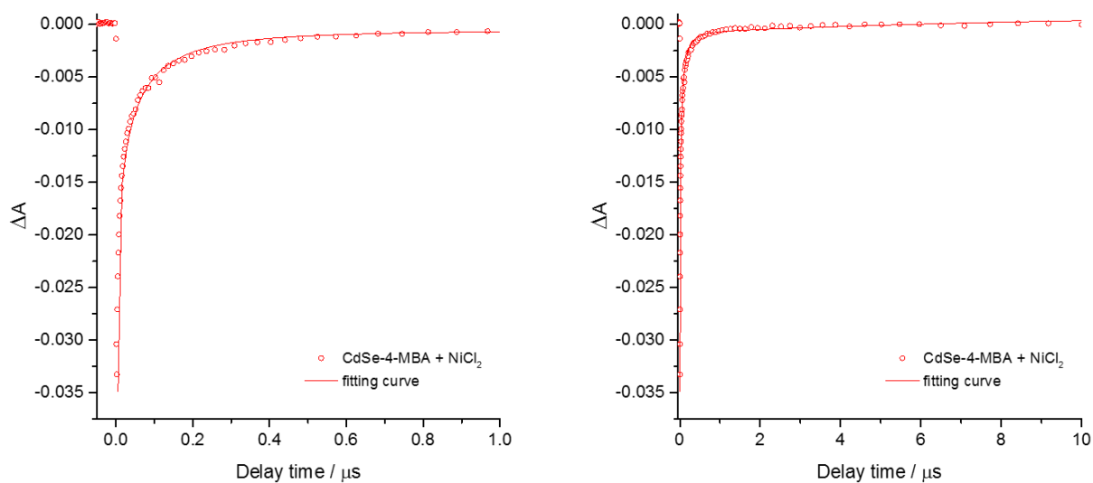
Figure 3-14. Analysis of kinetic trace of transient bleach about the mixture of CdSe-4-MBA and \text{NiCl}_2 in (left) short temporal window and (right) long temporal window. Circle: measured data, line: the result of analysis.
