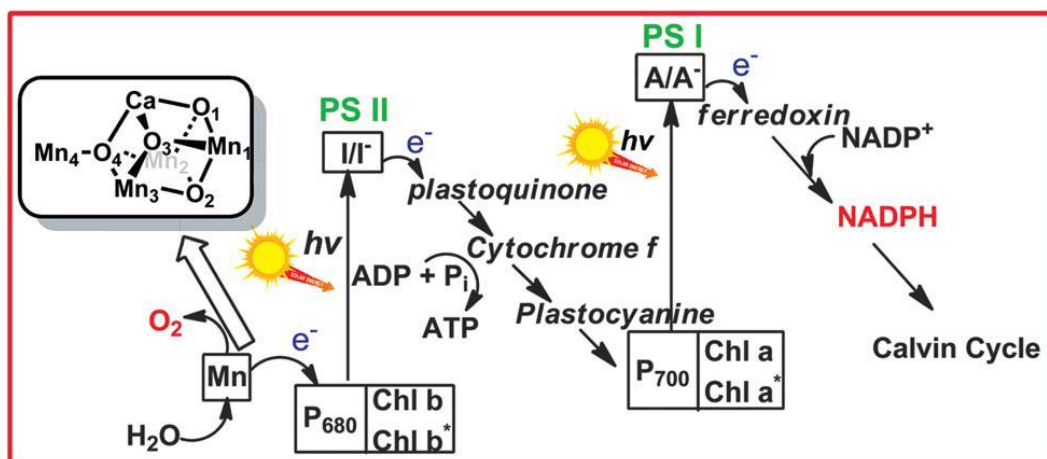
Figure 1-1. Two-step photoinduced-electron transfer reaction in natural photosynthesis (so called “Z scheme”). 4
