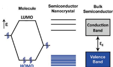
Figure 1-4. Electronic orbital of molecule, band structure of semiconductor nanocrystal and bulk semiconductor. 17
