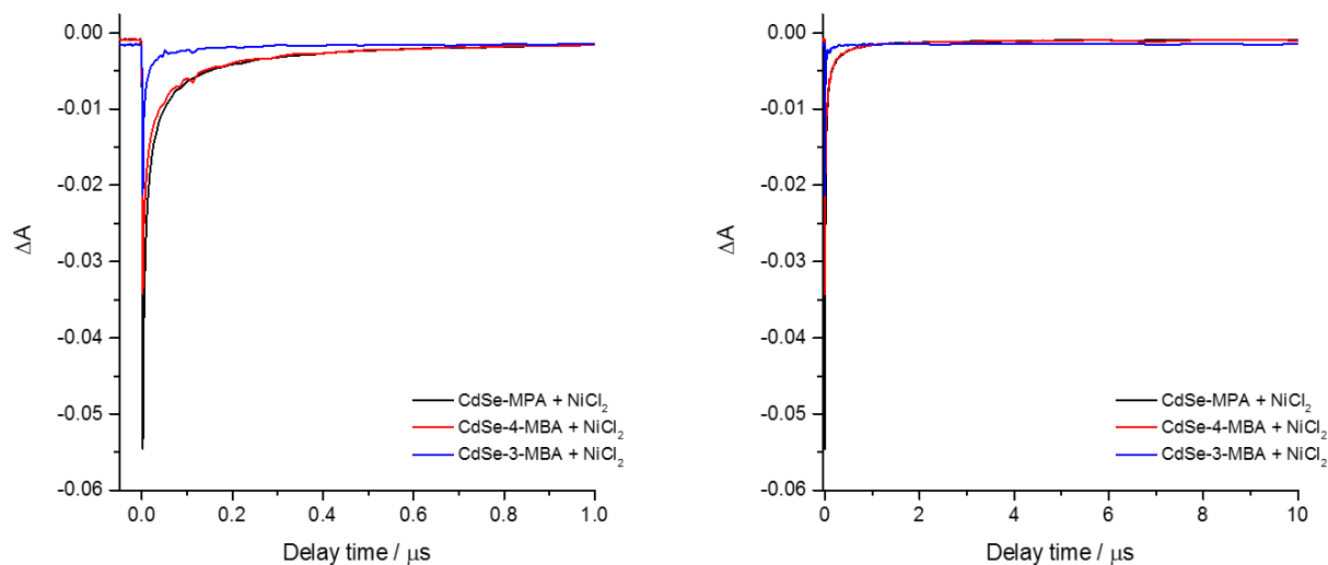
Figure 3-10. Kinetic trace of transient bleach about CdSe-MPA and \text{NiCl}_2 (black), CdSe-4-MBA and \text{NiCl}_2 (red), CdSe-3-MBA and \text{NiCl}_2 (blue) in (left) short temporal window and (right) long temporal window.
