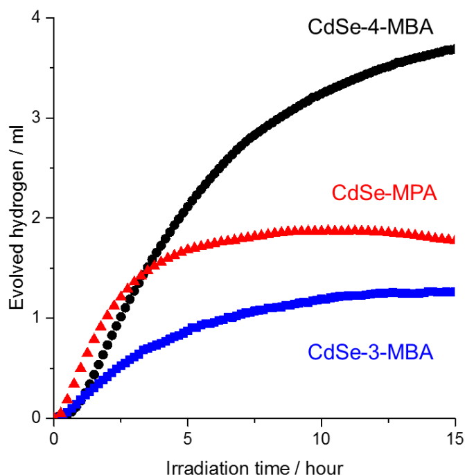
Figure 3-8. Photocatalytic hydrogen evolution reactions (HERs) from aqueous solution (pH 4) comprising 4 \mu M CdSe-4-MBA (black circles), CdSe-MPA (red triangles), CdSe-3-MBA (blue squares) as the photosensitizer, ascorbic acid (0.5M) as the sacrificial electron donor, and \text{NiCl}_2 (4 \mu M) as precursor of hydrogen evolution catalyst; light irradiation at 525 nm.
