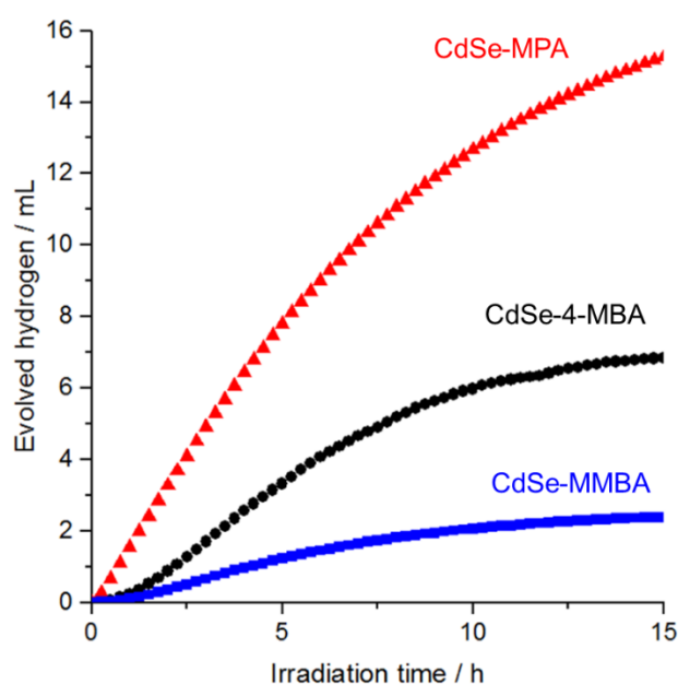
Figure 2-8. Photocatalytic hydrogen evolution reactions (HERs) from aqueous solutions (pH 6) comprising 4 \mu\text{M} CdSe-4-MBA (black circles), CdSe-MPA (red triangles) or CdSe-MMBA (blue squares) as the photosensitizer, ascorbic acid (0.5 M) as the sacrificial electron donor, and Pt-PVP (12 nM) as the hydrogen evolution catalyst; light irradiation at 525 nm.
