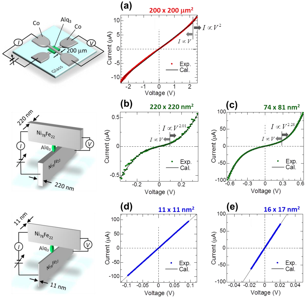
Figure 4.7 I - V characteristics of metal/Alq 3 /metal junctions. (a) Co/Alq 3 /Co junction with area of 200×200 μm 2 . Py/Alq 3 /Py nanoscale junctions with junction area of (b) 220×220 nm 2 , (c) 74×81 nm 2 , (d) 11×11 nm 2 and (e) 16×17 nm 2 .
