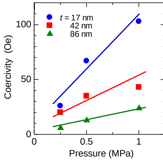
Figure 3.11 Pressure dependence of coercivity of Py thin films with thicknesses of 17, 42, and 86 nm sandwiched between LSP glasses after thermal pressing process.
