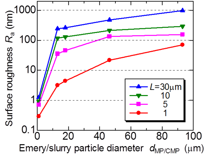
Figure 2.8 Surface roughness of polished LSP-glass/Co/LSP-glass observed using the AFM as function of diameter d_{MP/CMP} of Al_2O_3 -based emeries ( d_{MP} > 10 \mu m ) or CeO_2 slurries ( d_{CMP} = 1 \mu m ).
