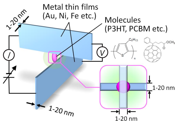
Figure 1.7 Schematic of metal/molecule/metal nanoscale junction containing metal thin-film edges. Nanoscale junction consists of molecules sandwiched between crossed edges of two metal thin films. Junction area is determined by film thickness; thus, 1–20-nm thick films could produce 1 \times 1 - 20 \times 20\text{-nm}^2 nanoscale junctions.
