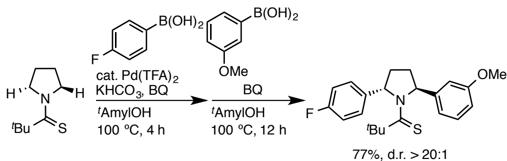
Scheme 9. Pd-catalyzed Stereoselective C(sp 3 )-H Arylation: Yu group
