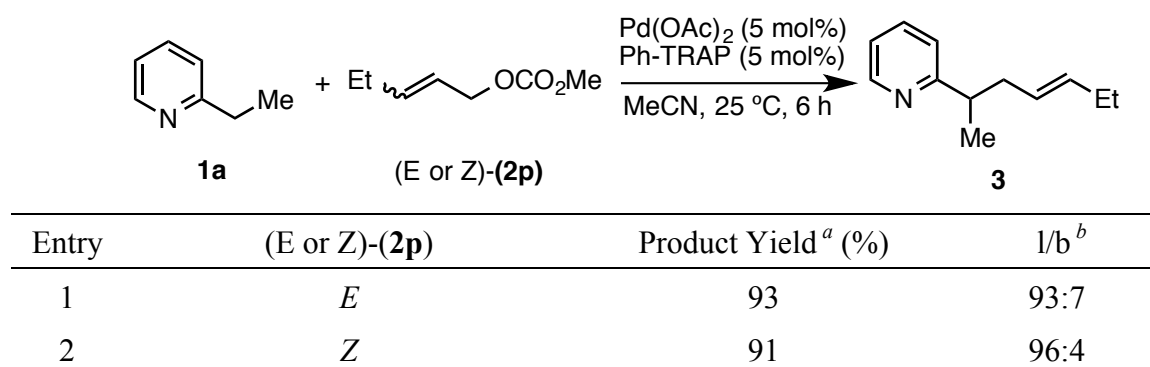
Figure 2. Effect of alkene geometries of allylic carbonates.
