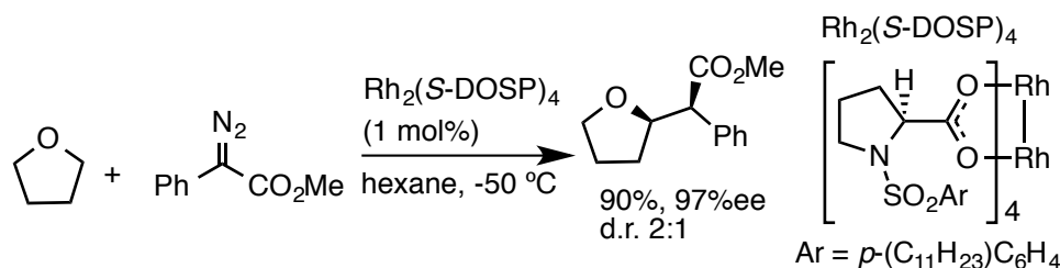
Scheme 18. Rhodium-catalyzed Enantioselective Insertion Reaction with Relatively Activated C(sp 3 )-H Bonds
