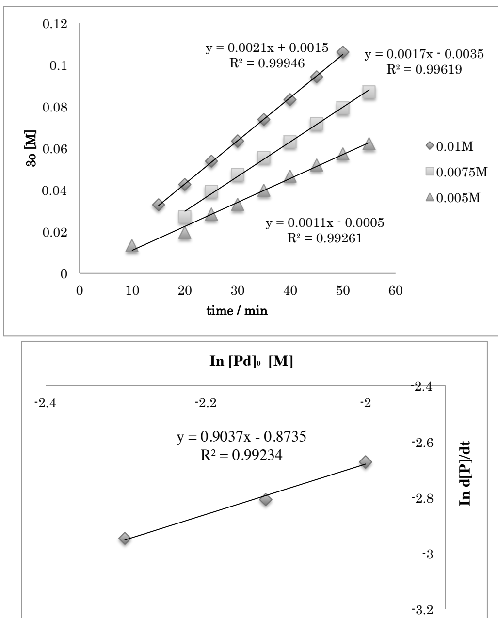
Figure 4. (a) Initial rate kinetic experiments for Pd (b) Plot of \ln(d[3s]/dt) versus \ln [Pd] .
