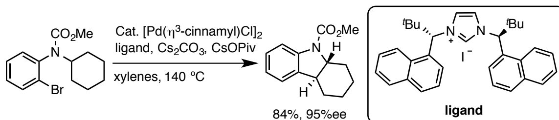
Scheme 11. Enantioselective C(sp 3 )-H Functionalization: Intramolecular Reaction
