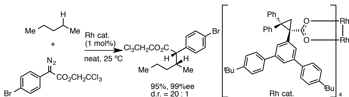
Scheme 19. Rhodium-catalyzed Enantioselective Unactivated C(sp 3 )-H Insertion Reaction
