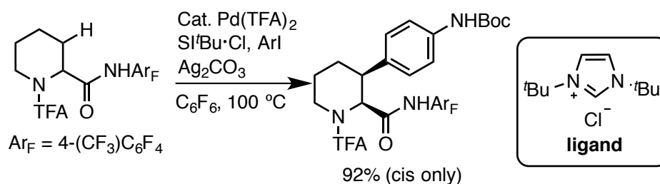
Scheme 10. Ligand-enabled Stereoselective C(sp 3 )-H Arylation: Yu group
