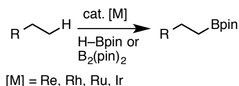
Scheme 30. Selective Borylation of Primary C(sp 3 )-H Bonds
