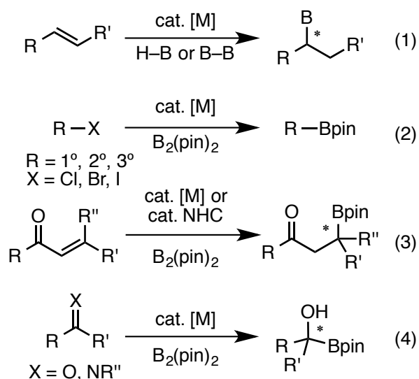
Scheme 29. Synthesis of Alkylboronates: Transition Metal Catalysts
