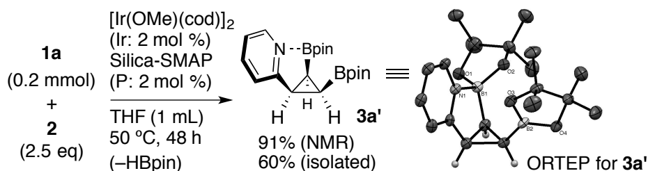
Scheme 2. Silica-SMAP-Ir catalyzed bisborylation of 1a .
