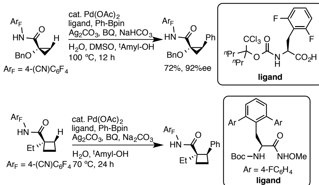
Scheme 14. Pd-catalyzed Enantioselective C(sp 3 )-H Functionalization of Small-ring Carbocycles
