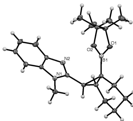
Figure 2. Molecular structure of the tertiary alkylboronate 3j .
