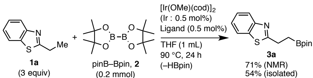
Scheme 1. Gram-scale borylation of 1a .
