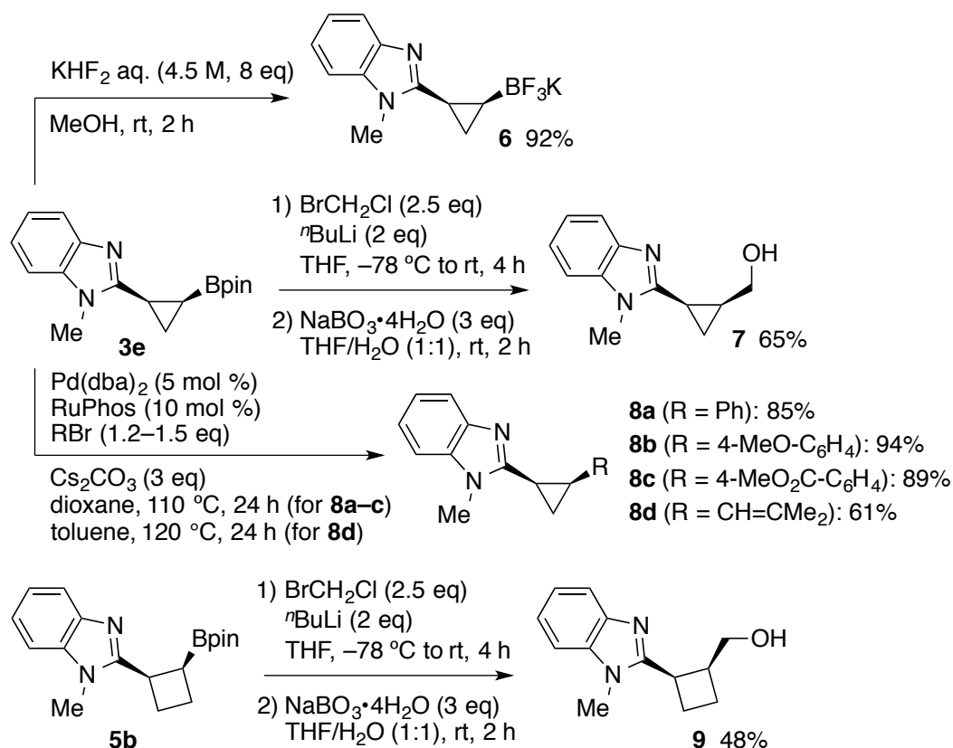
Scheme 5. Transformations of borylation products.
