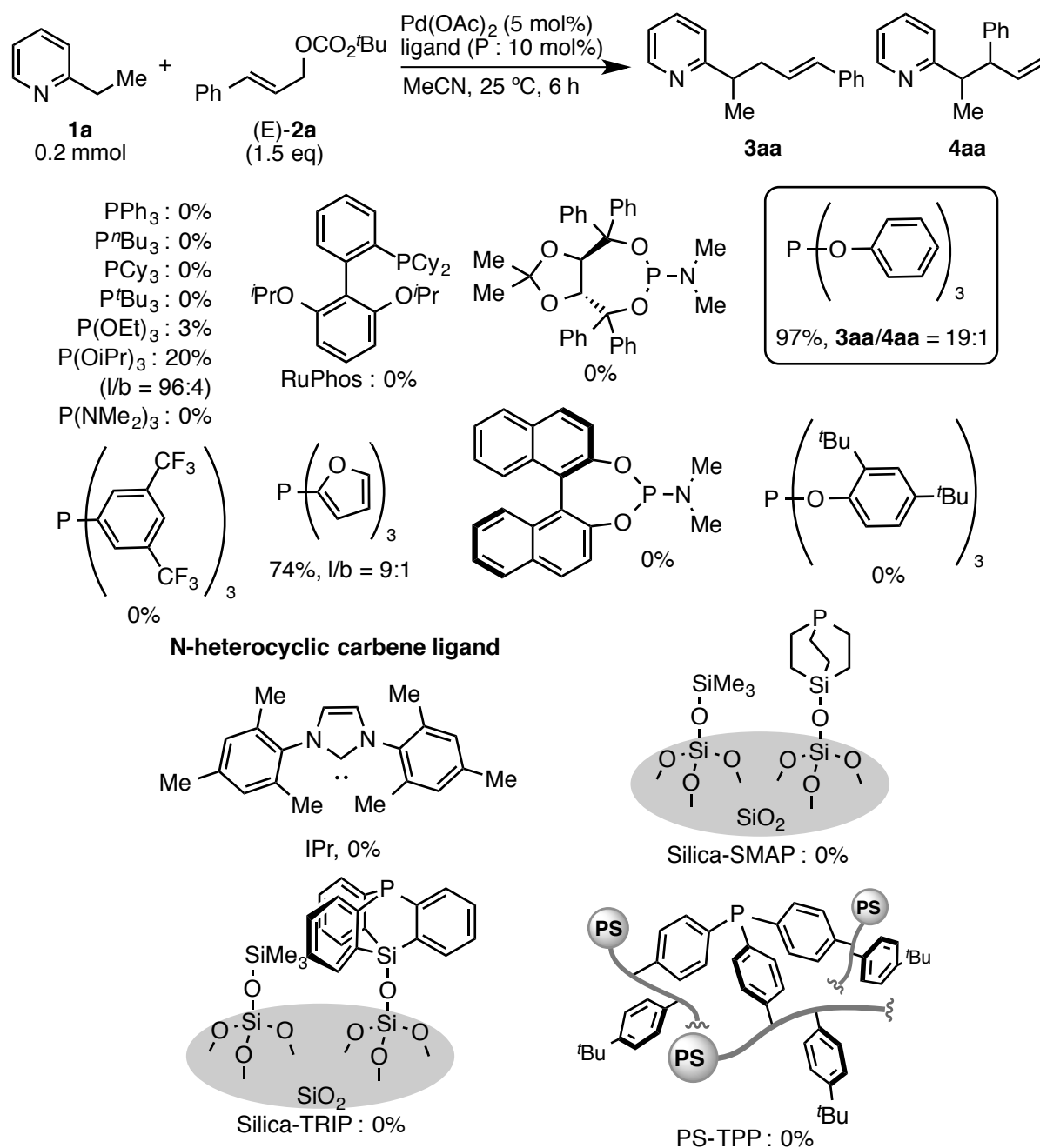
Figure 1. Screening of monodentate ligands. Reaction conditions:
