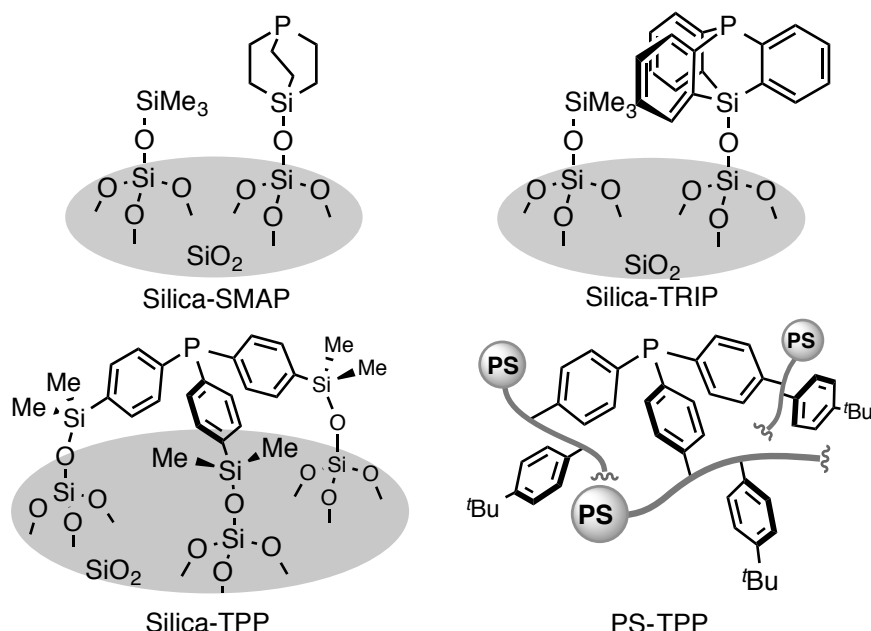
Figure 2. Solid-Supported Monophosphine.
