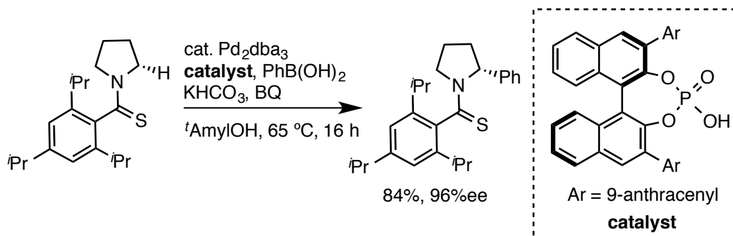
Scheme 15. Pd-catalyzed Enantioselective Amine \alpha\text{-C(sp}^3\text{)-H} Arylation
