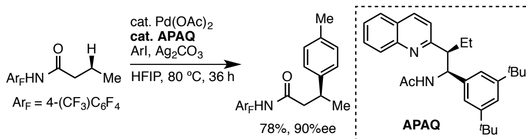
Scheme 16. Pd-catalyzed Enantioselective Unactivated C(sp 3 )-H Arylation
