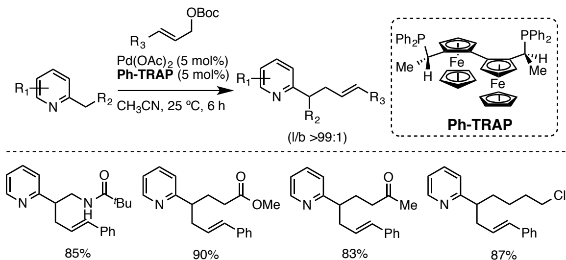
Scheme 40. Ph-TRAP-Pd-catalytic System: Substrate Scope
