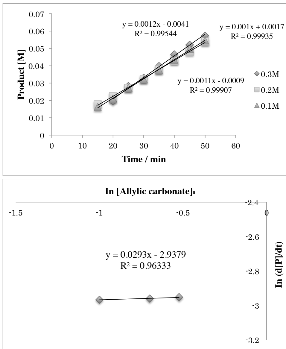
Figure 3. (a) Initial rate kinetic experiments for 1k (b) Plot of \ln(d[3s]/dt) versus \ln [1k] .
